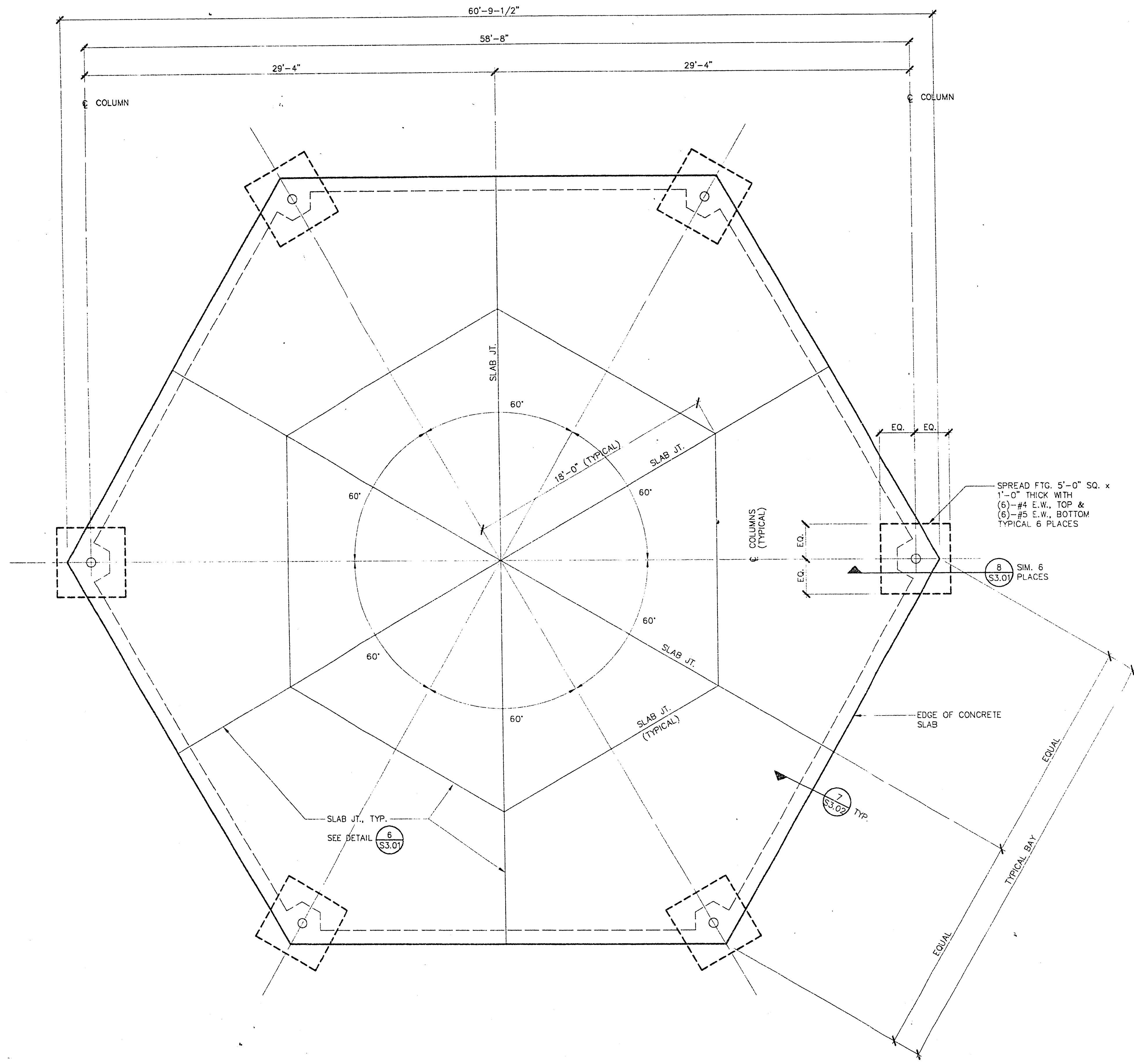
FOUNDATION PLAN - 60' CANOPY BLDG. (ALTERNATE #2) EAST PARK ONLY 1/4" = 1'-0"
