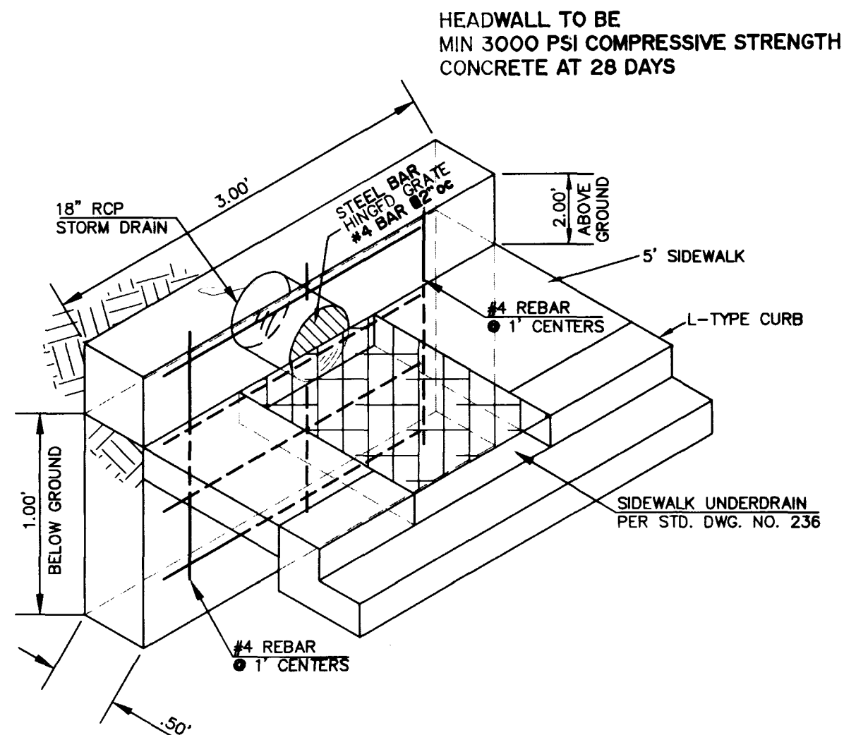
HEADWALL AND OUTLET DETAIL N.T.S.
