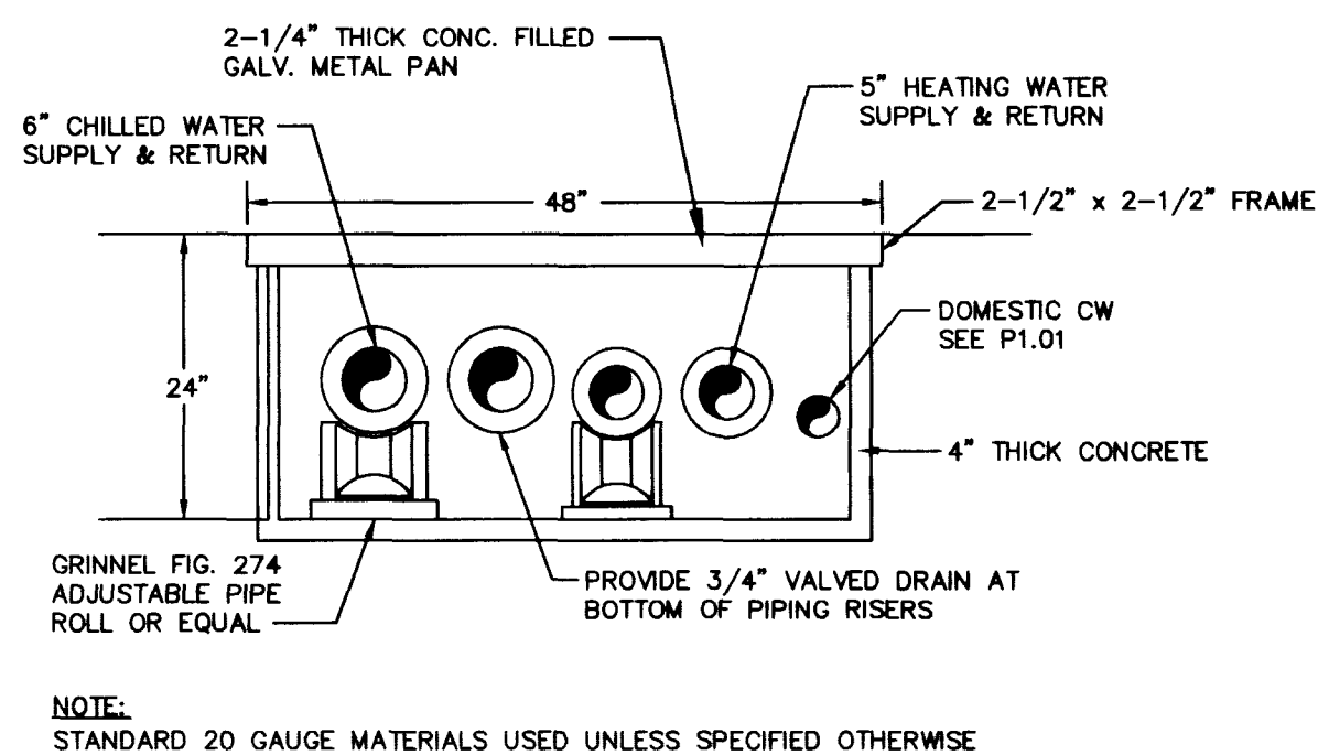
PIPING IN UTILITY TRENCH DETAIL
