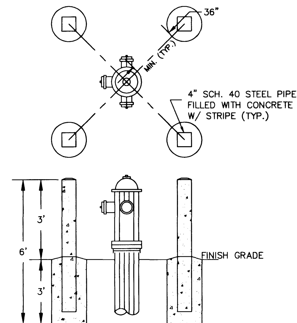
BOLLARD DETAIL
