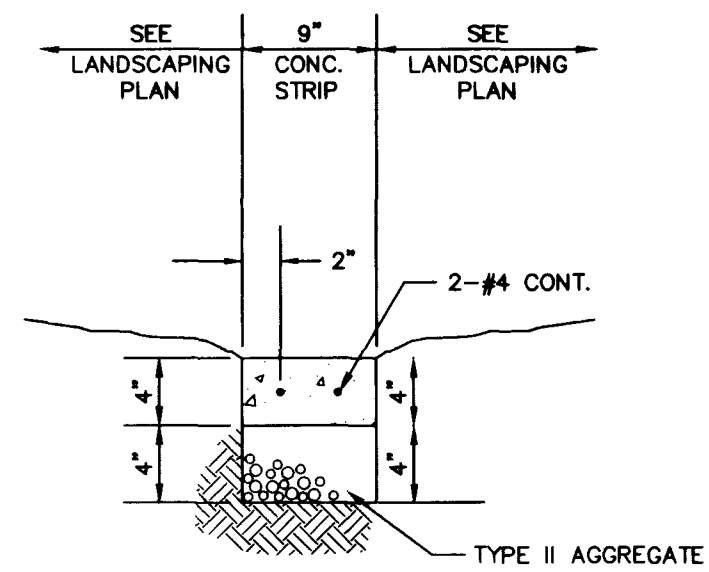
CONCRETE STRIP SECTION
