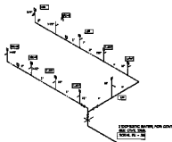
COLD WATER ISOMETRIC PIPING DIAGRAM
