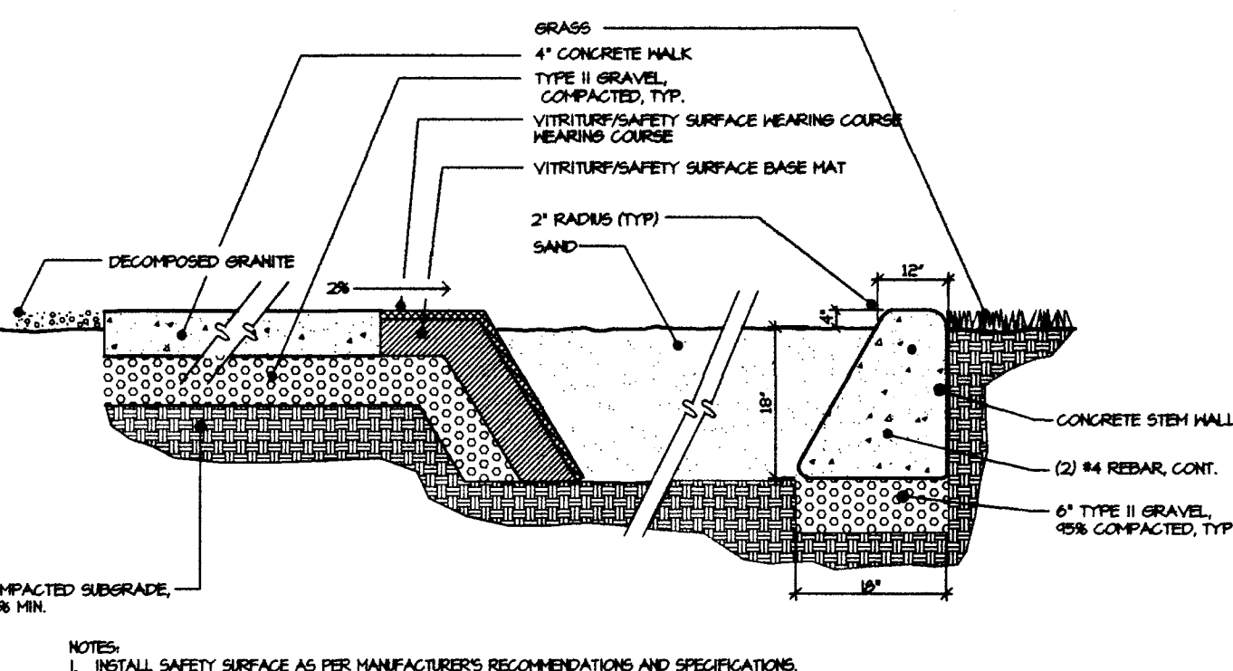
Q PLAYGROUND SECTION
