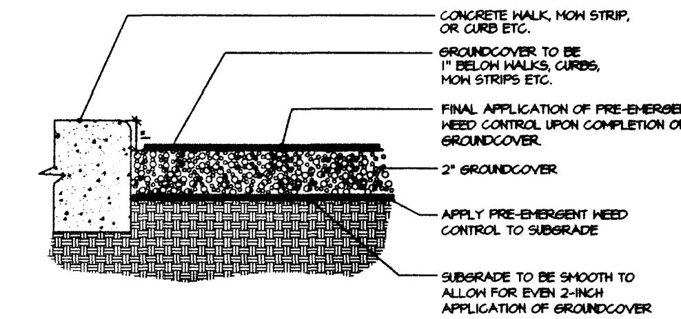
C GROUNDCOVER DETAIL
