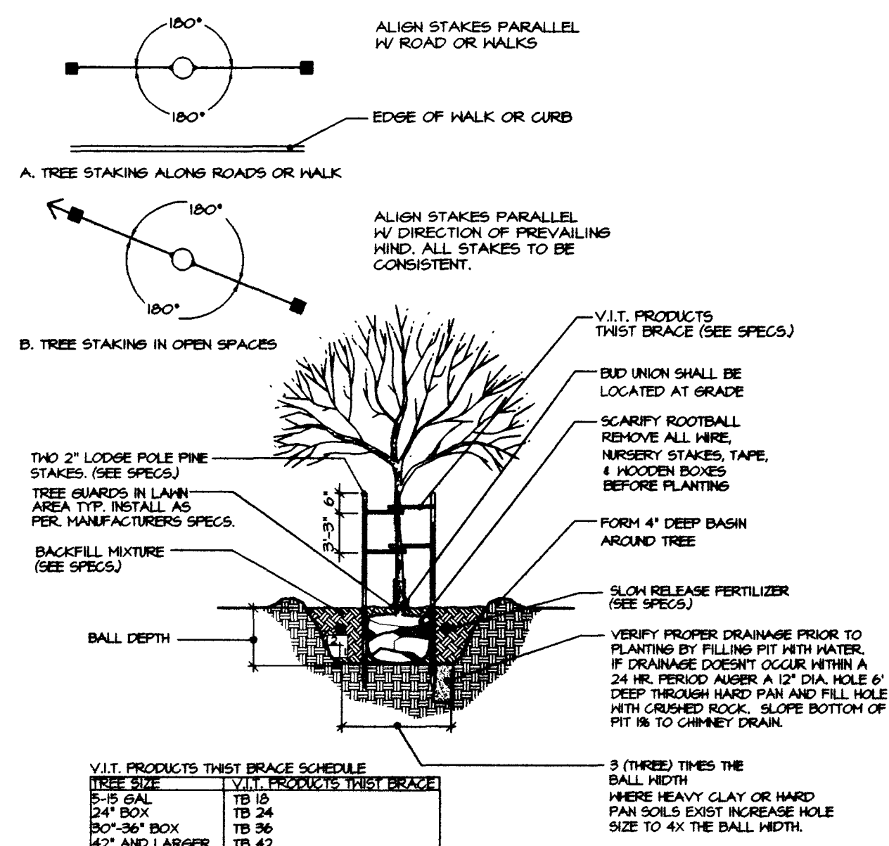
A TREE PLANTING & STAKING W/ TRUNK GUARD
