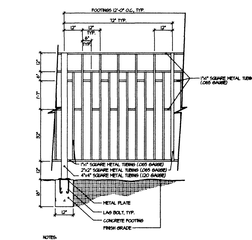
D DECORATIVE FENCING
