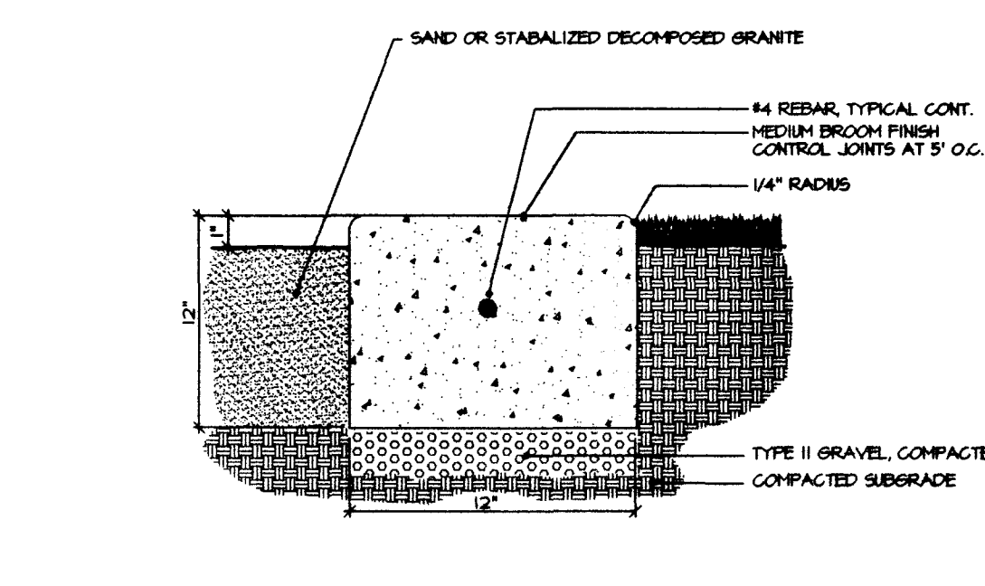
E 12" CONCRETE MOW STRIP
