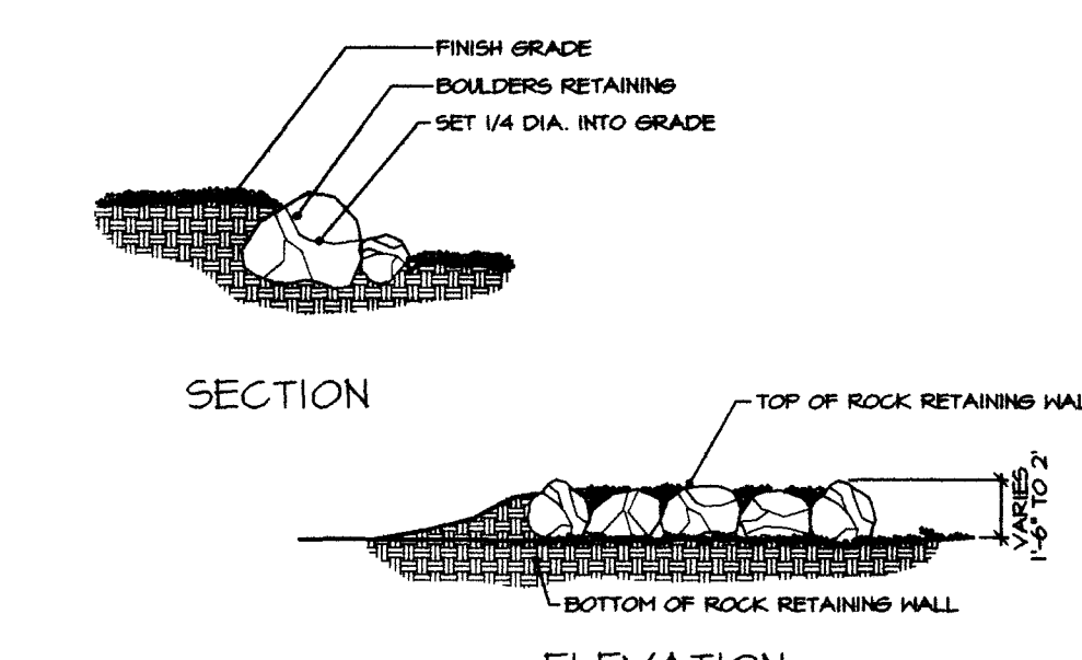
F BOULDER RETAINING WALL
