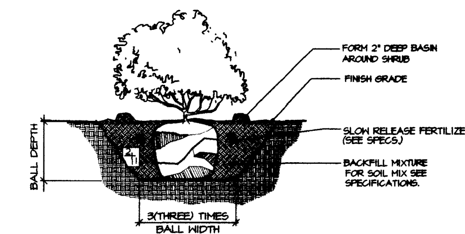
B SHRUB PLANTING
