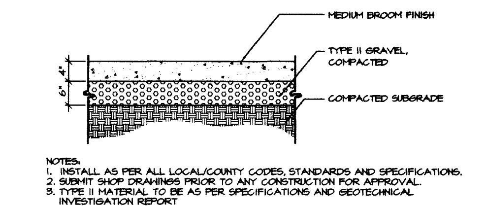
L CONCRETE WALK/PLAZA AREA
