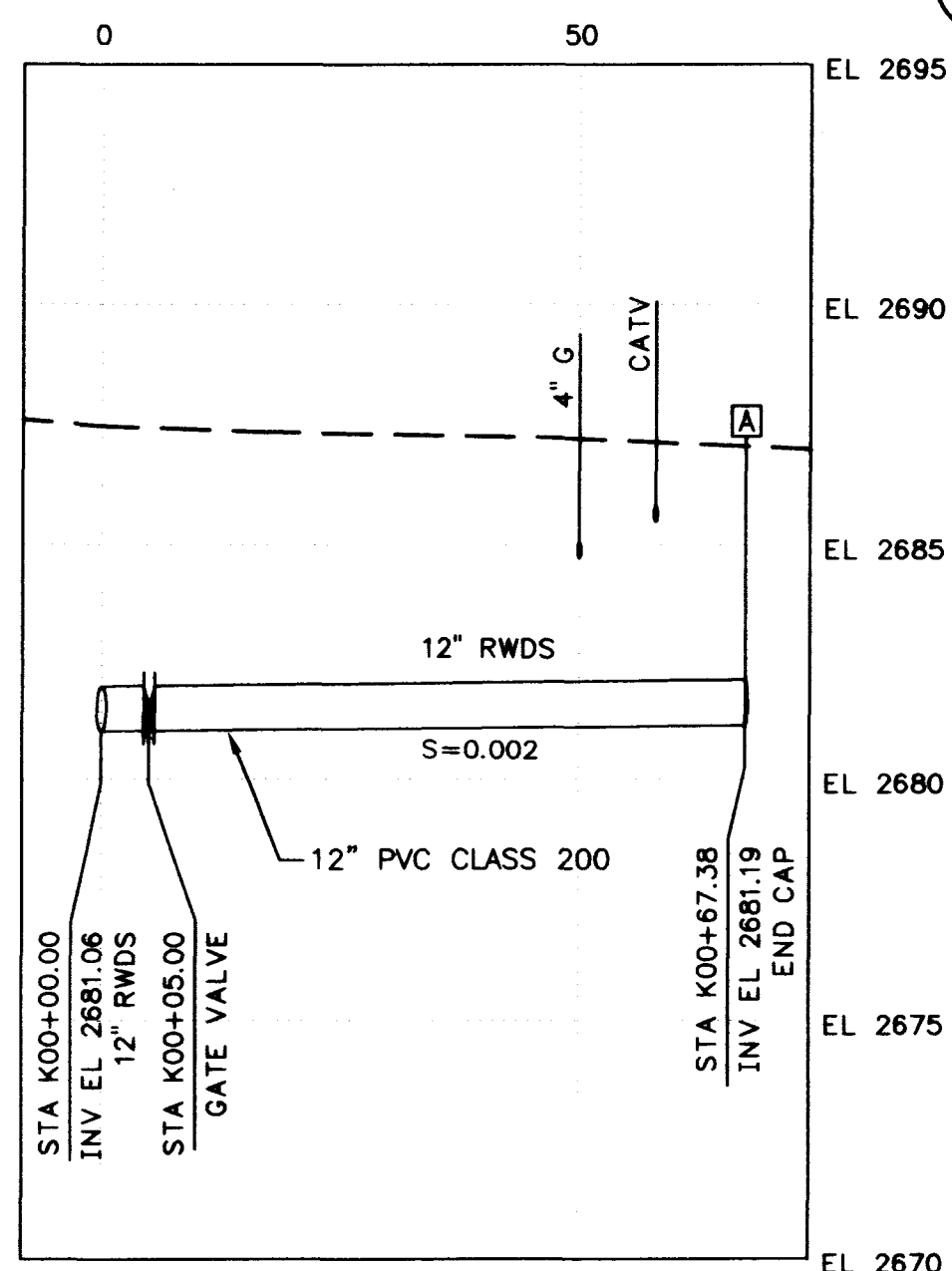
BRANCH 'K' - 12" AT STA 192+02.67 (10) (C17)
