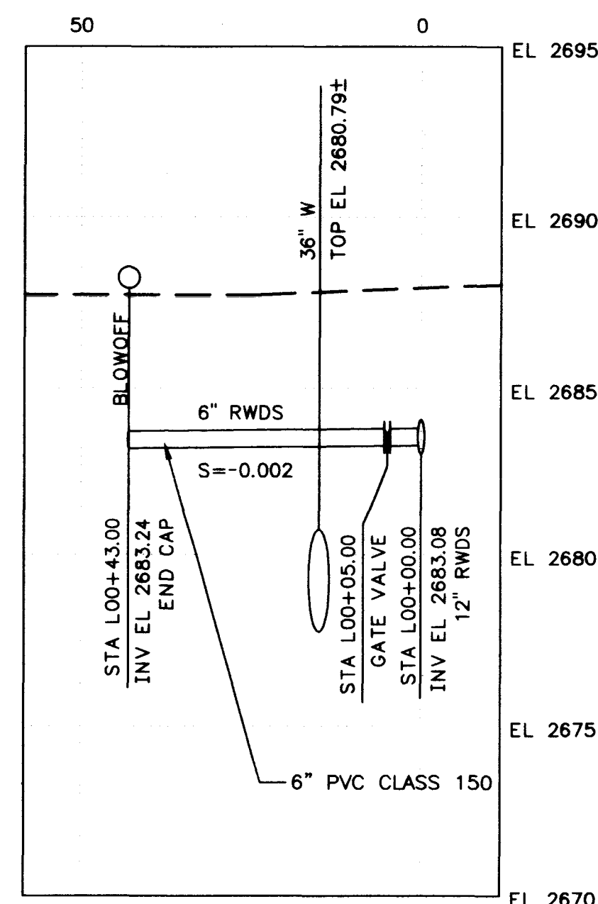
BRANCH 'L' - 6" AT STA 196+02.75 (11) (C18)
