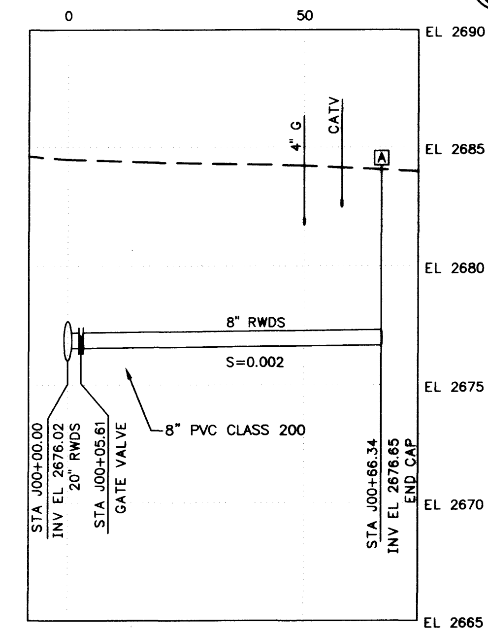
BRANCH 'J' - 8" AT STA 188+00.00 (9) (C17)
