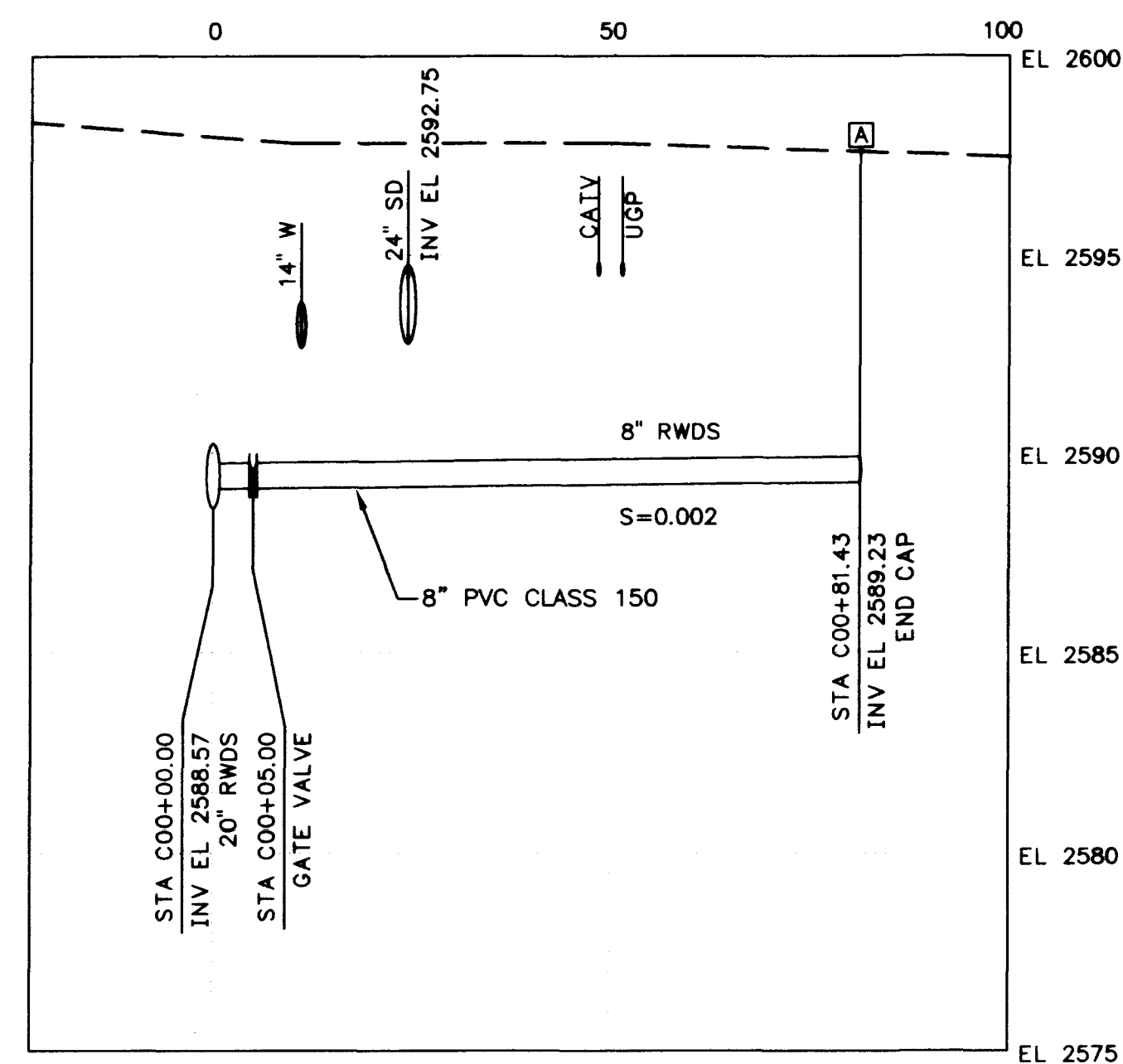
BRANCH 'C' - 8" AT STA 102+85.96 (3) (C9)
