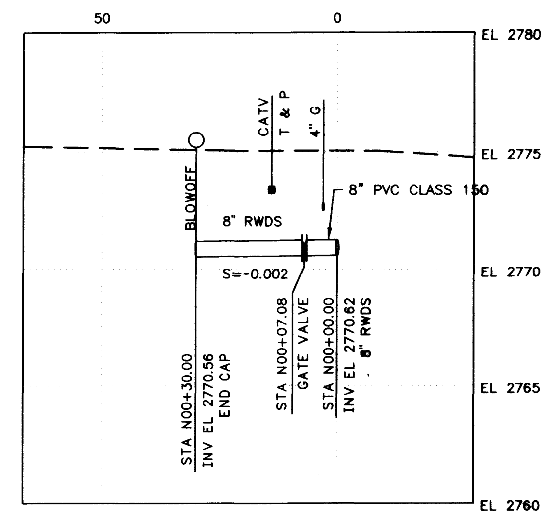
BRANCH 'N' - 8" AT STA 272+10.00 (13) (C25)
