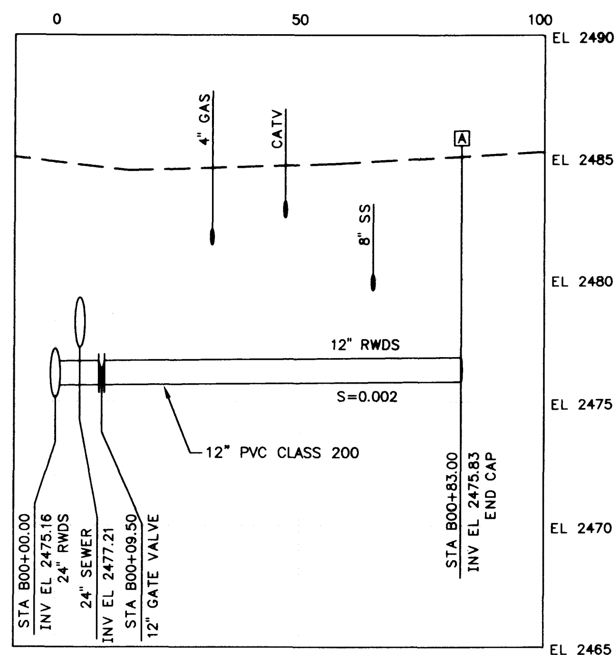
BRANCH 'B' - 12" AT STA 42+60.00 (2) (C4)
