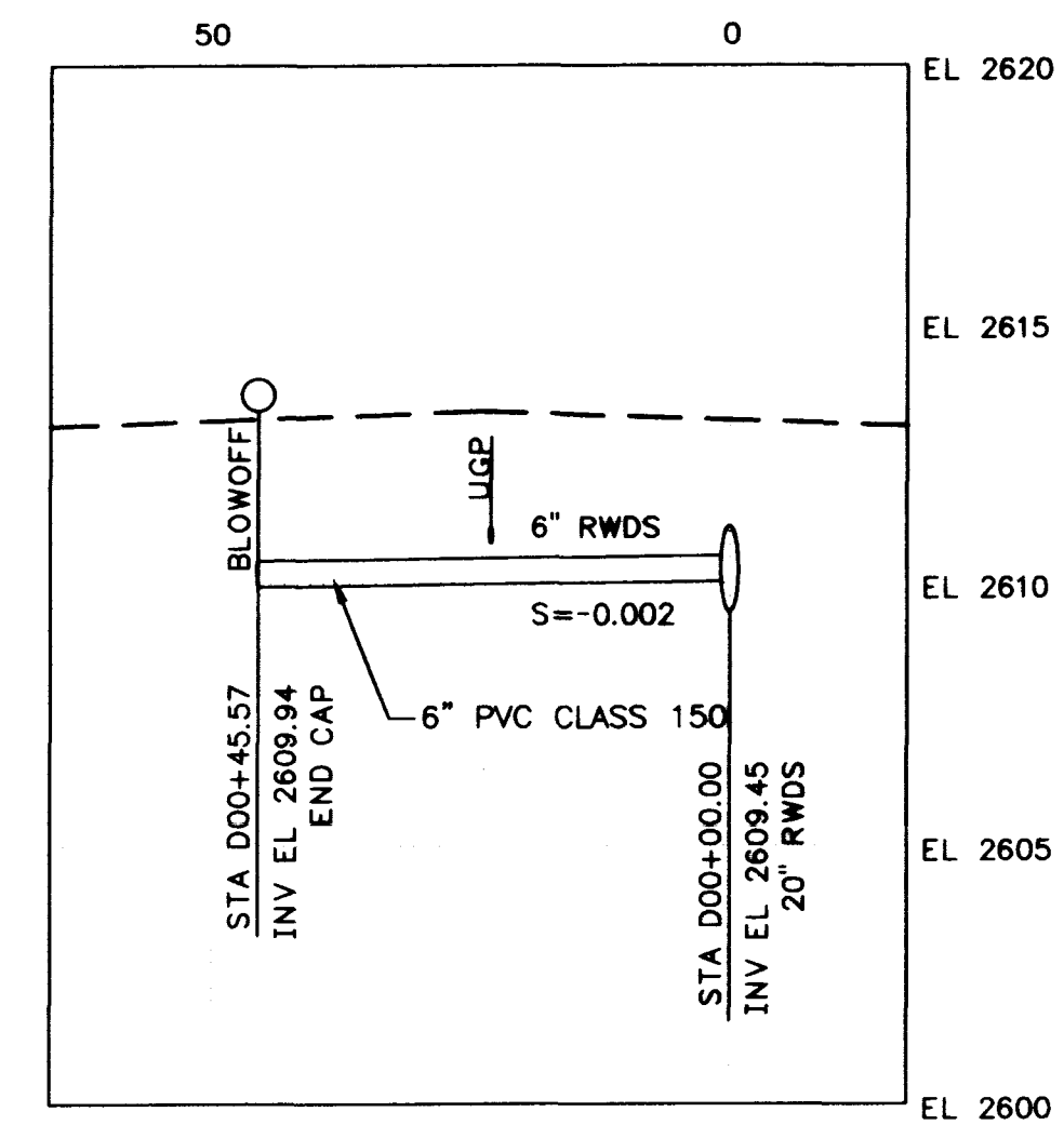
BRANCH 'D' - 6" AT STA 115+30.00 (4) (C10)
