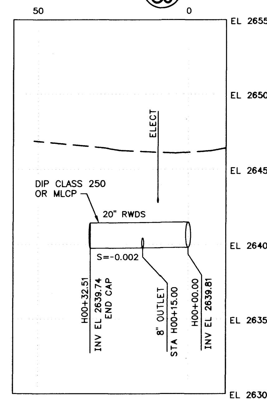
TURNOUT 'H' - 20" AT STA 140+13.31 (8) (C12)
