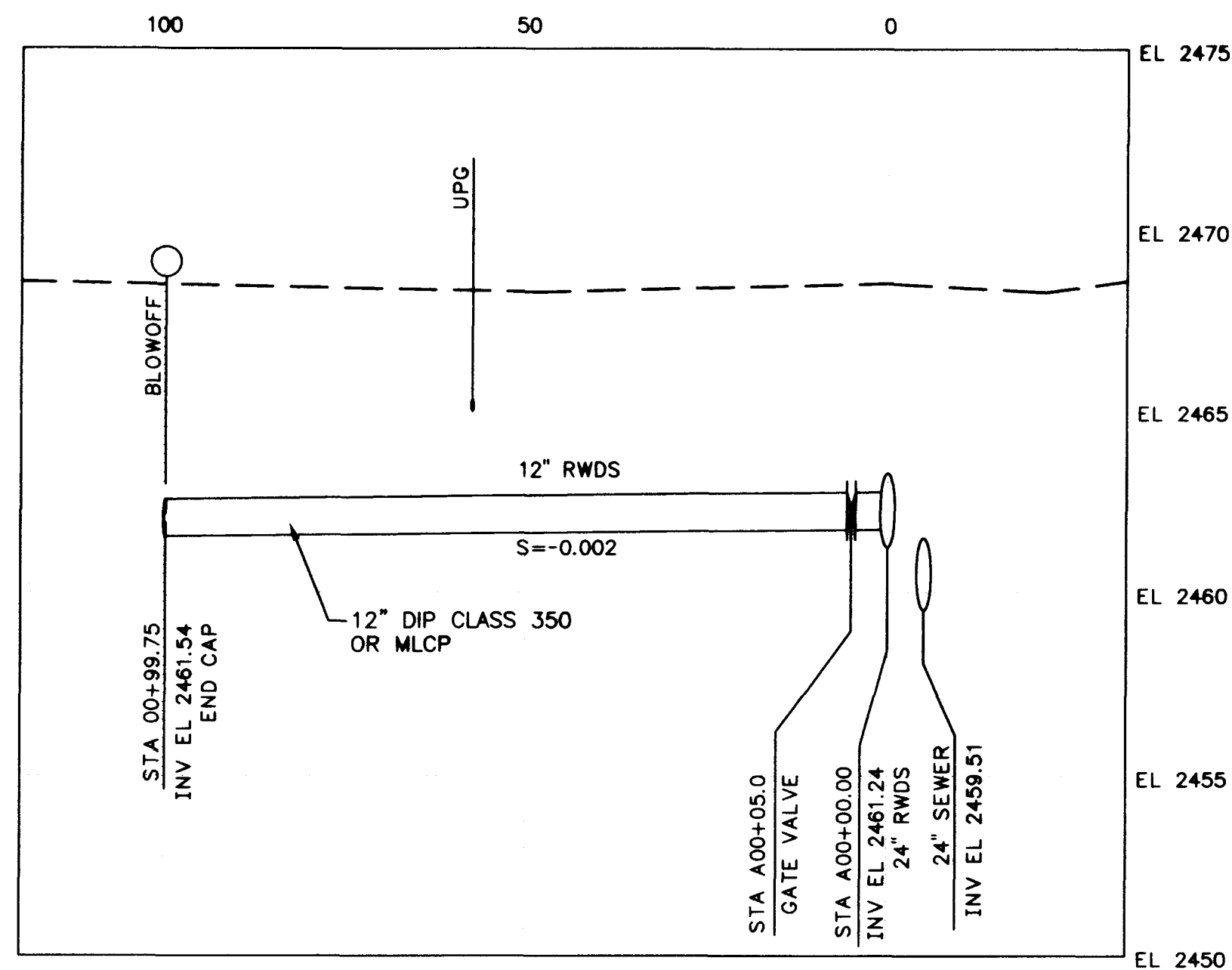
BRANCH 'A' - 12" AT STA 28+50.00 (1) (C2)
