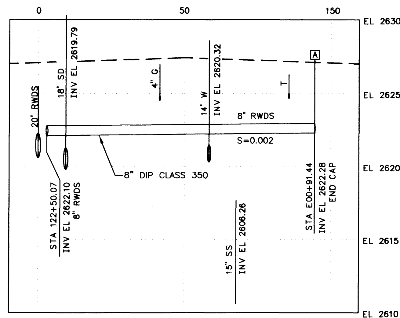
BRANCH 'E' - 8" AT STA 122+50.07 (5) (C11)
