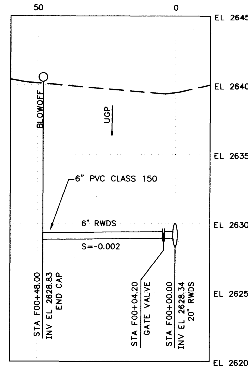
BRANCH 'F' - 6" AT STA 128+60.00 (6) (C11)
