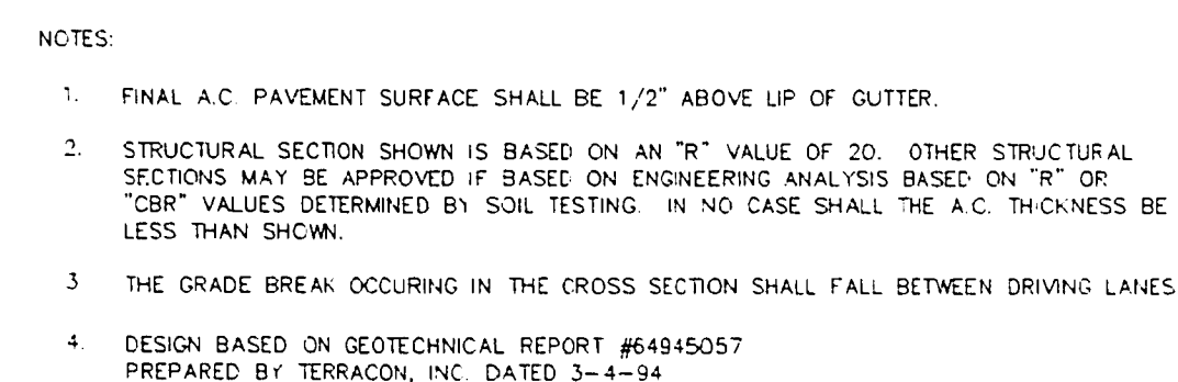
JAMES BILBRAY DR. STREET SECTION DETAIL STD. DWG. NO. 205
