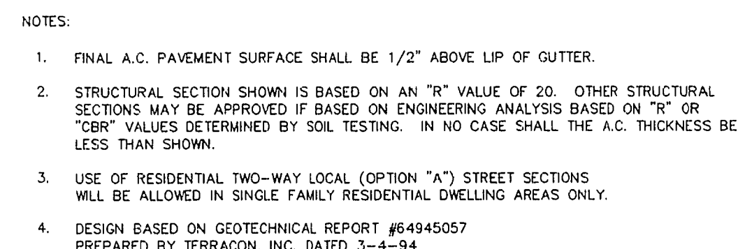
51' ROW STREET SECTION DETAIL STD. DWG. NO. 206
