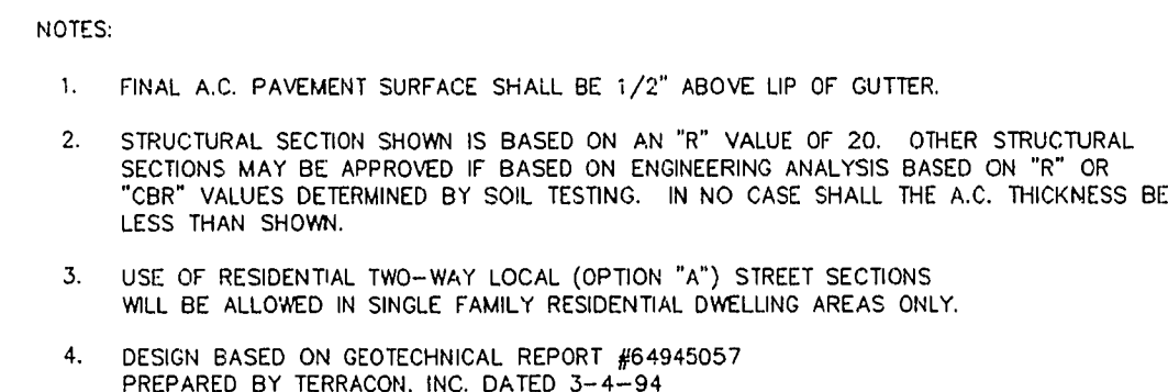
AVERY DRIVE SECTION DETAIL SECTION C-C N.T.S. STD. DWG. #206
