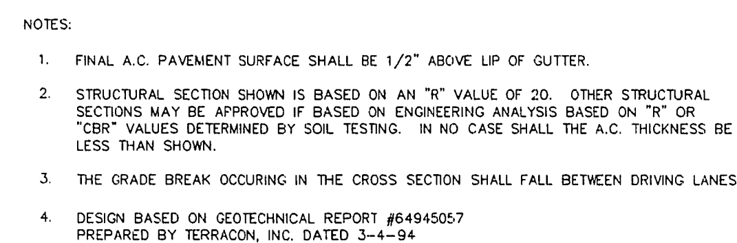
JAMES BILBRAY DR. E - E SECTION DETAIL STD. DWG. NO. 205
