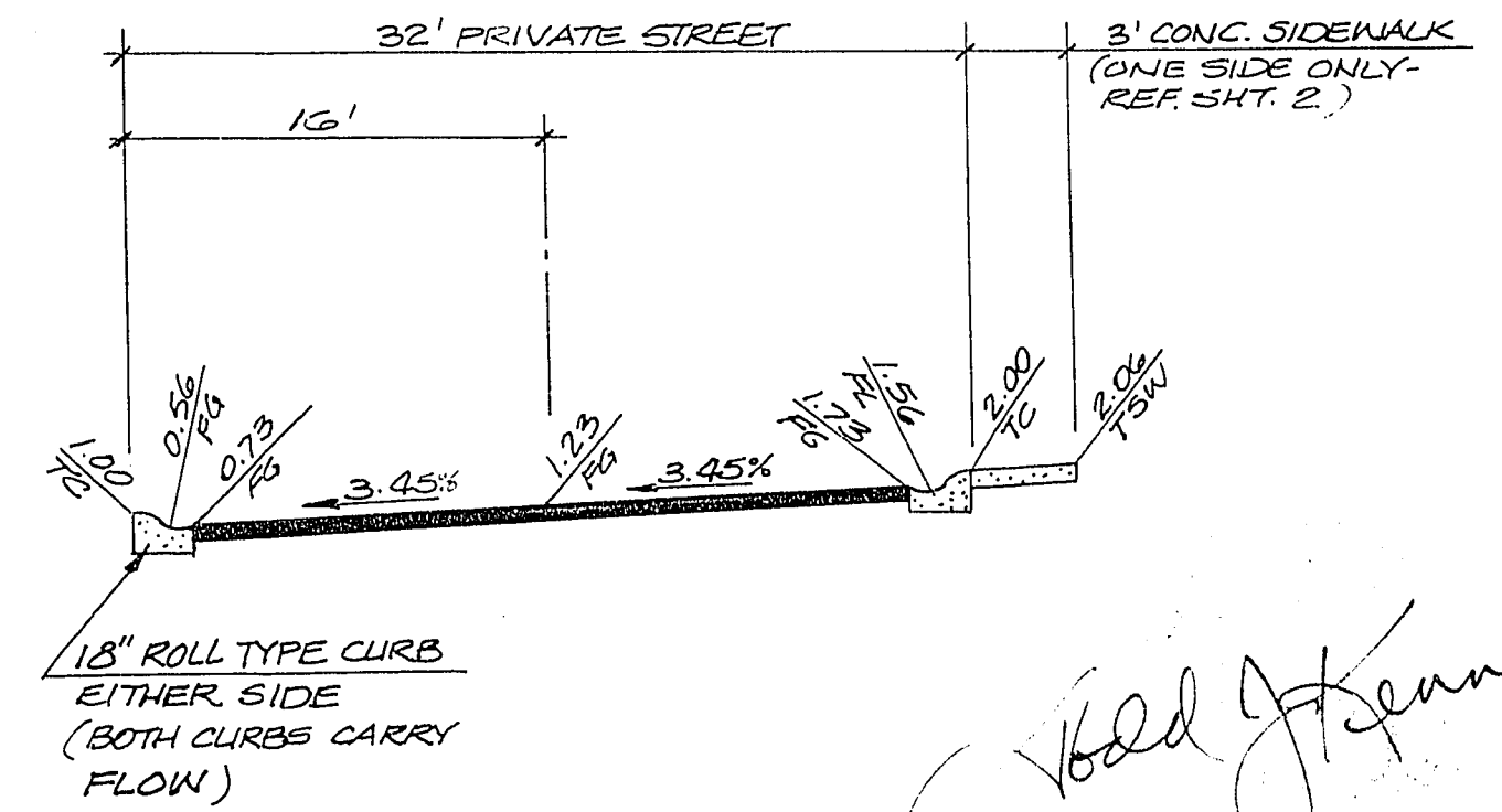
TYPICAL ONSITE SECTION
