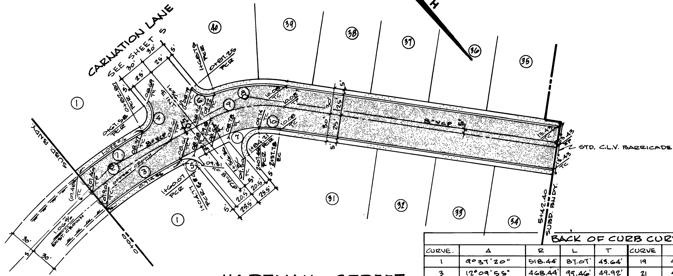
HARTMAN STREET SCALES: 1"=50' HOR.; 1"=2' VER.
