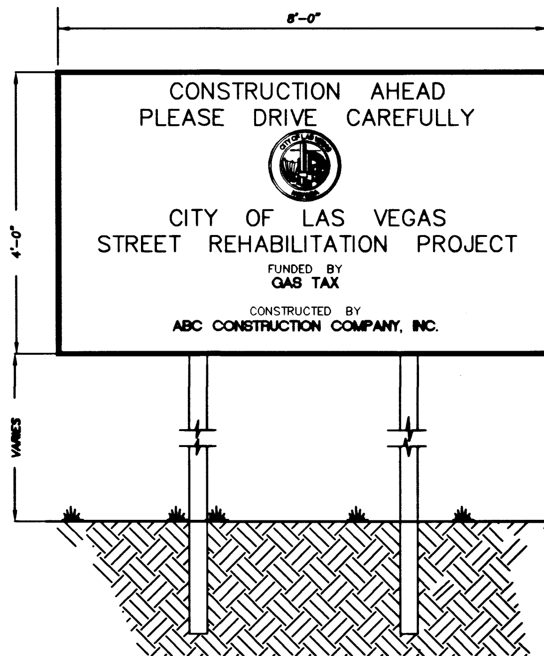
PROJECT SIGN
