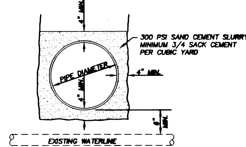
STORM DRAIN ENCASEMENT DETAIL
