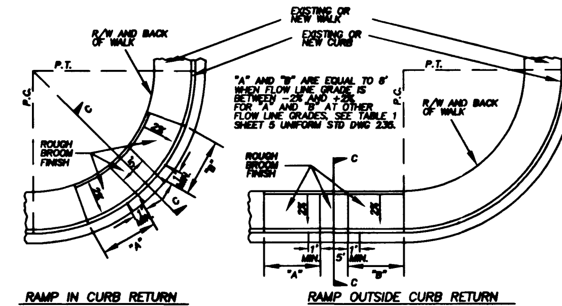
RAMP IN CURB RETURN
