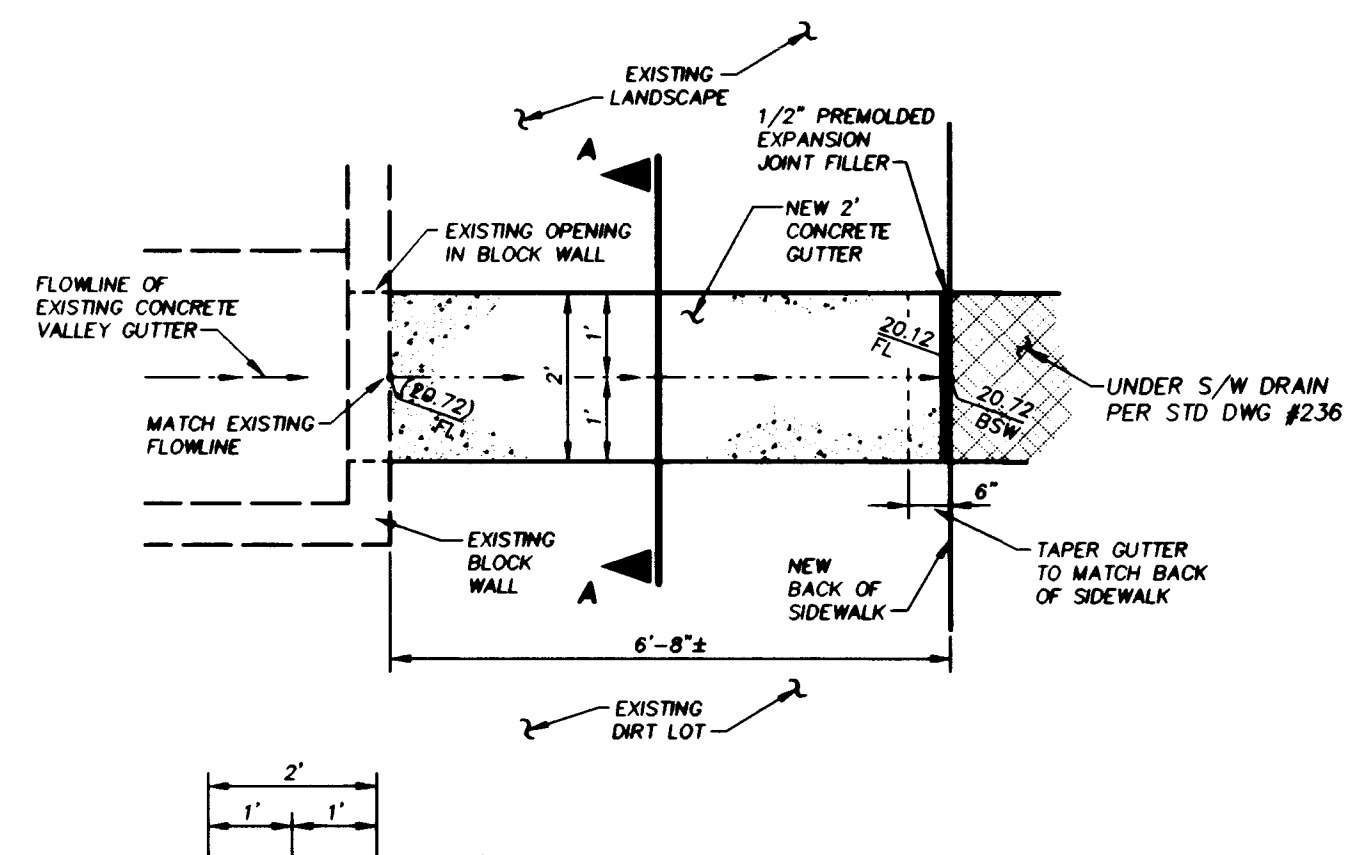
CONCRETE GUTTER
