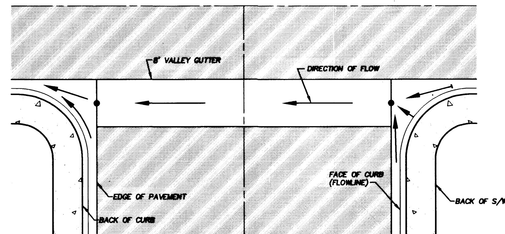
FLOWLINE GRADING & VALLEY GUTTER
