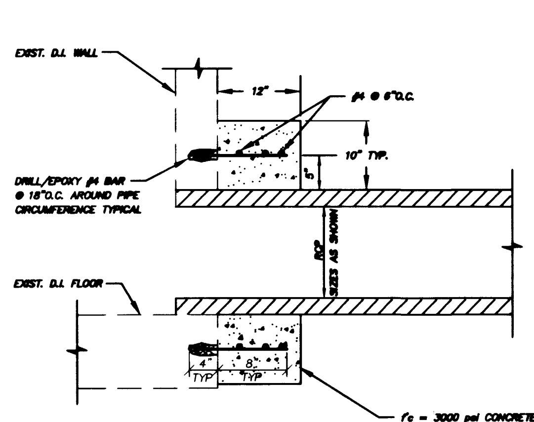
CONCRETE COLLAR
