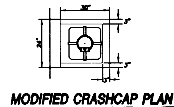
MODIFIED CRASHCAP PLAN
