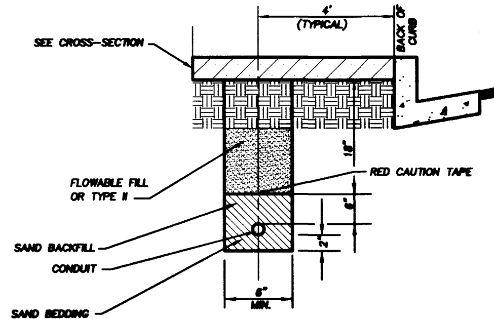
TRENCH DETAIL
