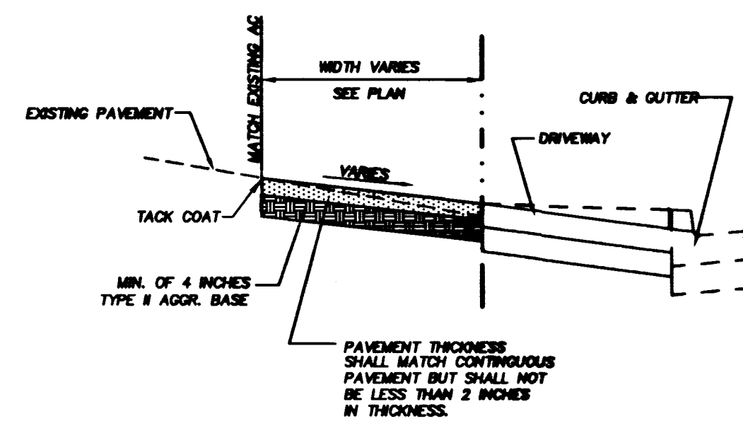
MISCELLANEOUS ASPHALT PATCH
