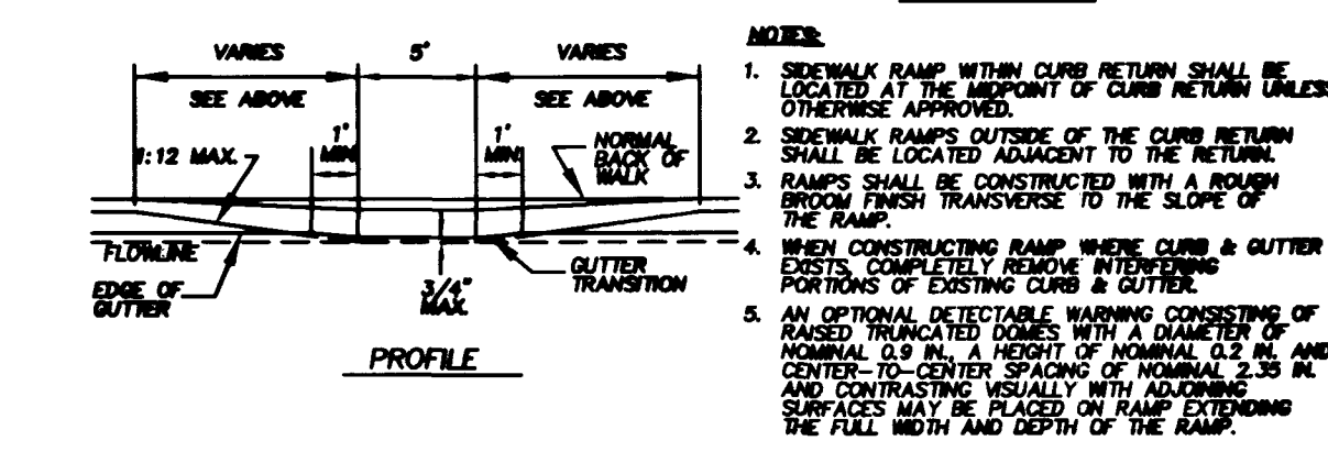
SIDEWALK RAMP CASE 1A
