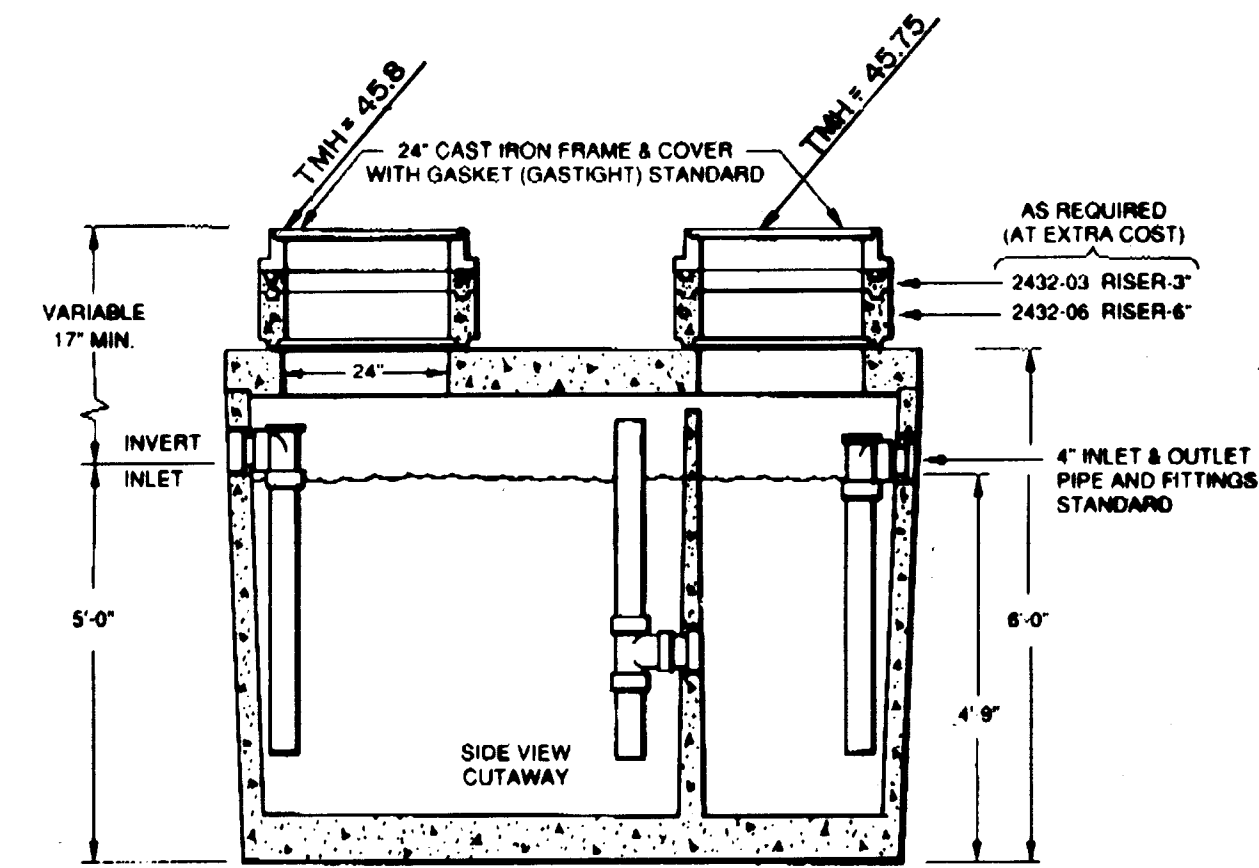
GREASE PIT DETAIL
