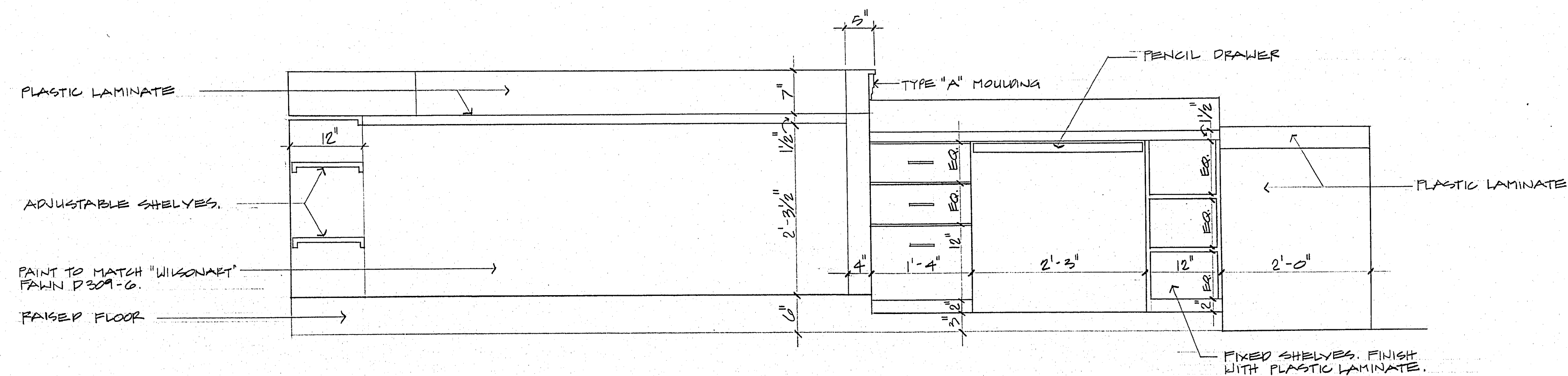
ELEVATION #4 1"=1'-0"
