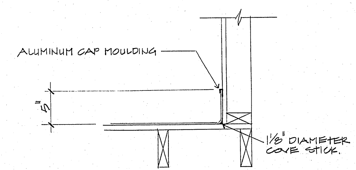
VINYL FLOORING COVE 1/2" = 1'-0"
