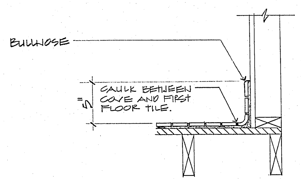
CERAMIC TILE COVE 1/2" = 1'-0"
