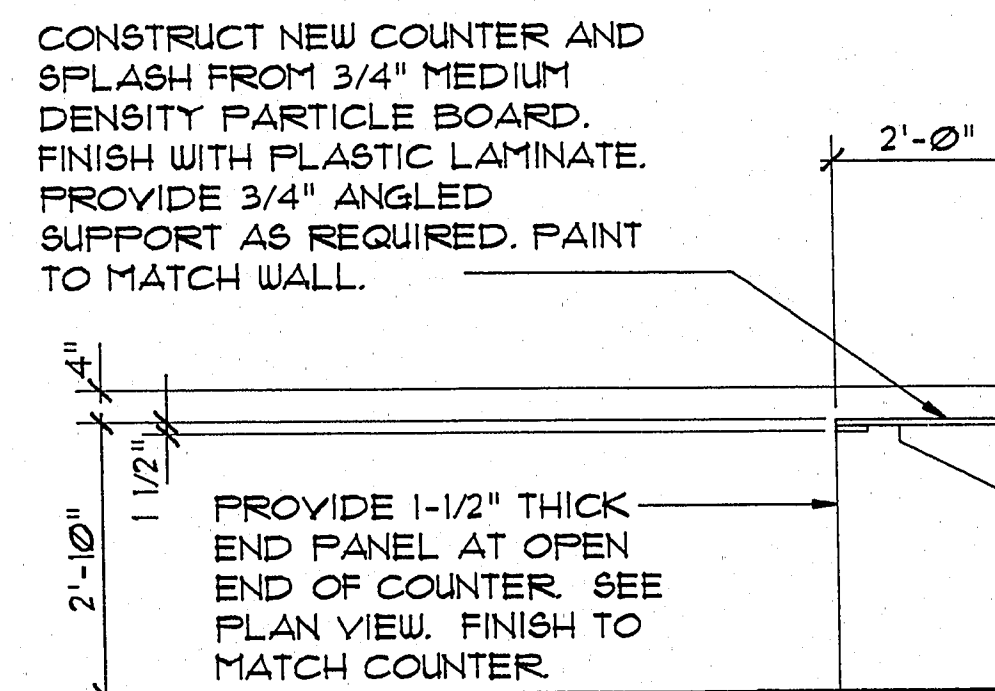
CROSS SECTION "G"
