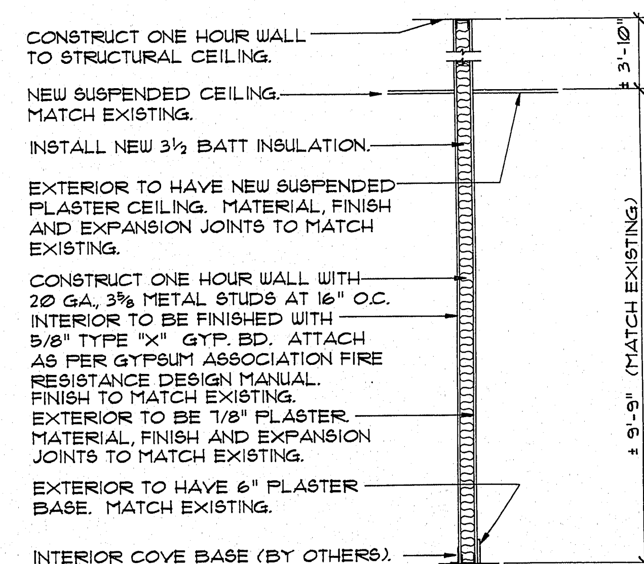
CROSS SECTION "L"
