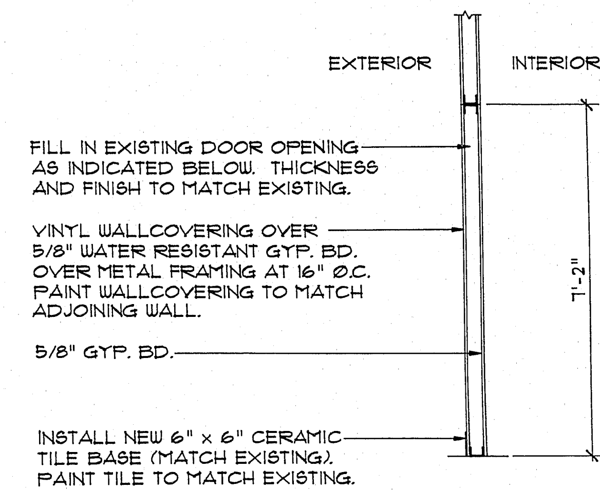
CROSS SECTION "D"
