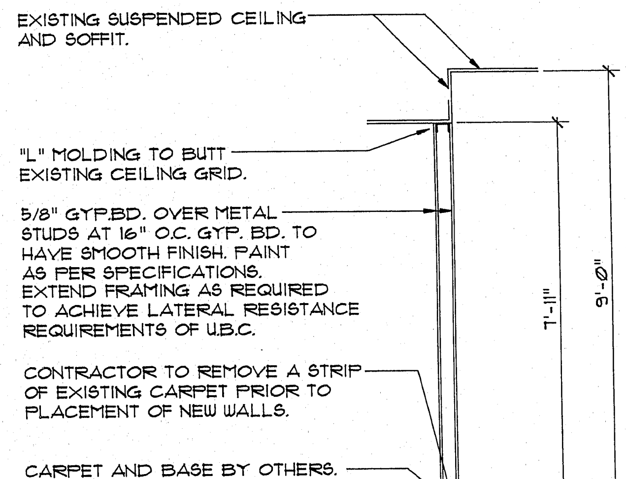
CROSS SECTION "E"
