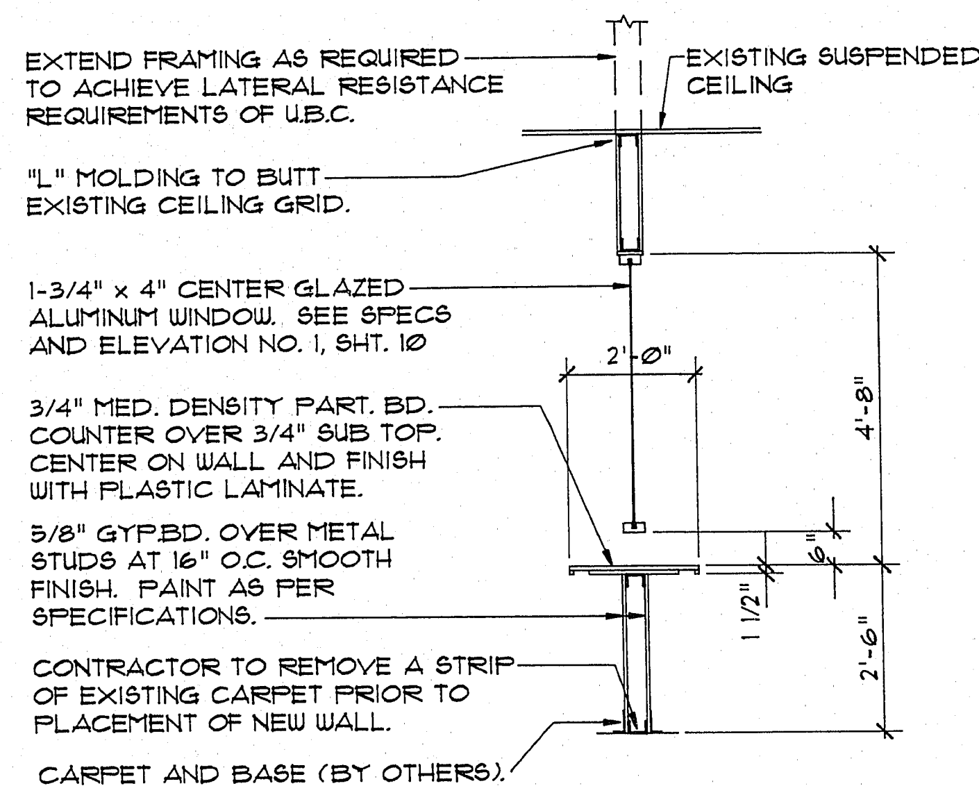
CROSS SECTION "B"
