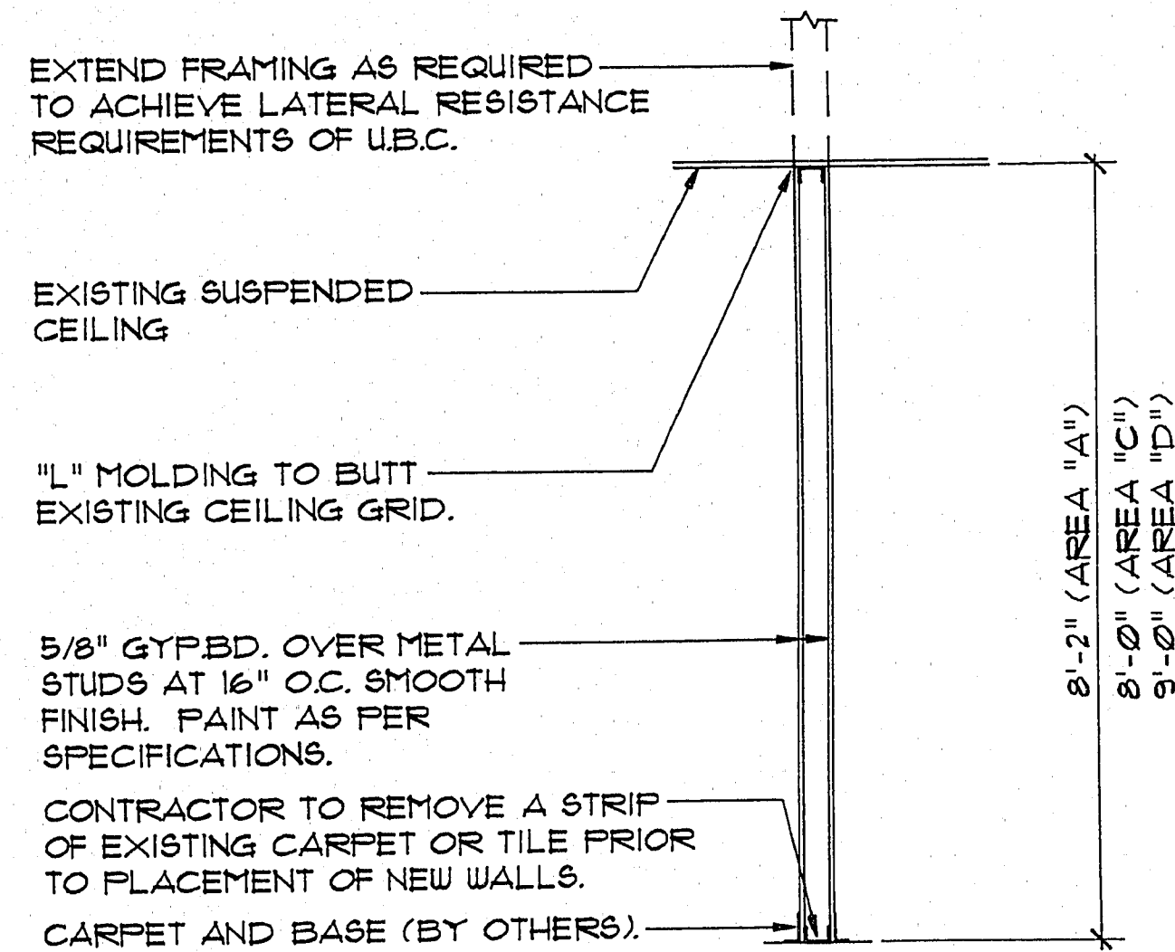
CROSS SECTION "A"
