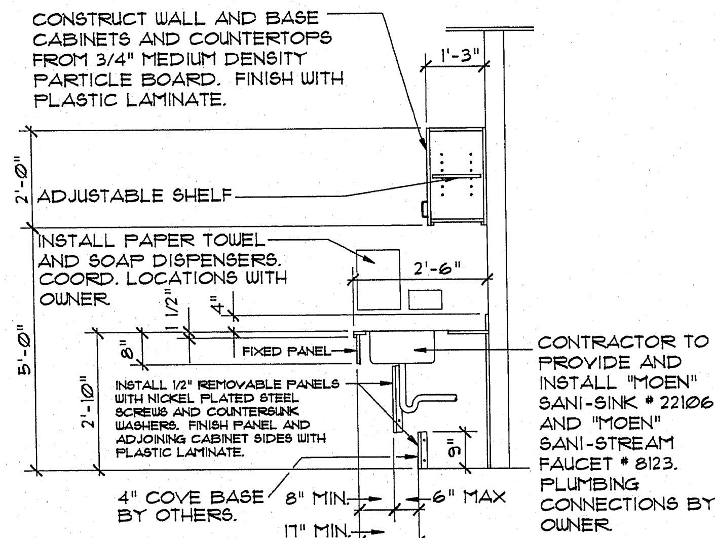
CROSS SECTION "F"
