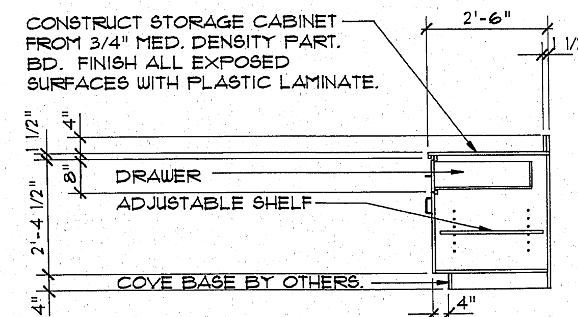
CROSS SECTION "K"
