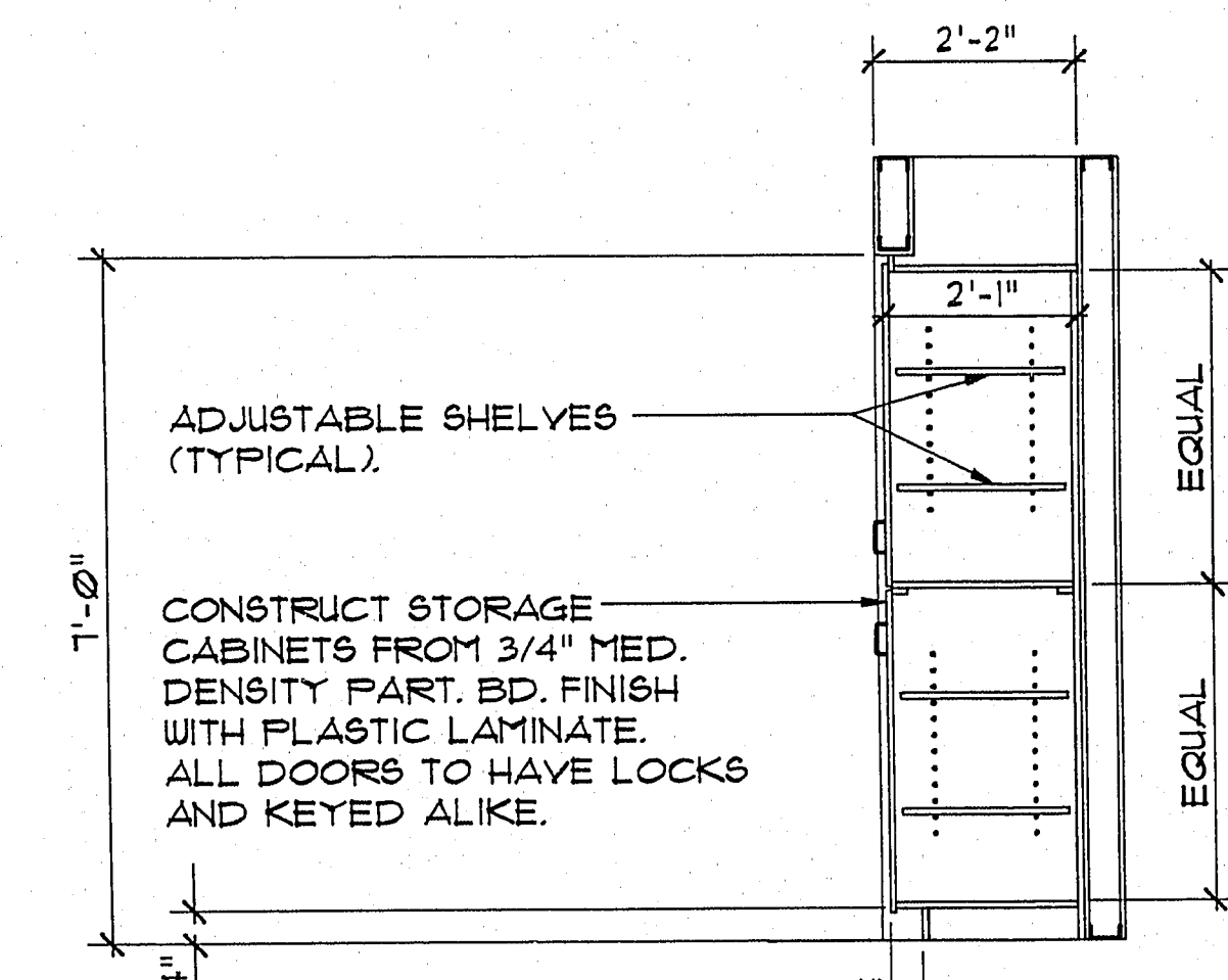
CROSS SECTION "H"
