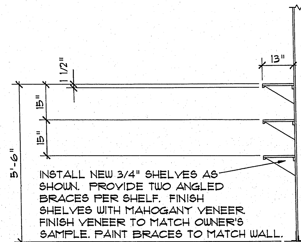
CROSS SECTION "J"
