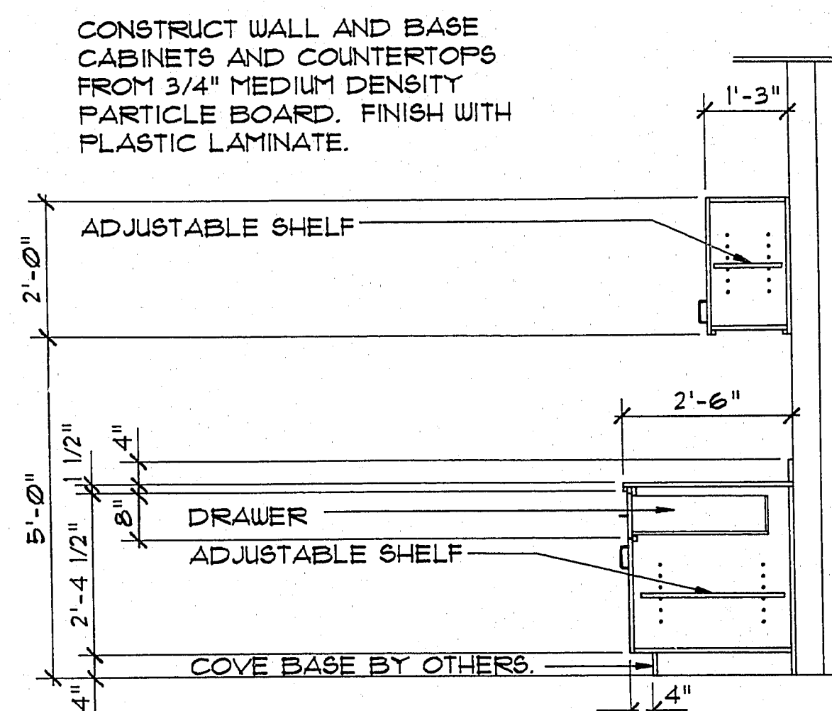
CROSS SECTION "C"
