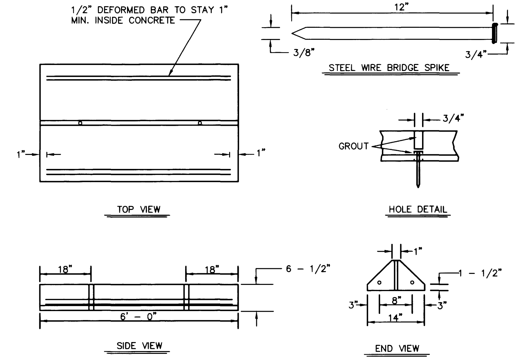
PRECAST BUMPER BLOCK 1 C3.01
