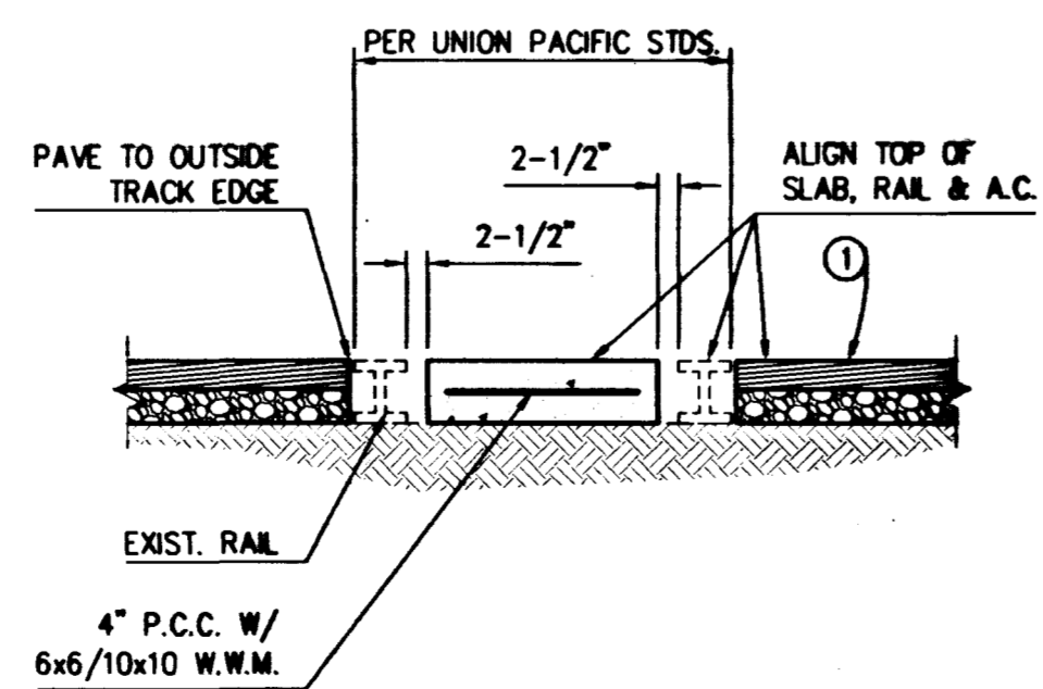
3 TRACK CROSSING N.T.S.
