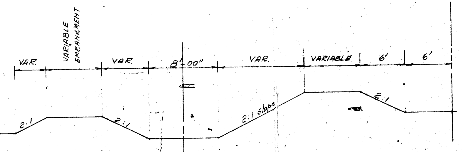
SECTION A-A No Scale
