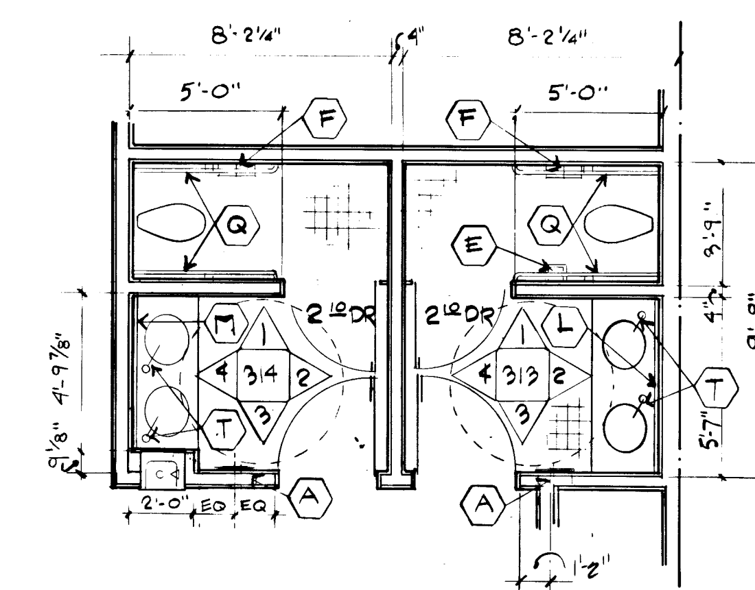
TOILET RM. PLAN 233/234
