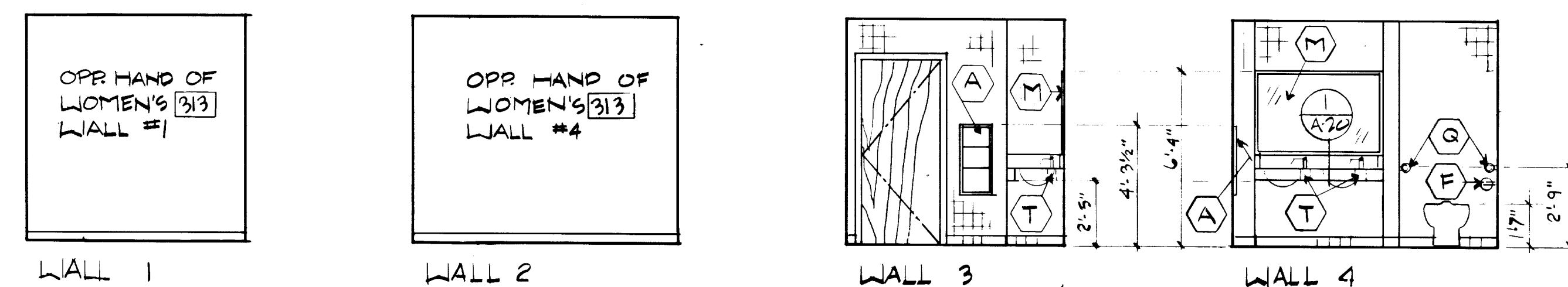
MEN'S TOILET RM. 234
