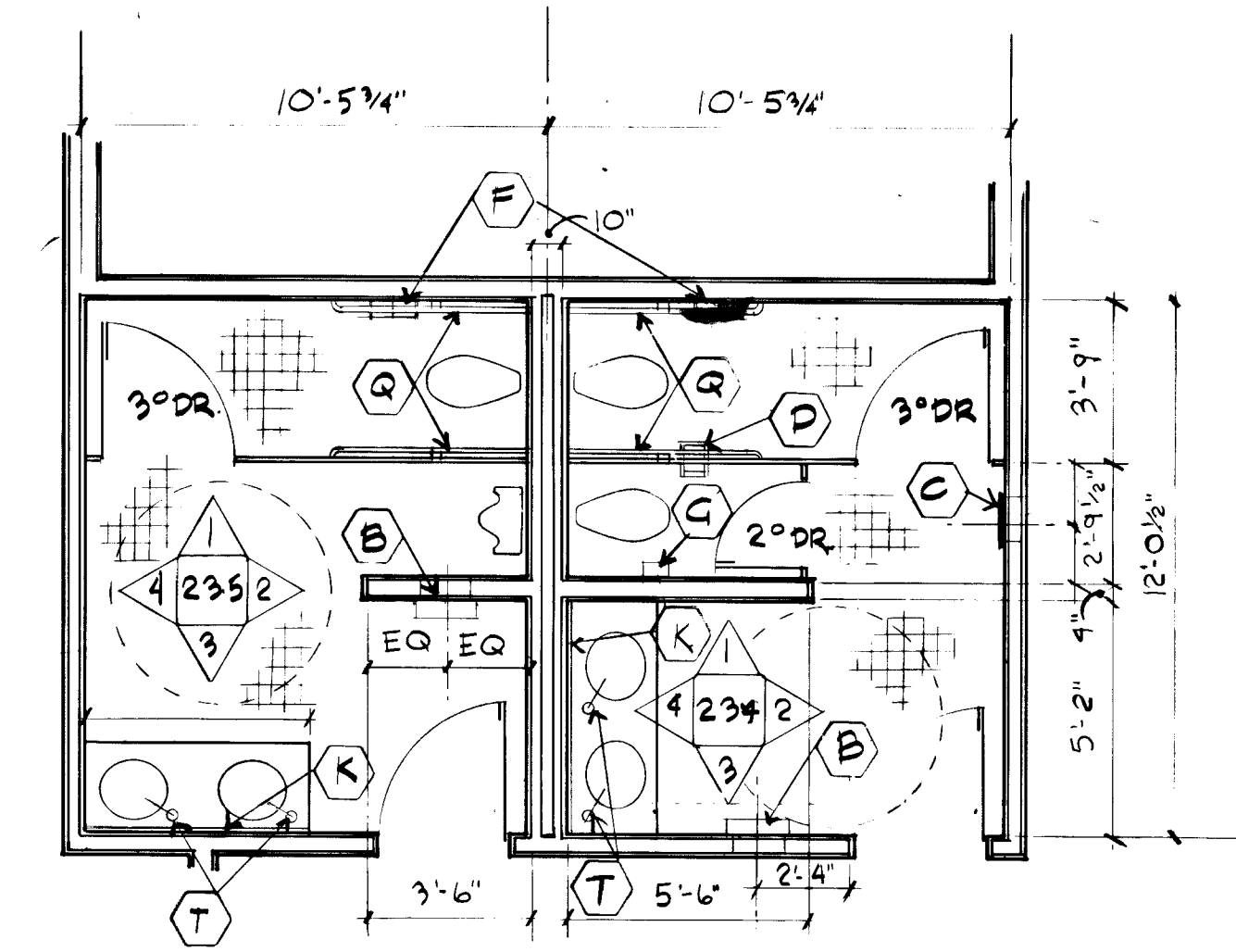
TOILET RM. PLAN 235/234
