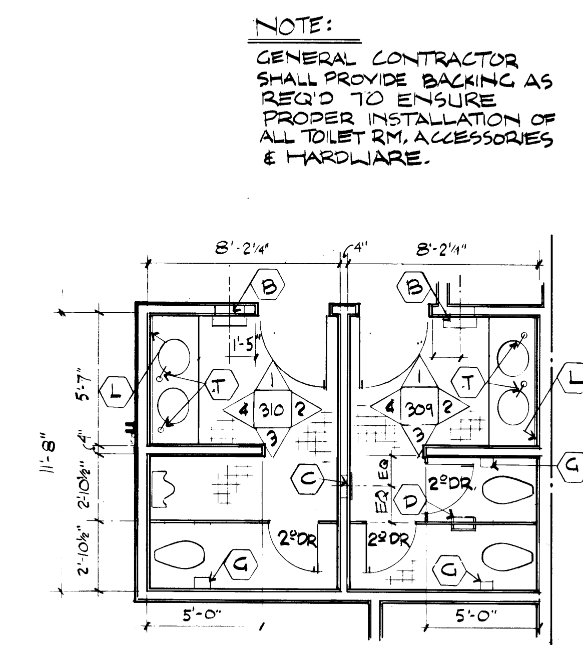
TOILET RM. PLAN 2309/2310
