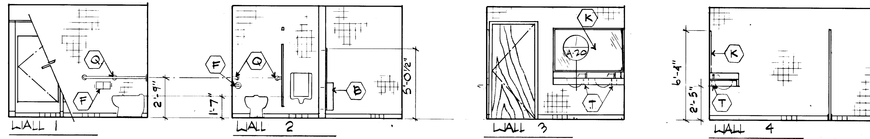
MEN'S TOILET RM. 235
