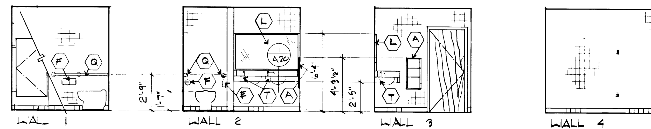
WOMEN'S TOILET RM. 233
