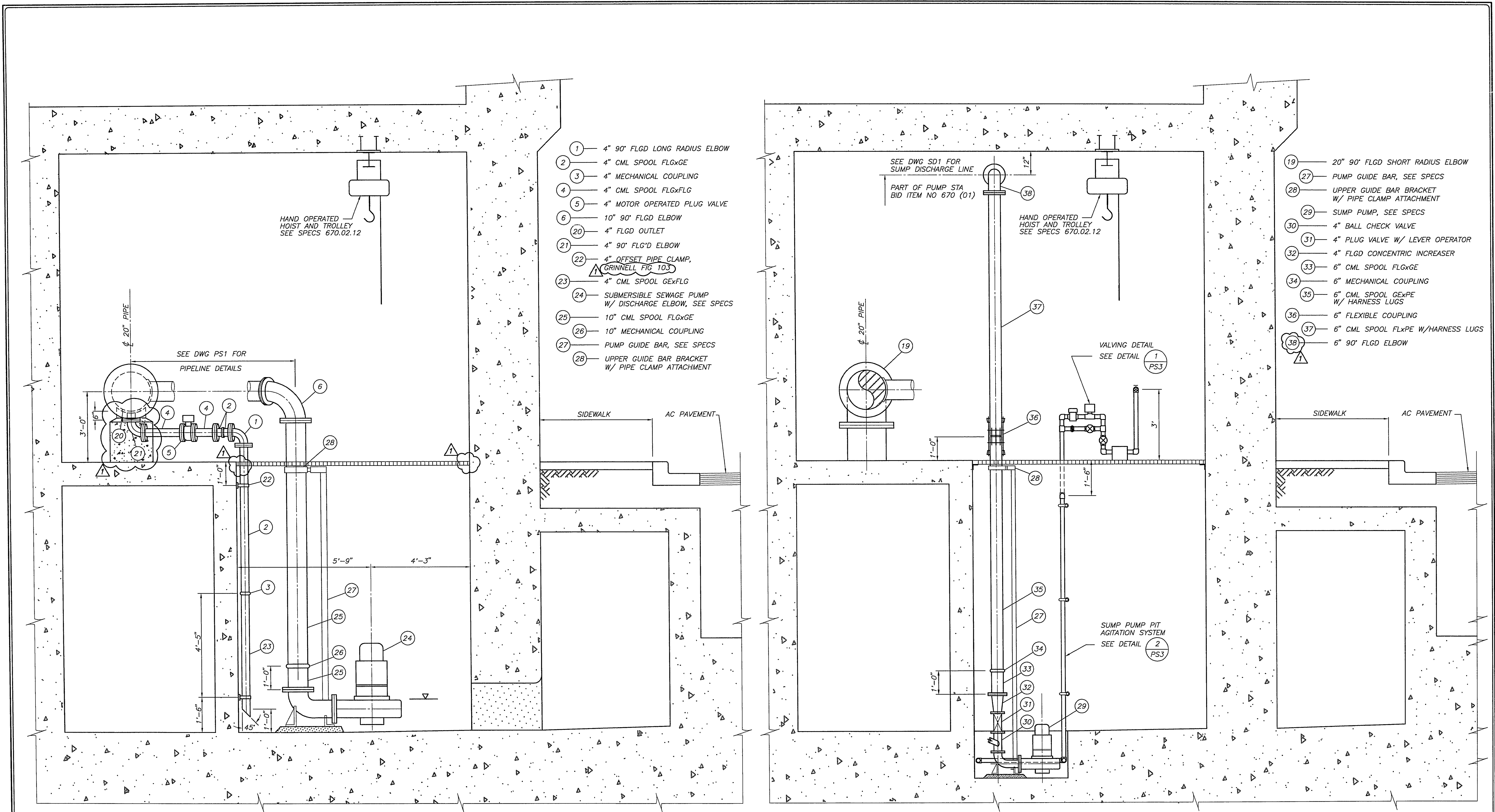
PUMPING STATION SECTION A SCALE: 1/2" = 1'-0" PS1
