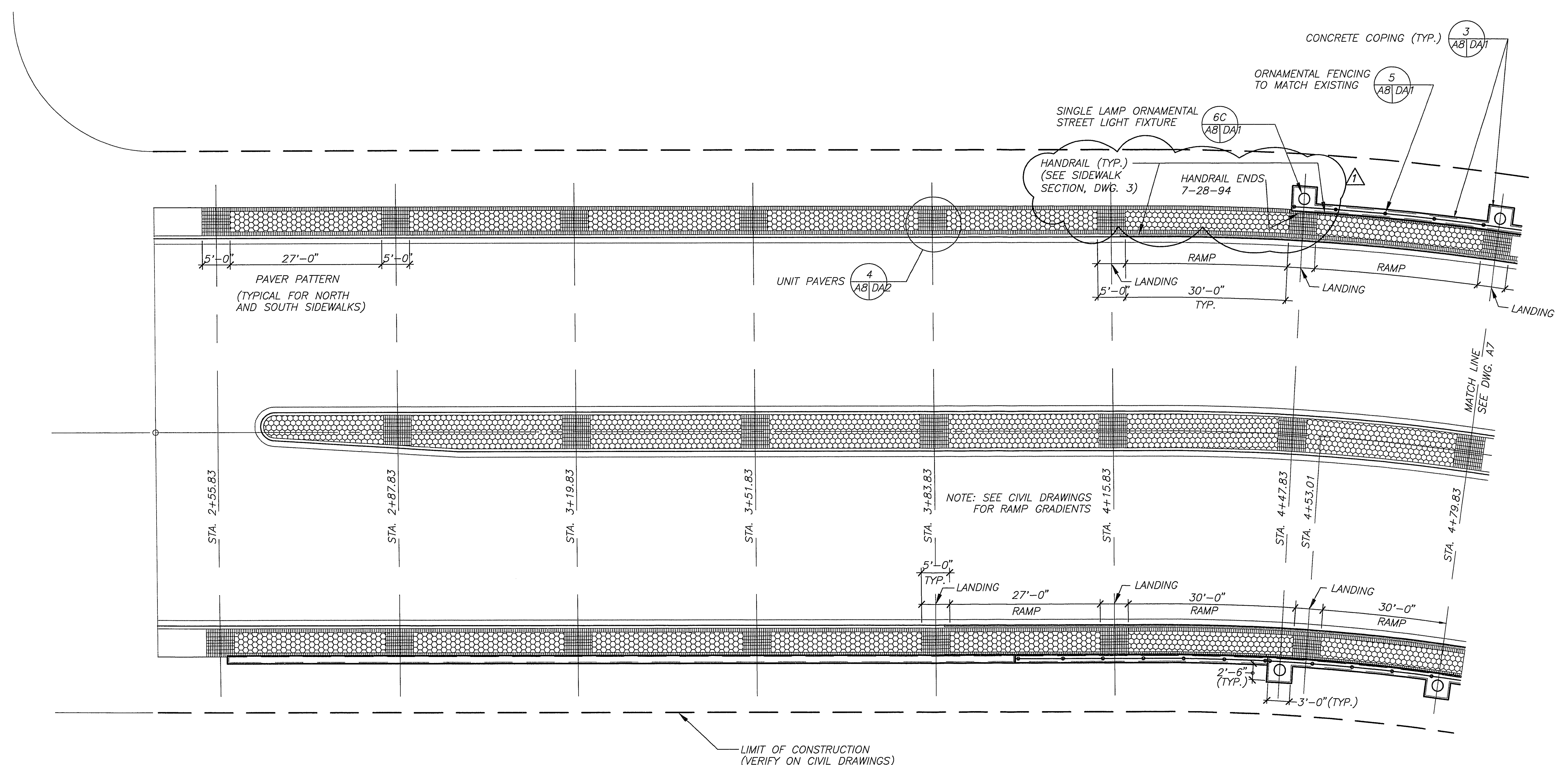
WEST ENTRY PLAN SCALE 1"=10'-0"
