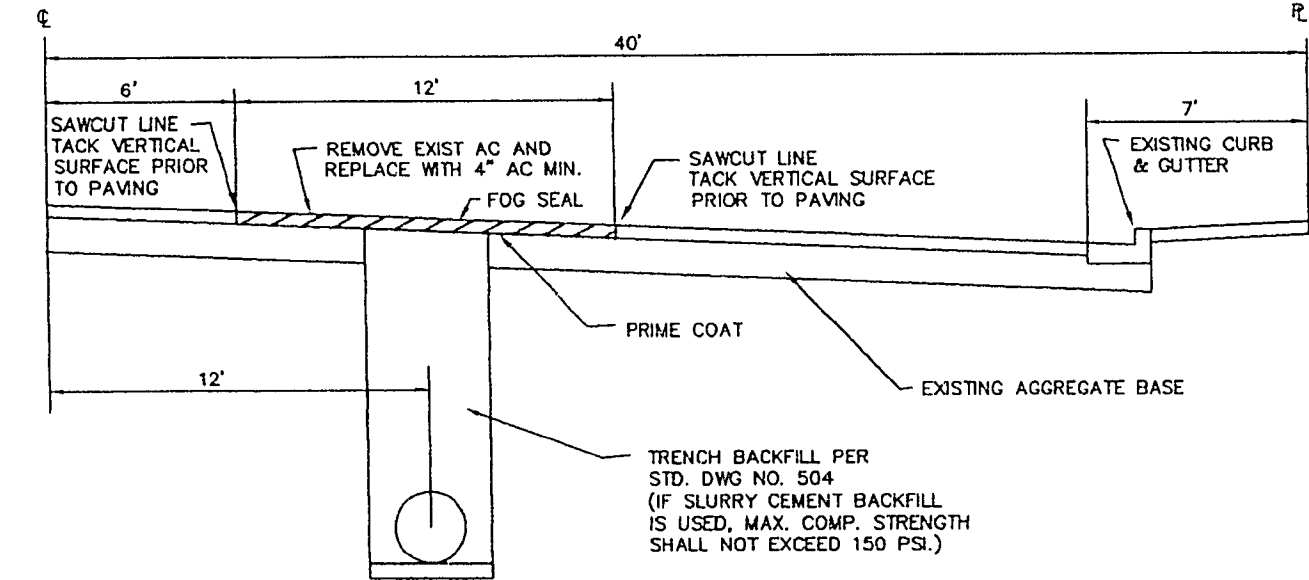
PAVEMENT REMOVAL AND REPLACEMENT DETAIL FOR STATION 71+64 TO STA 82+00
