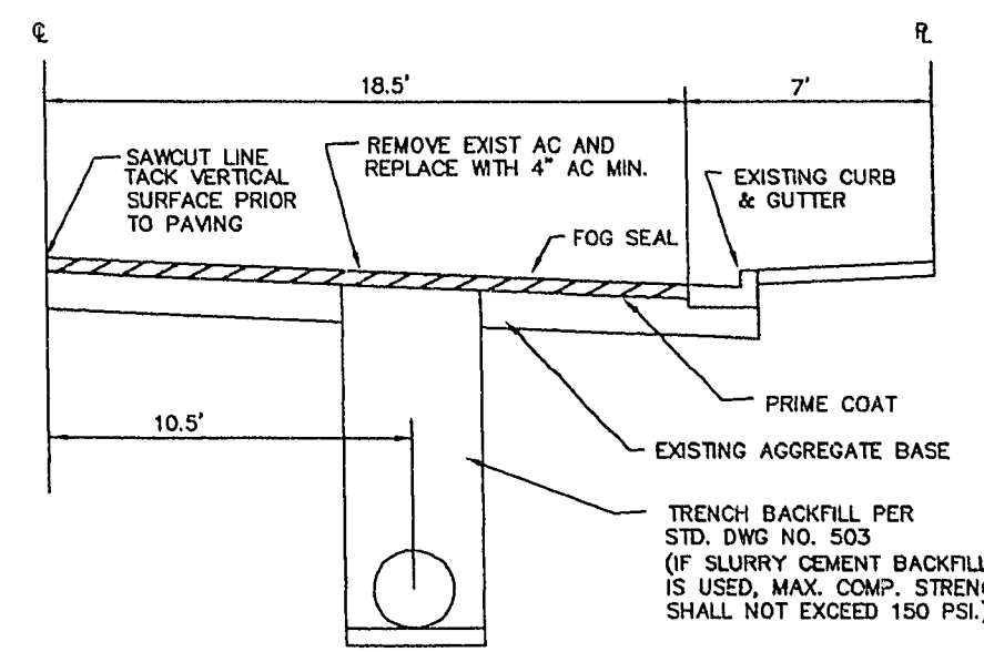
PAVEMENT REMOVAL AND REPLACEMENT DETAIL FOR STATION 47+63 TO STA 60+80
