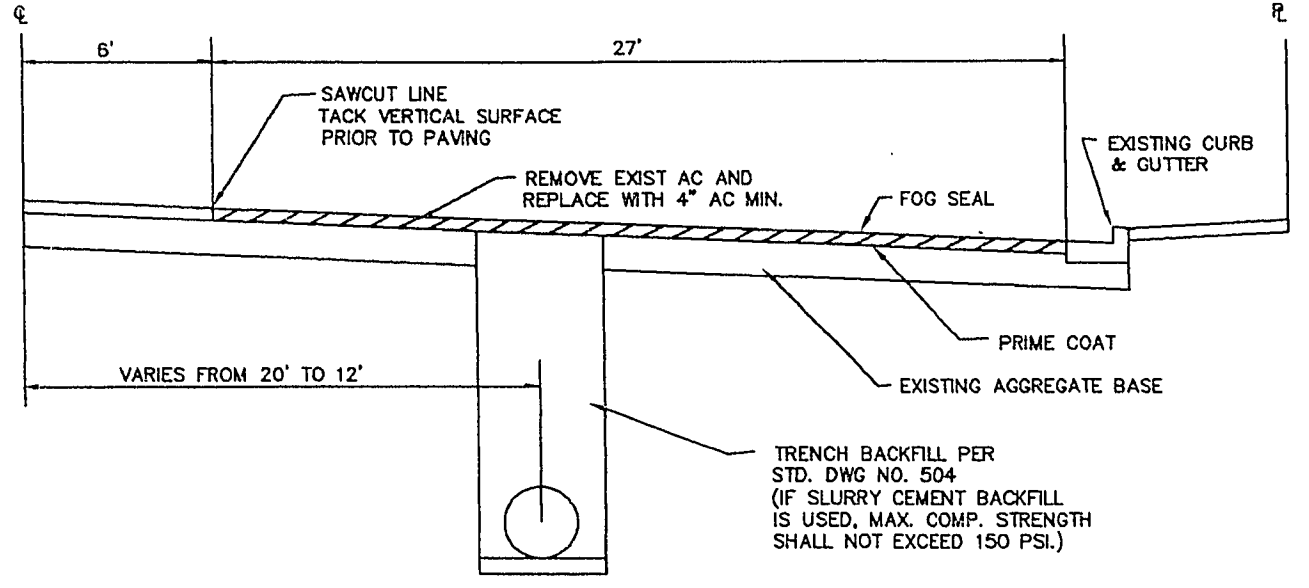
PAVEMENT REMOVAL AND REPLACEMENT DETAIL FOR STATION 60+80 TO STA 71+64
