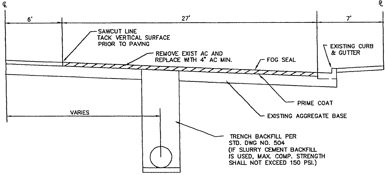
PAVEMENT REMOVAL AND REPLACEMENT DETAIL FOR STATION 37+52 TO STA 40+20
