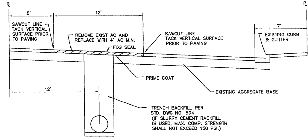
PAVEMENT REMOVAL AND REPLACEMENT DETAIL FOR STATION 40+20 TO STA 47+63
