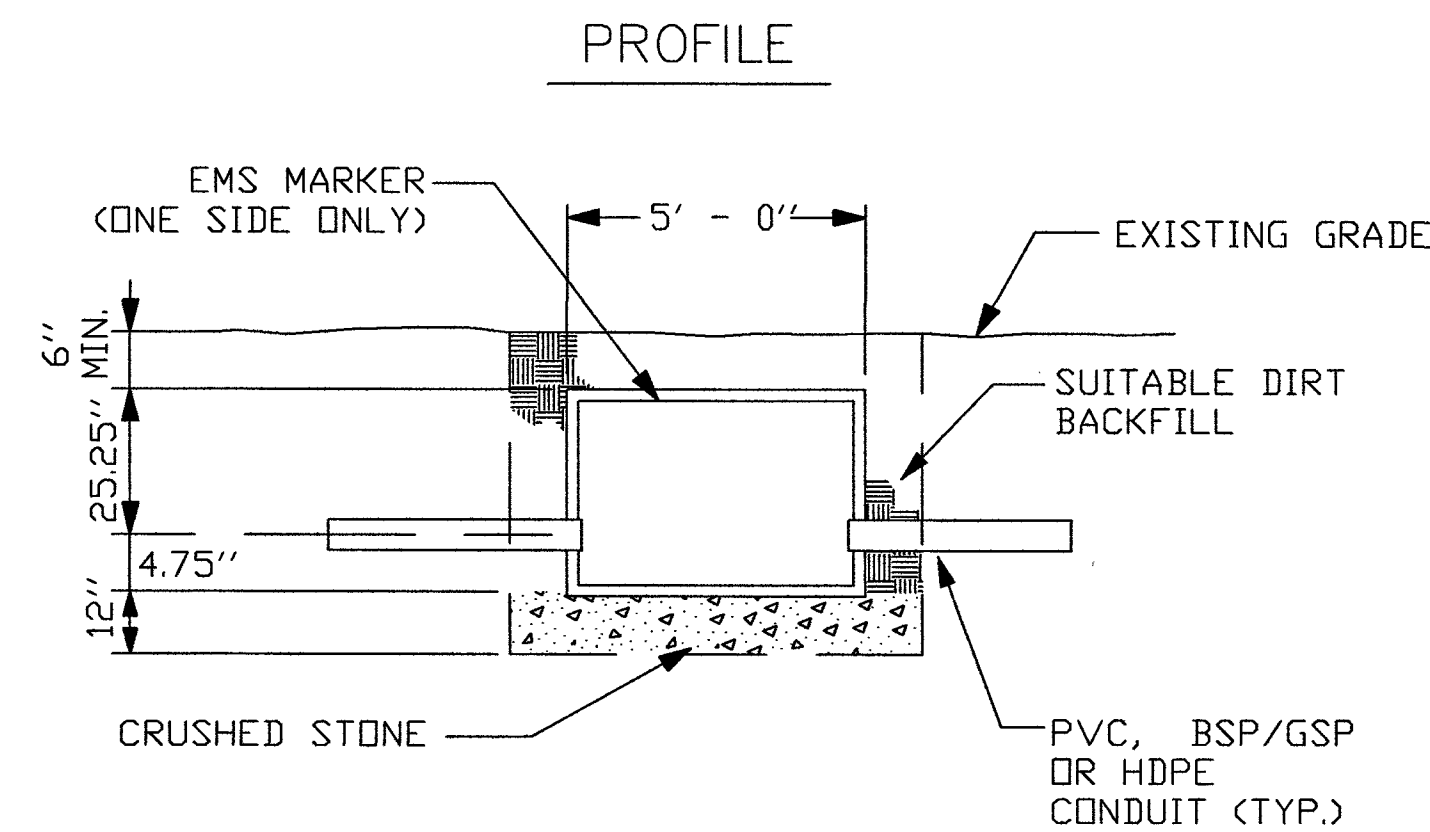
DETAIL "C" EXCAVATION PIT
