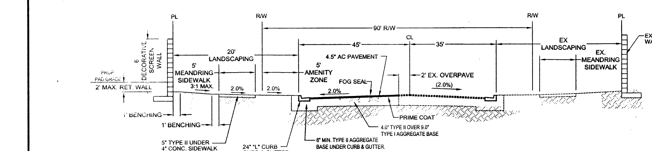
SECTION 'Q' NTS 90' R/W HORSE DRIVE (PUBLIC)
