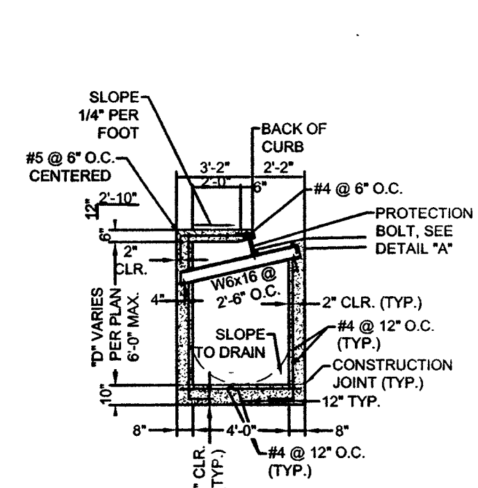
TYPE 'CM' DROP INLET SECTION SCALE 3/4"=1'
