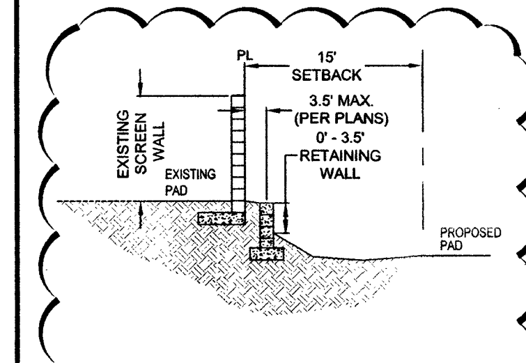
SECTION 'E' NTS NORTH PROPERTY LINE
