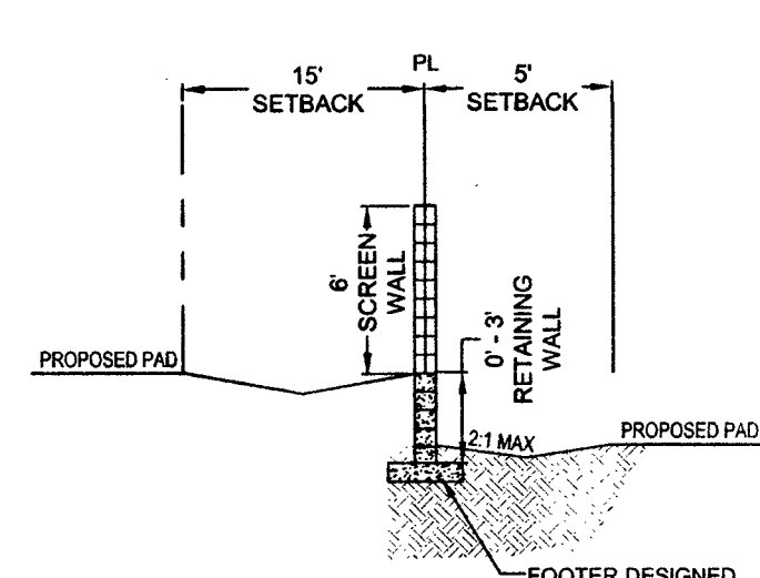
SECTION 'F' NTS REAR YARD TO SIDE YARD
