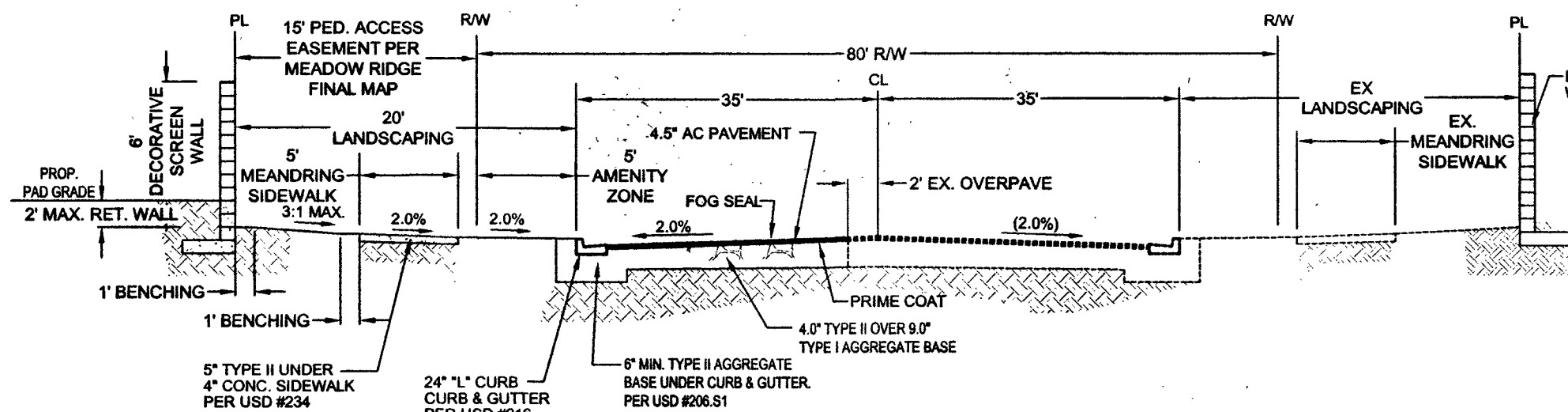
SECTION 'A' NTS 80' R/W HORSE DRIVE (PUBLIC)
