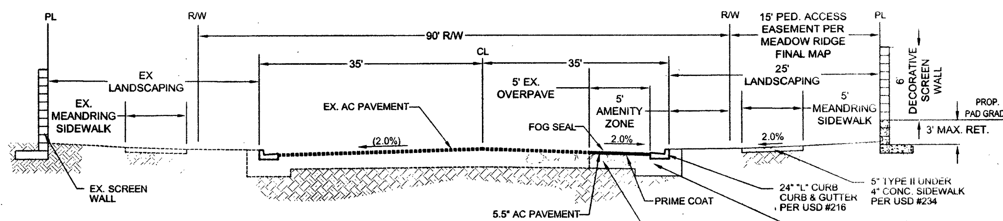
SECTION 'B' NTS 90' R/W JONES DRIVE (PUBLIC)
