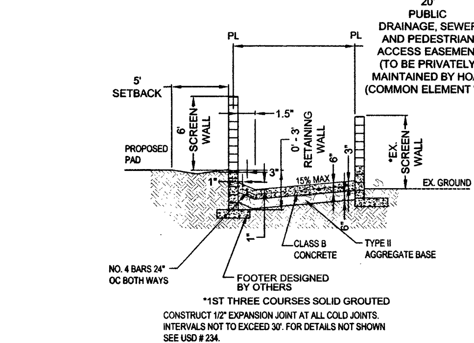
SECTION 'J' NTS 20' EASEMENT
