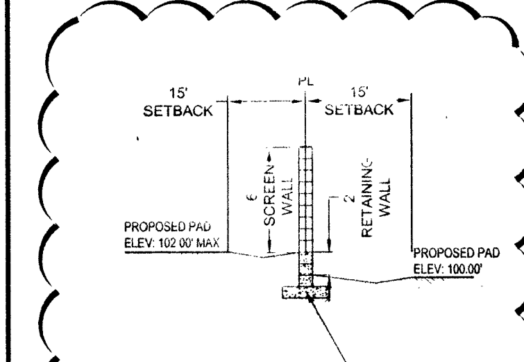
SECTION 'G' NTS REAR YARD TO REAR YARD
