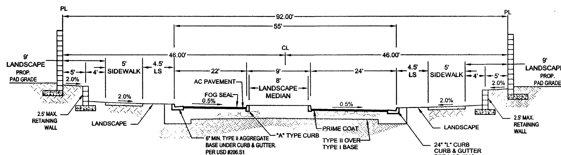
SECTION 'D' NTS MEADOW ROSE (ENTRY) (PRIVATE)
