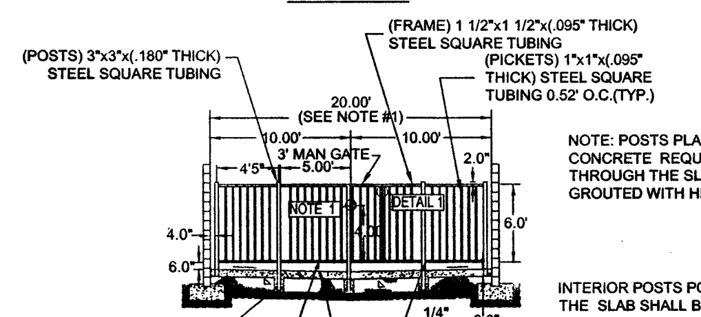
DETAIL 'M' NTS CLV FENCE DETAIL - MODIFIED (STD DWG 421B)
