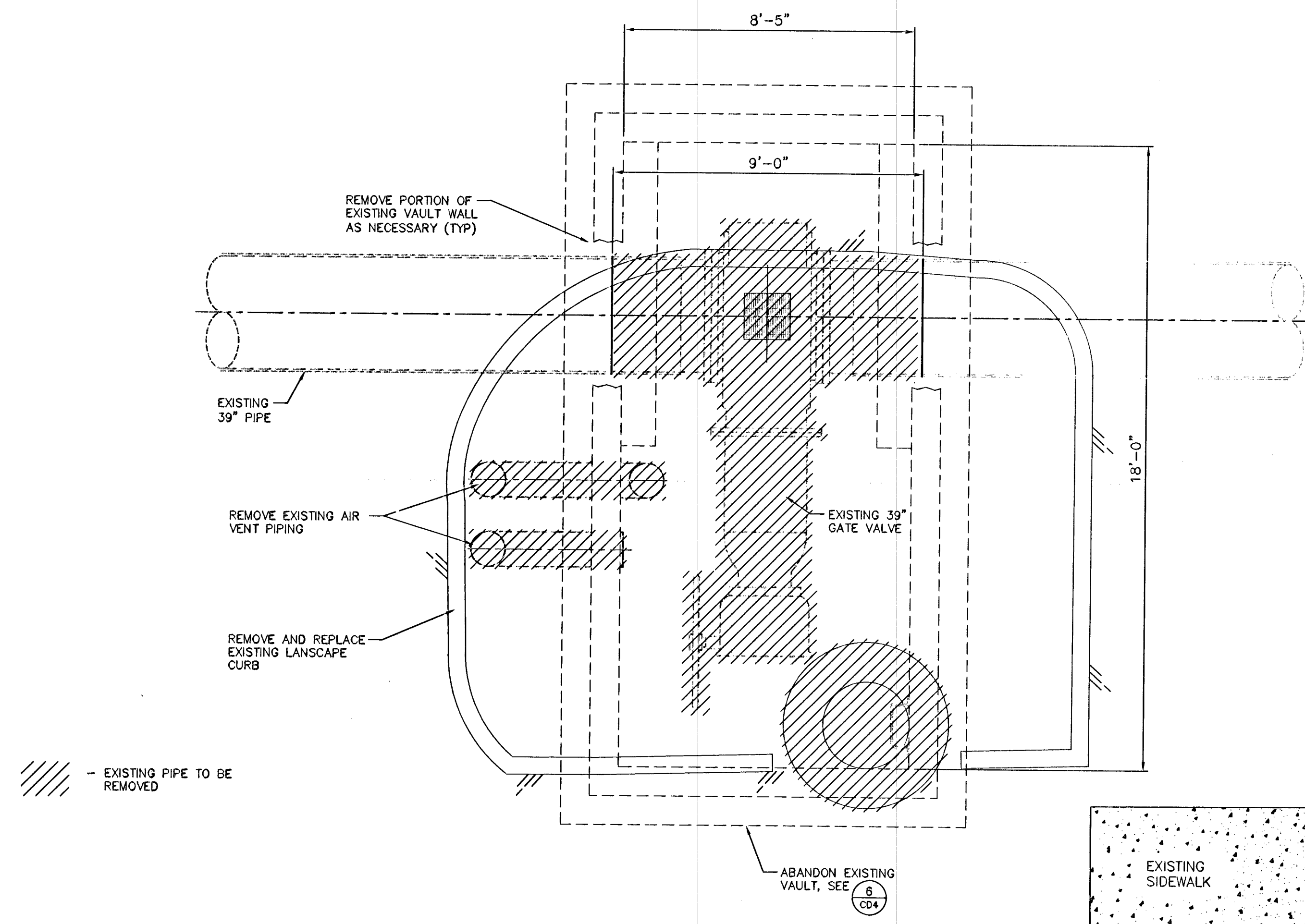
VAULT #834419 DEMOLITION PLAN
