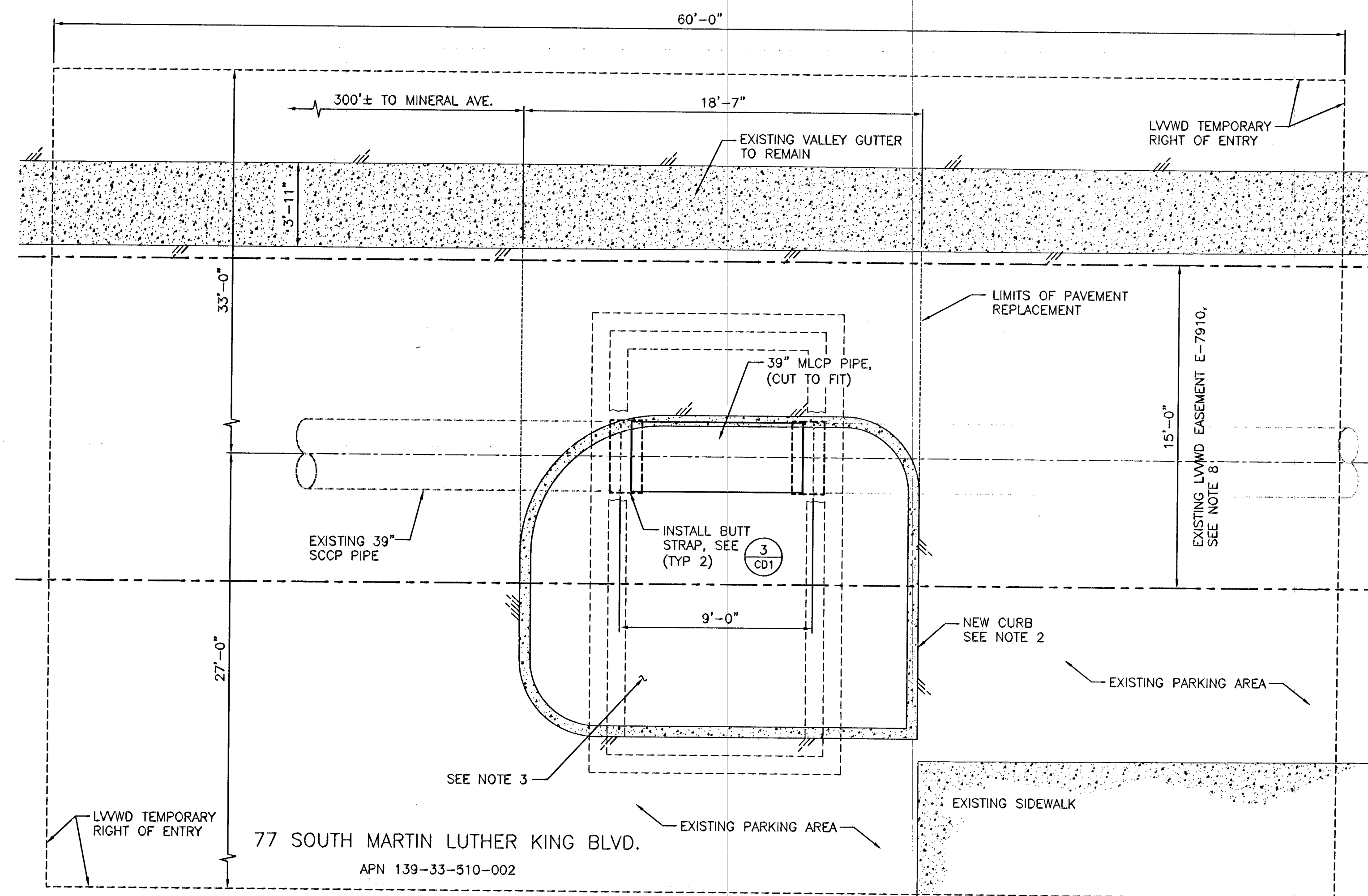
VAULT #834419 PIPE INSTALLATION PLAN
