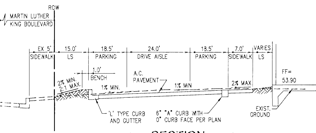
SECTION B NO SCALE
