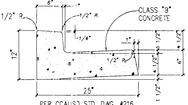
"L" CURB DETAIL NO SCALE
