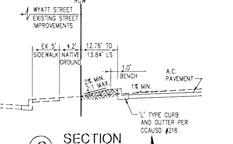
SECTION G NO SCALE
