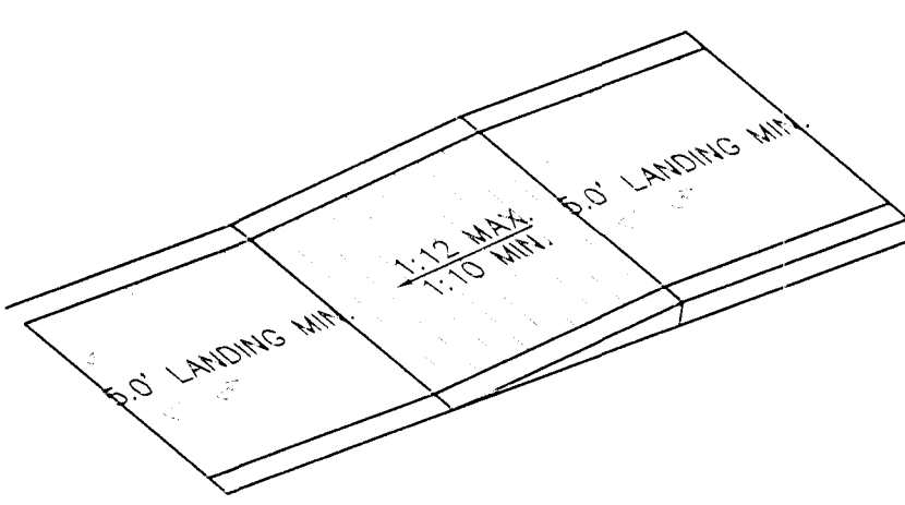
SIDEWALK RAMP DETAIL NO SCALE
