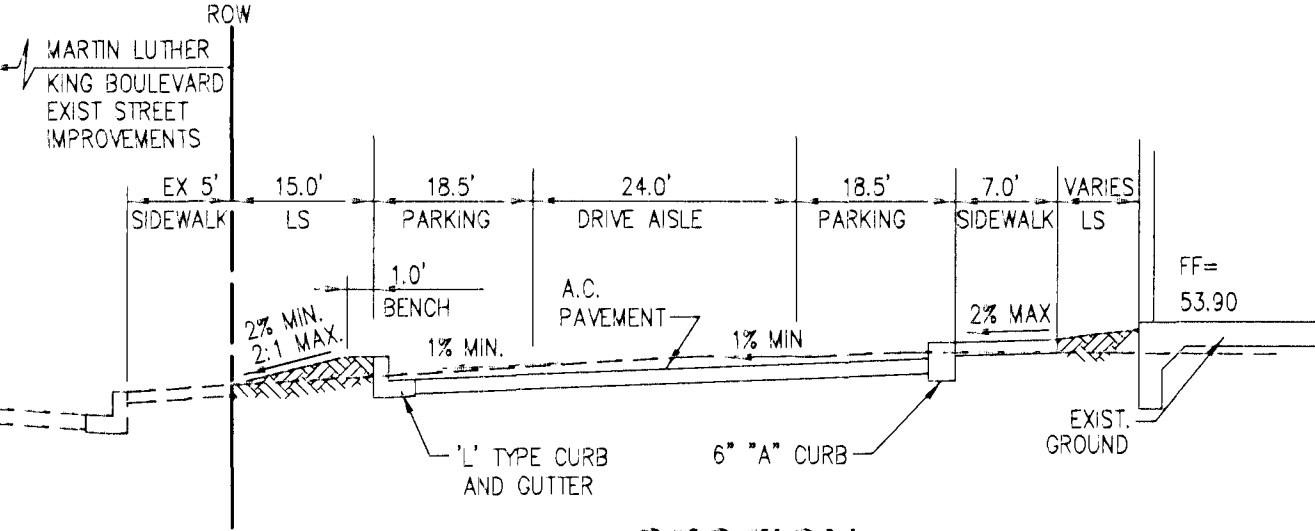
SECTION A NO SCALE
