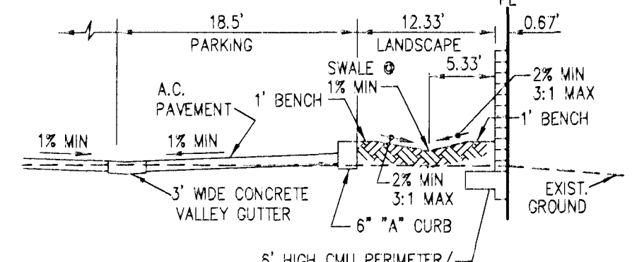
SECTION F NO SCALE
