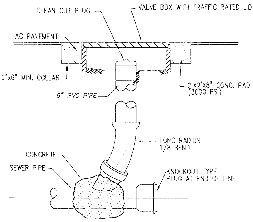
TRAFFIC RATED CLEANOUT NO SCALE
