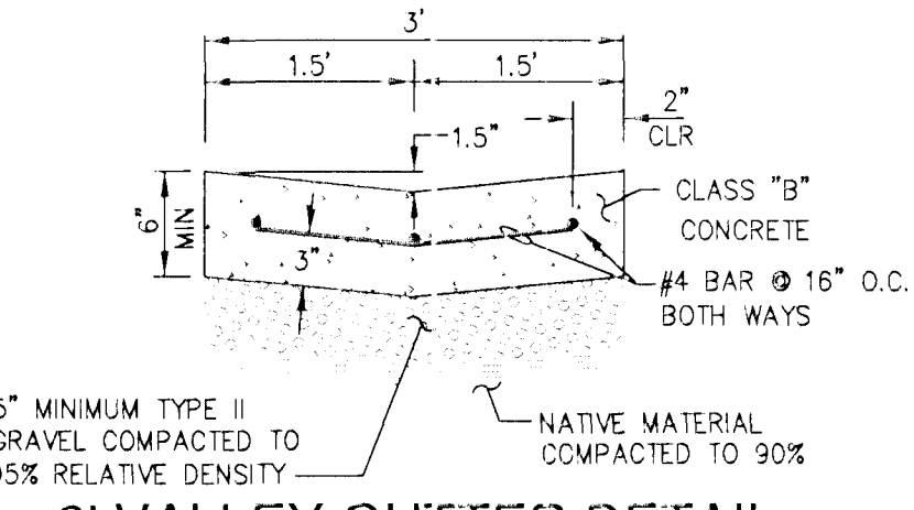
3' VALLEY GUTTER DETAIL NO SCALE
