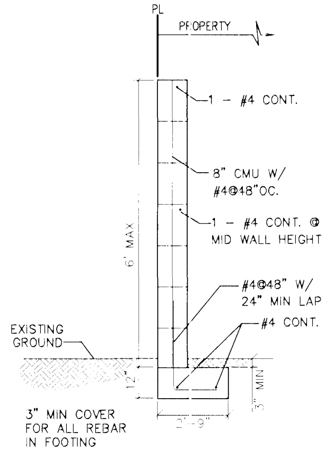
6' PERIMETER WALL NO SCALE
