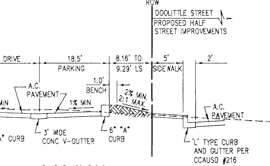
SECTION H NO SCALE
