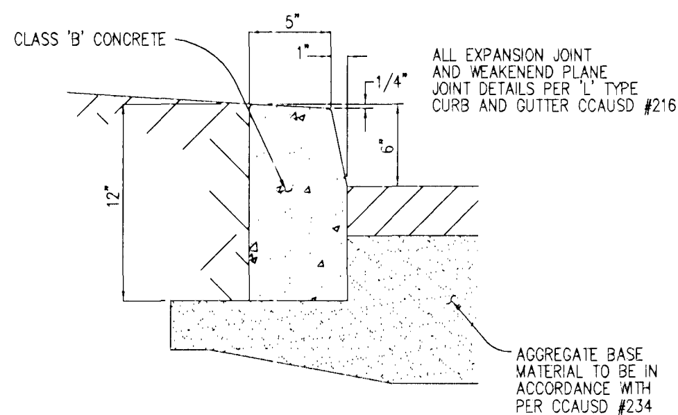
"A" CURB DETAIL NO SCALE
