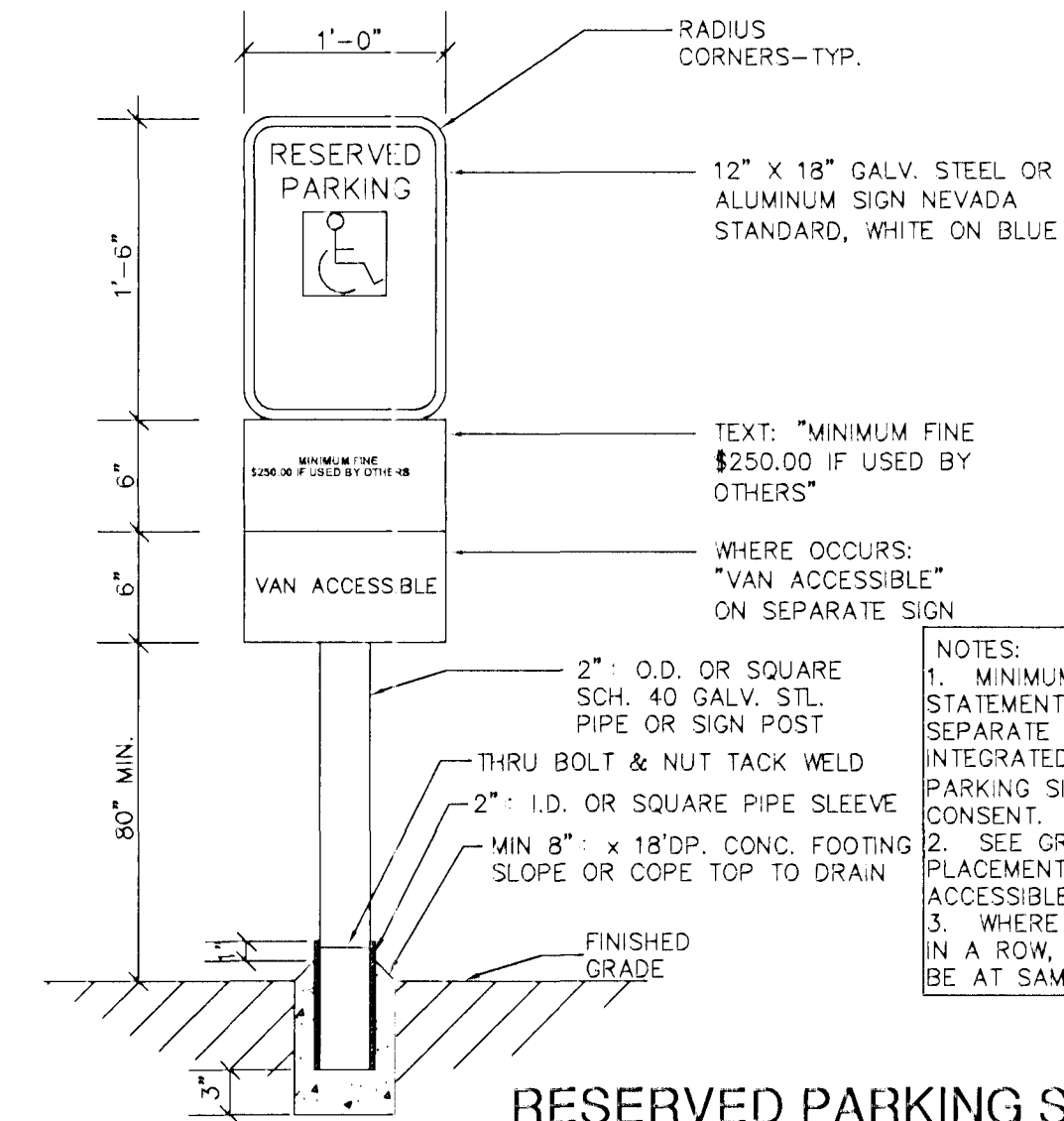
RESERVED PARKING SIGN NO SCALE
