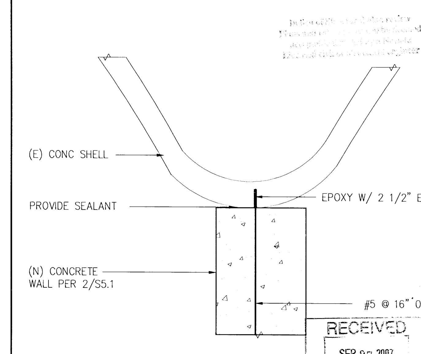
4 DETAIL 3/4"=1'-0"
