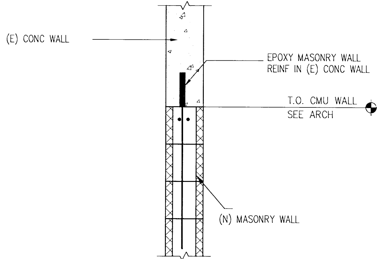
9 WALL DETAIL 1"=1'-0"
