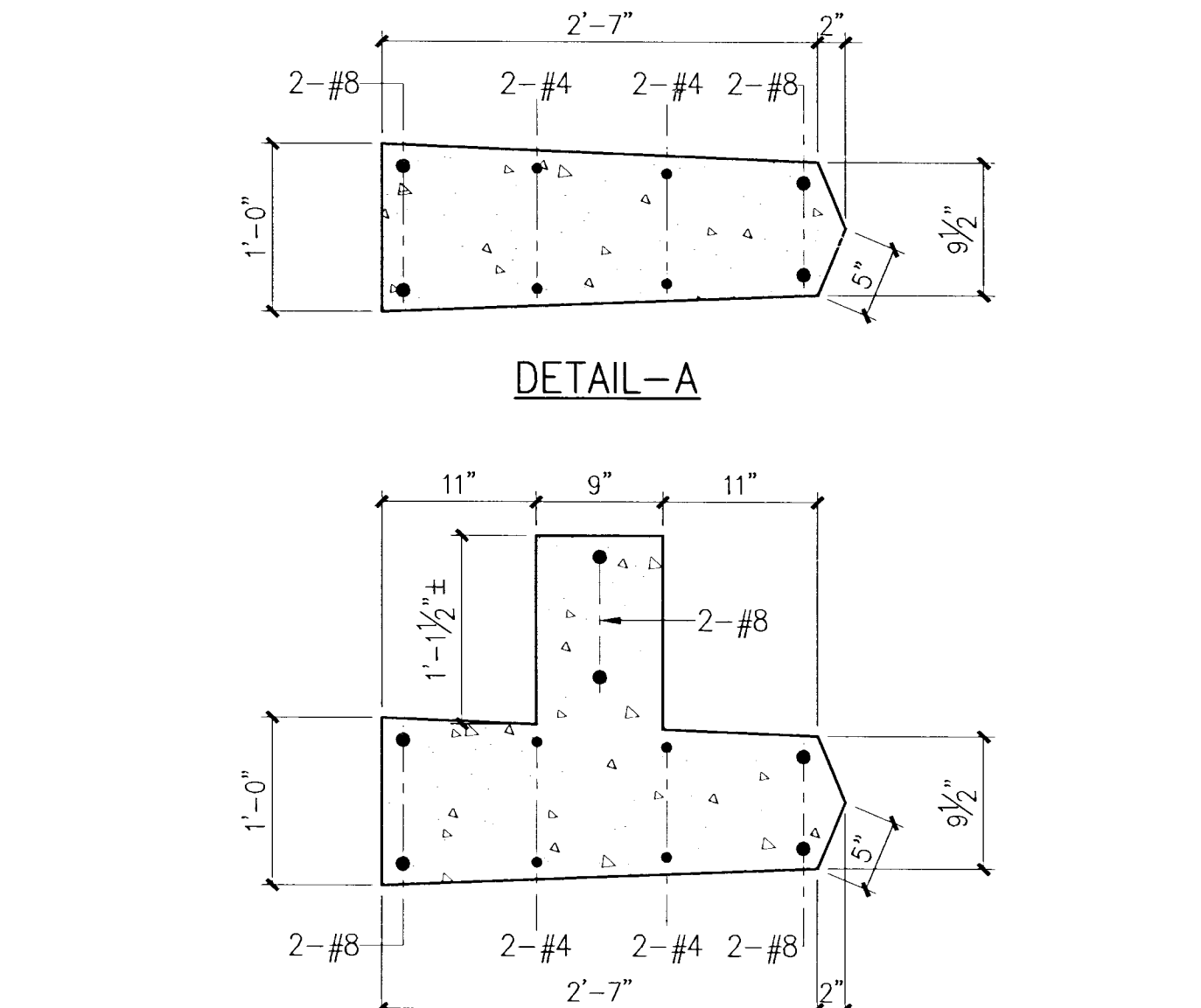
8 DETAIL 1"=1'-0"
