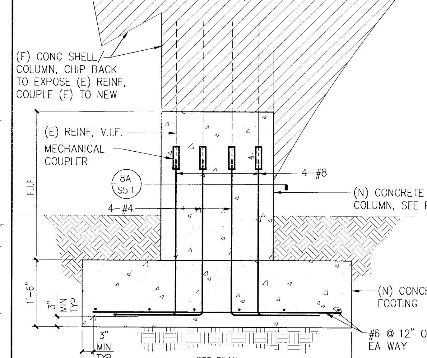
3 DETAIL 3/4"=1'-0"
