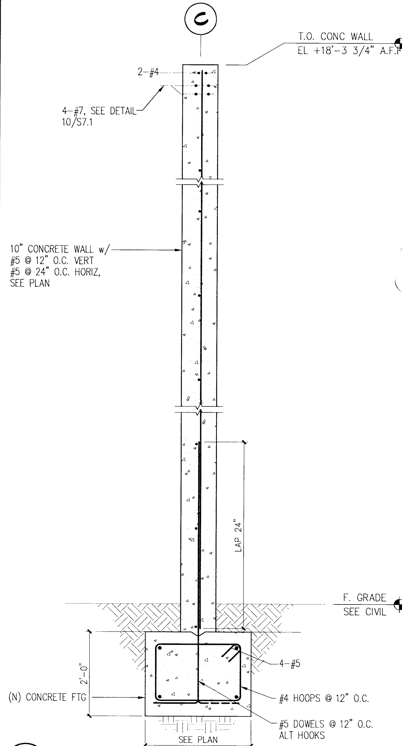
6 WALL SECTION 3/4"=1'-0"
