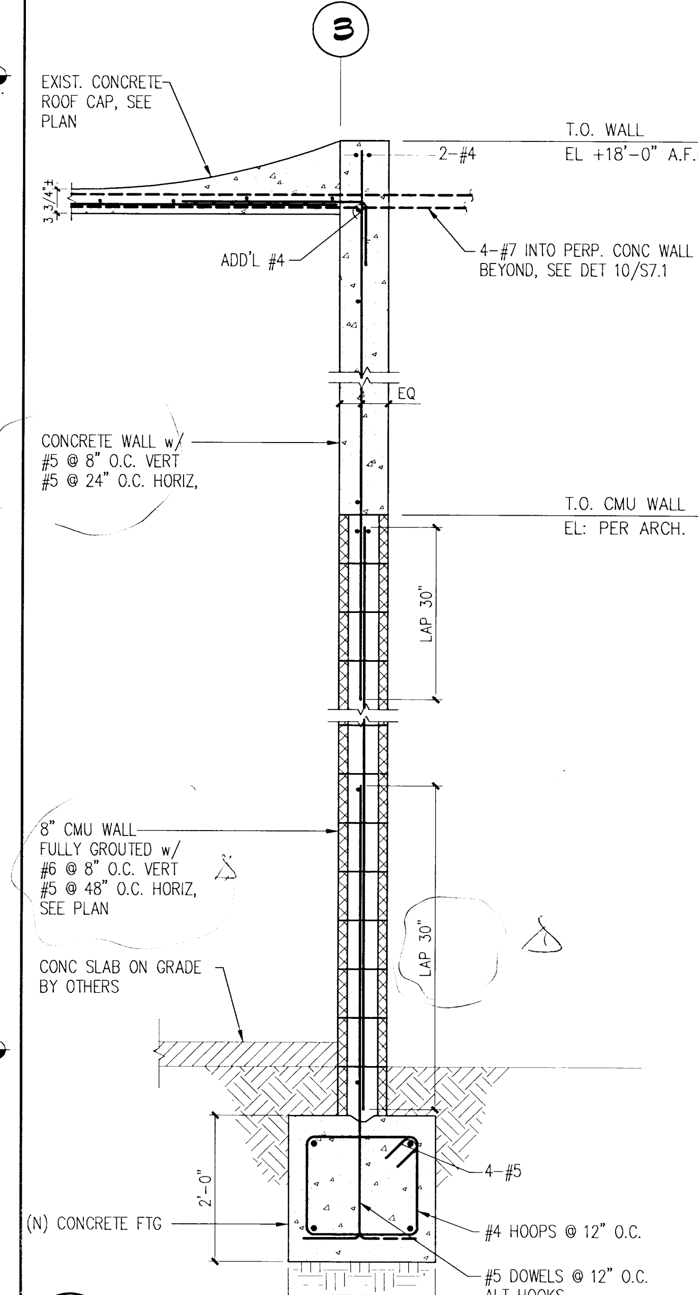
2 WALL SECTION 3/4"=1'-0"
