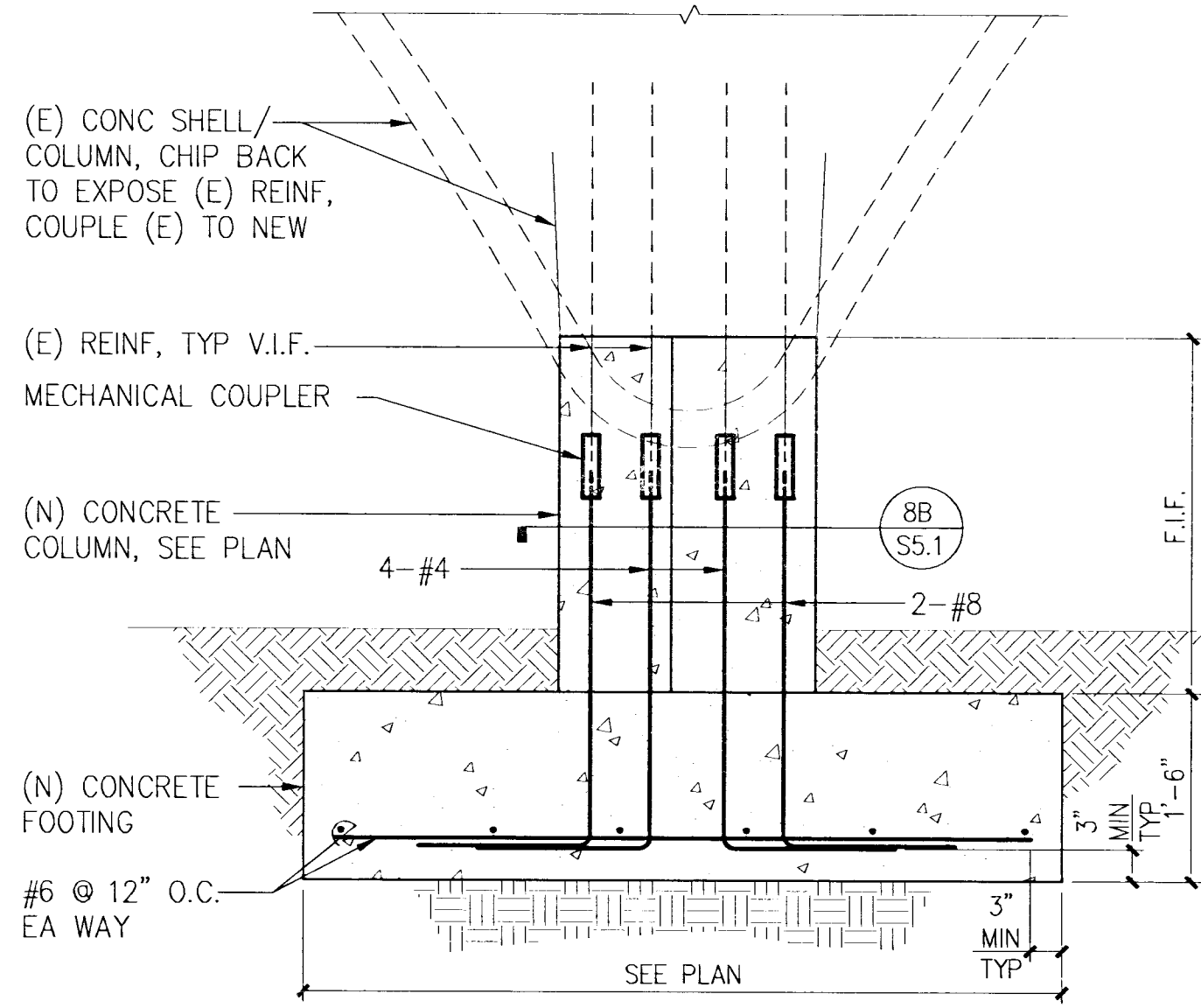
7 DETAIL 3/4"=1'-0"
