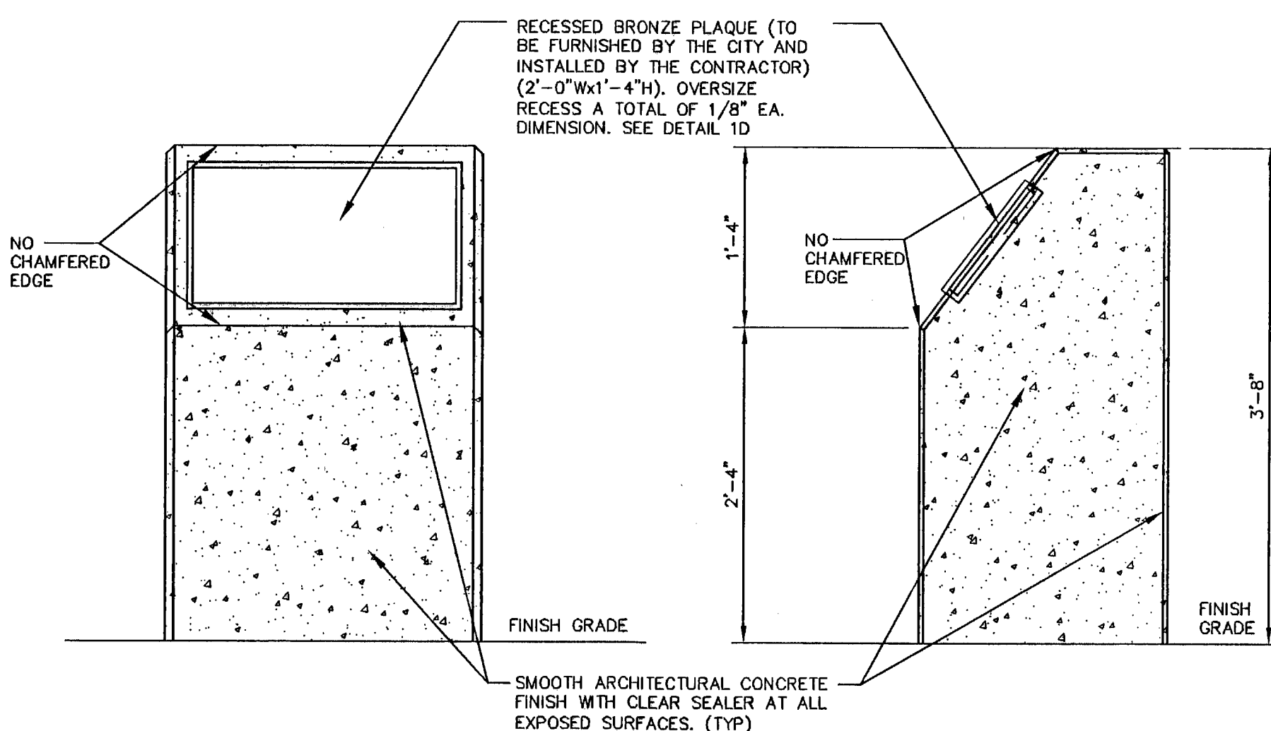
ELEVATIONS - CONCRETE MONUMENT FOR BRONZE PLAQUE N.T.S.
