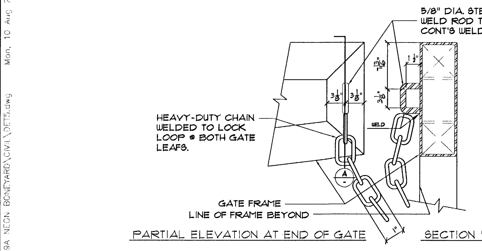
VEHICLE GATE CHAIN LOCK LOOP N.T.S.
