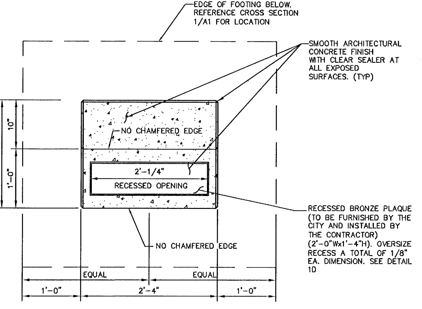
TOP VIEW - CONCRETE MONUMENT FOR BRONZE PLAQUE N.T.S.
