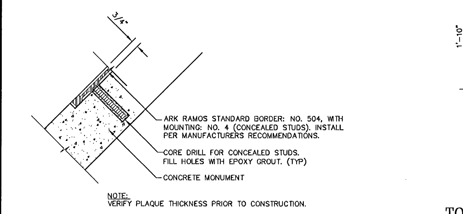
DETAIL FOR BRONZE PLAQUE N.T.S.
