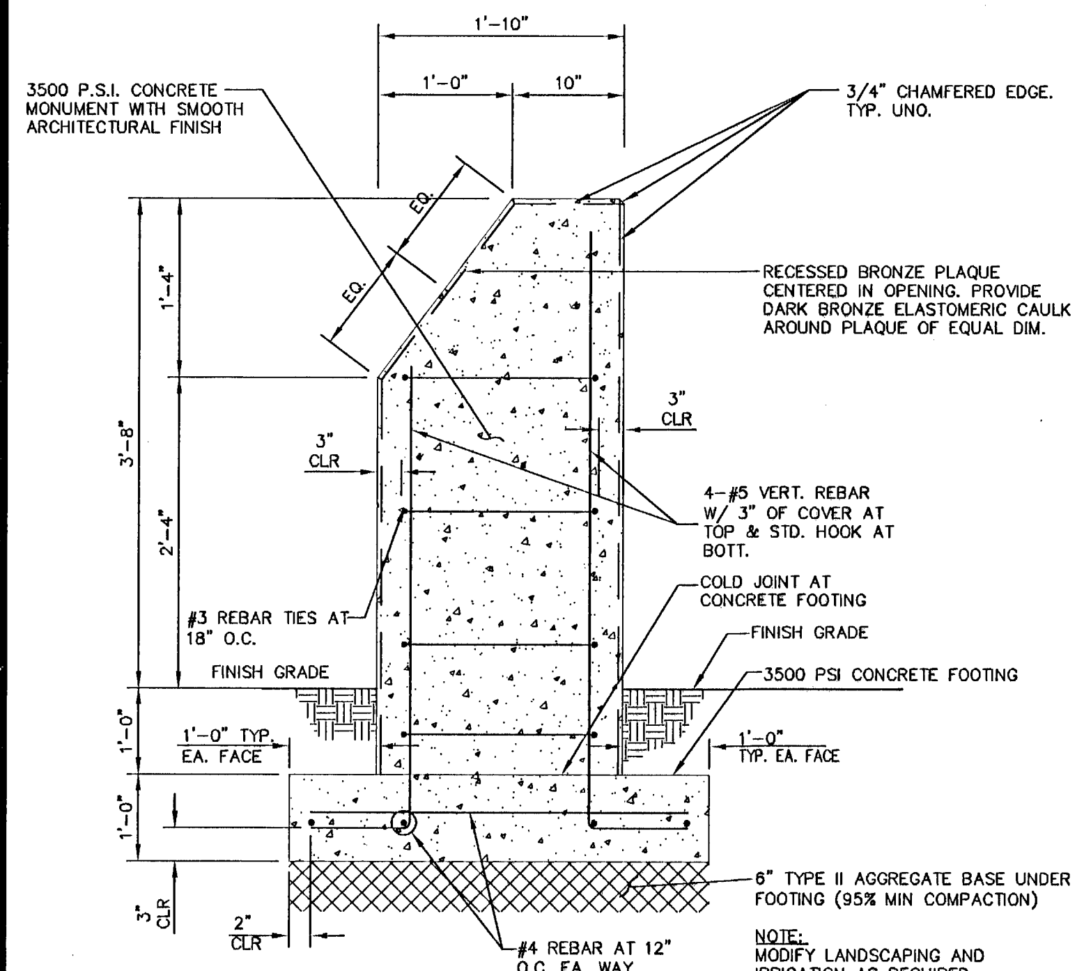
SECTION - CONCRETE MONUMENT FOR BRONZE PLAQUE N.T.S.
