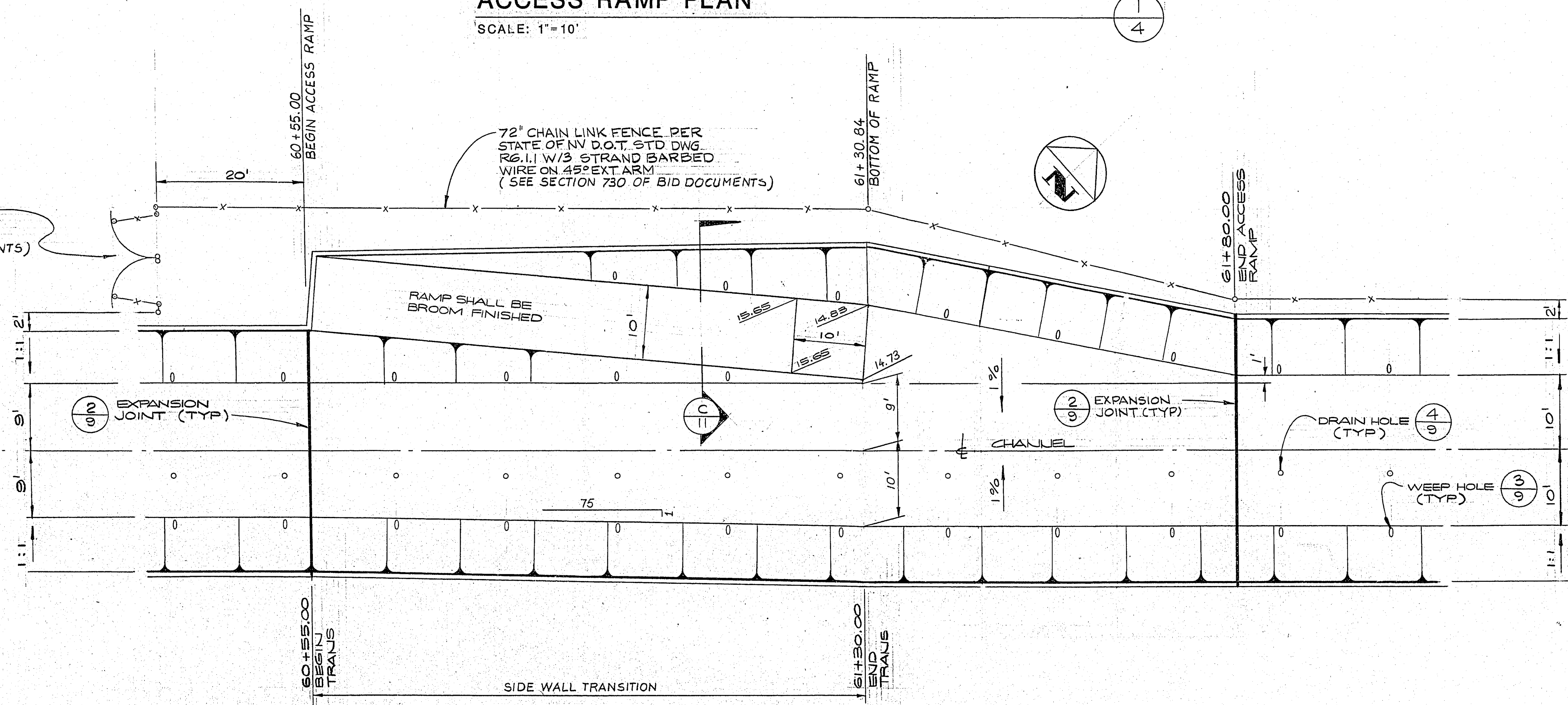
ACCESS RAMP PLAN
