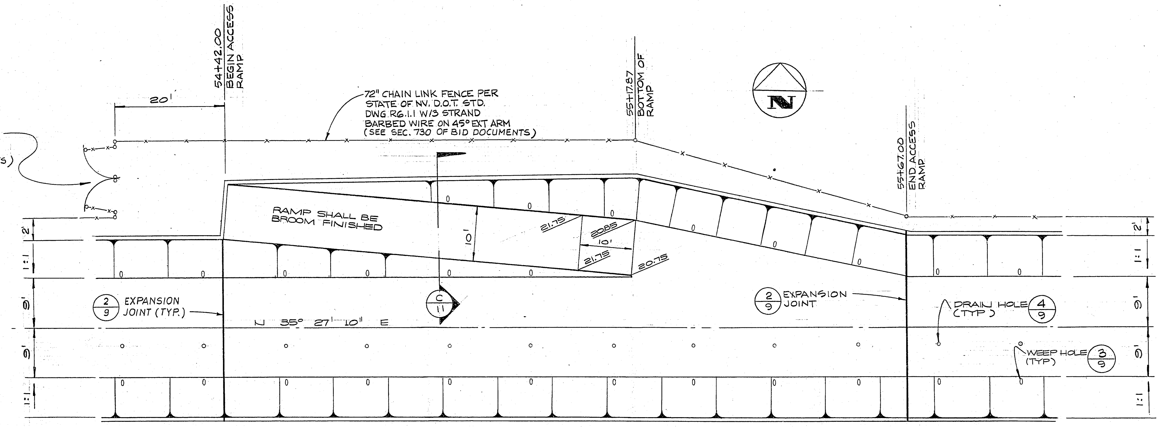
ACCESS RAMP PLAN
