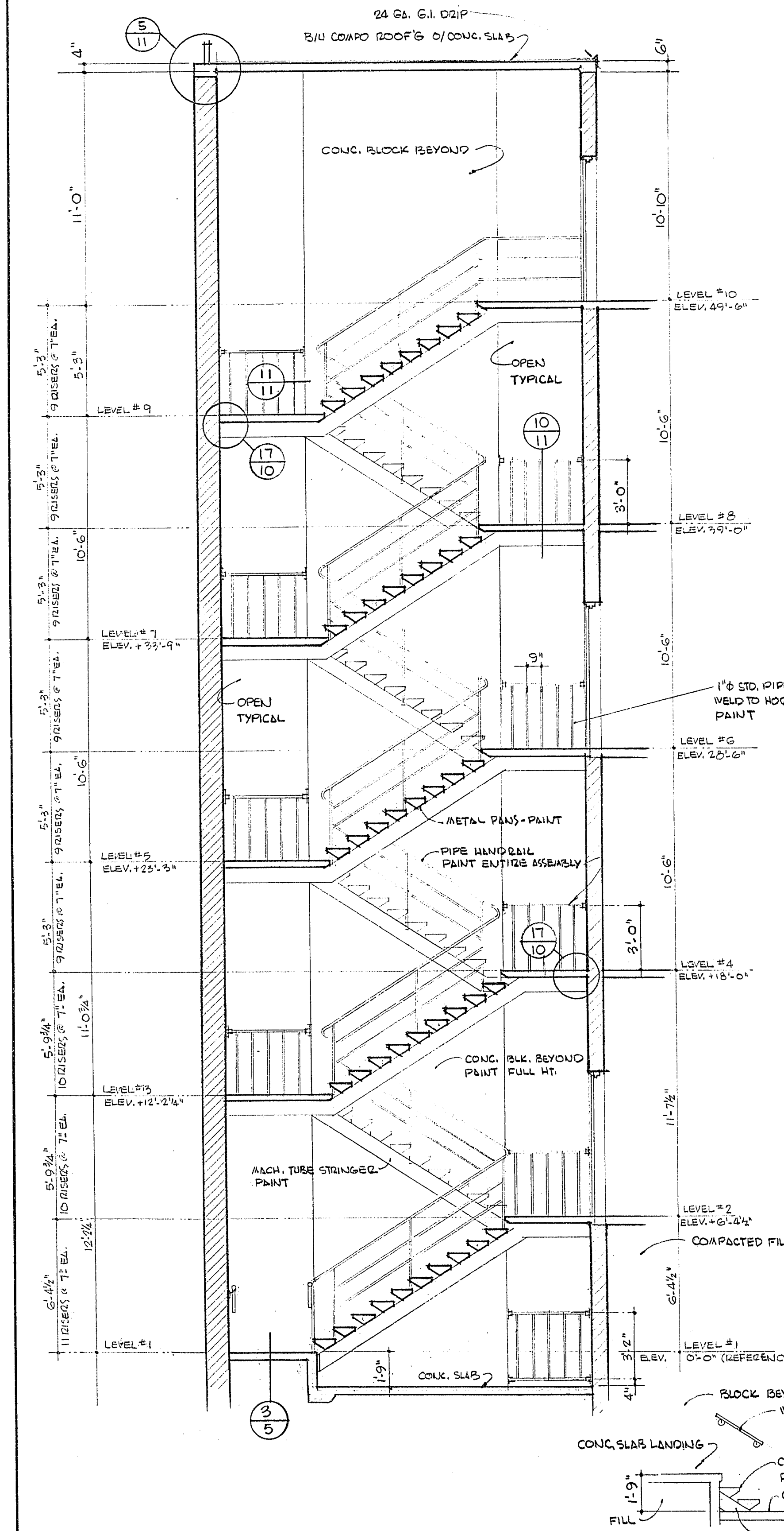
STAIRS NO 2 SECTION (2/5) SCALE - 1/4" = 1'-0"
