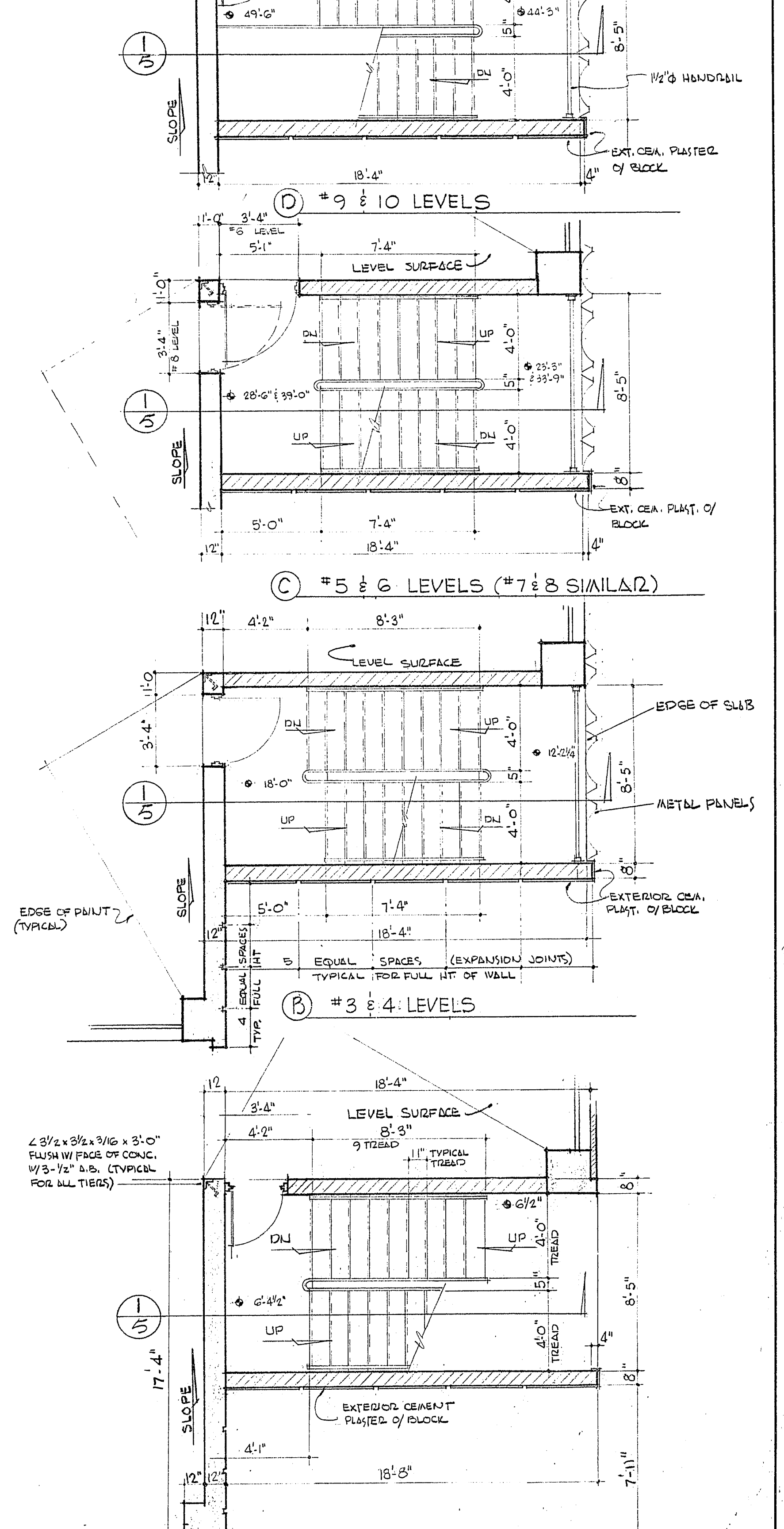
STAIRS NO 1 PLANS (A) #1 & 2 LEVELS SCALE - 1/4" = 1'-0"
