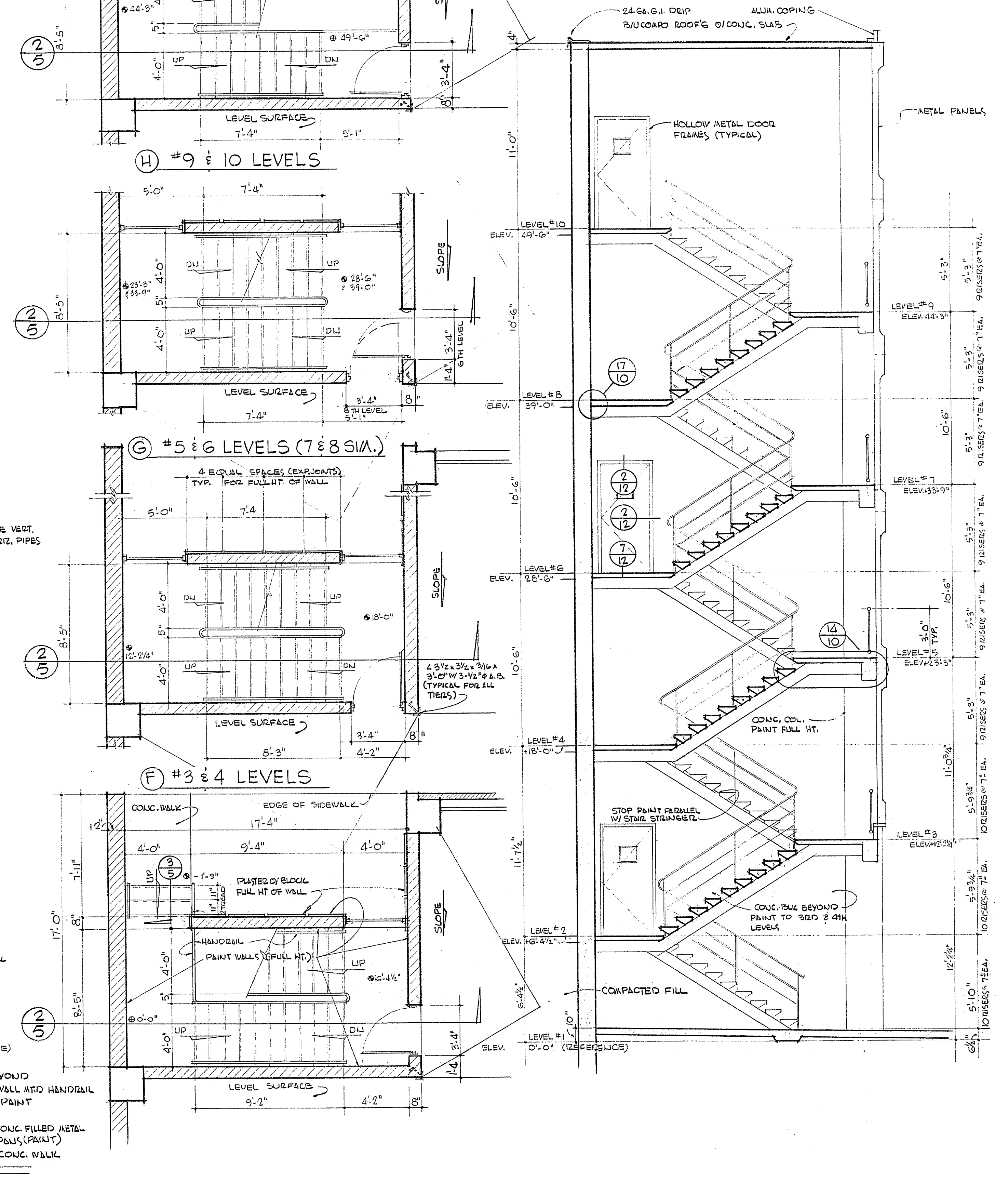
STAIRS NO 1 SECTION (1/5) SCALE - 1/4" = 1'-0"
