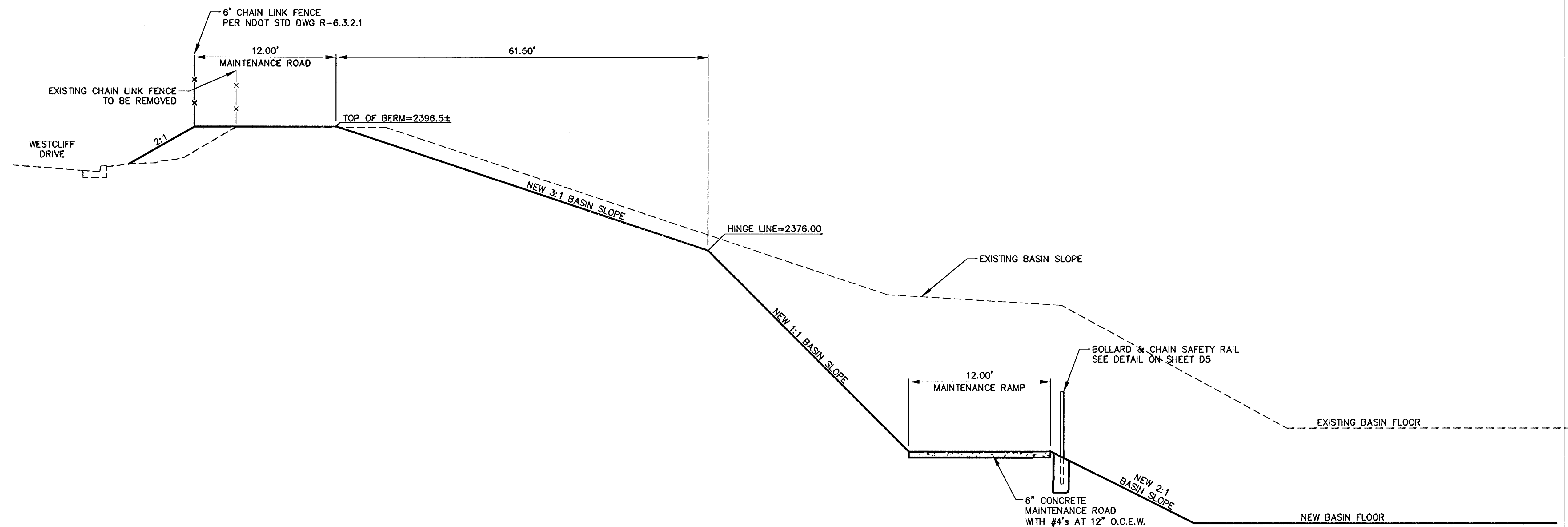
SECTION C-C EAST DETENTION BASIN SECTION ALONG WESTCLIFF DRIVE
