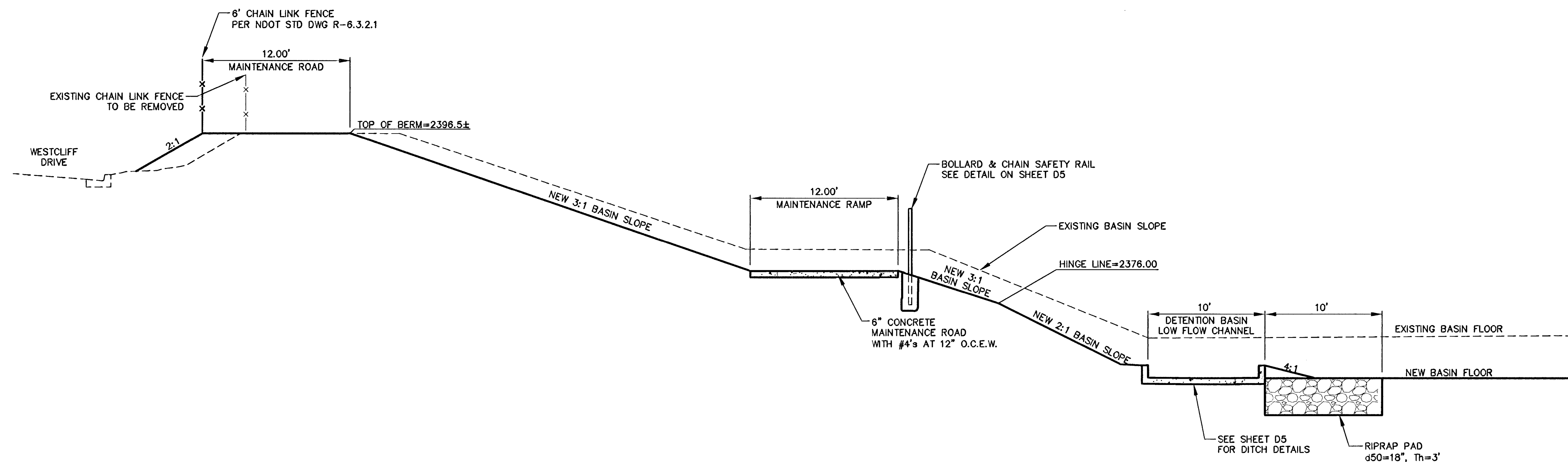
SECTION C-C EAST DETENTION BASIN SECTION ALONG WESTCLIFF DRIVE
