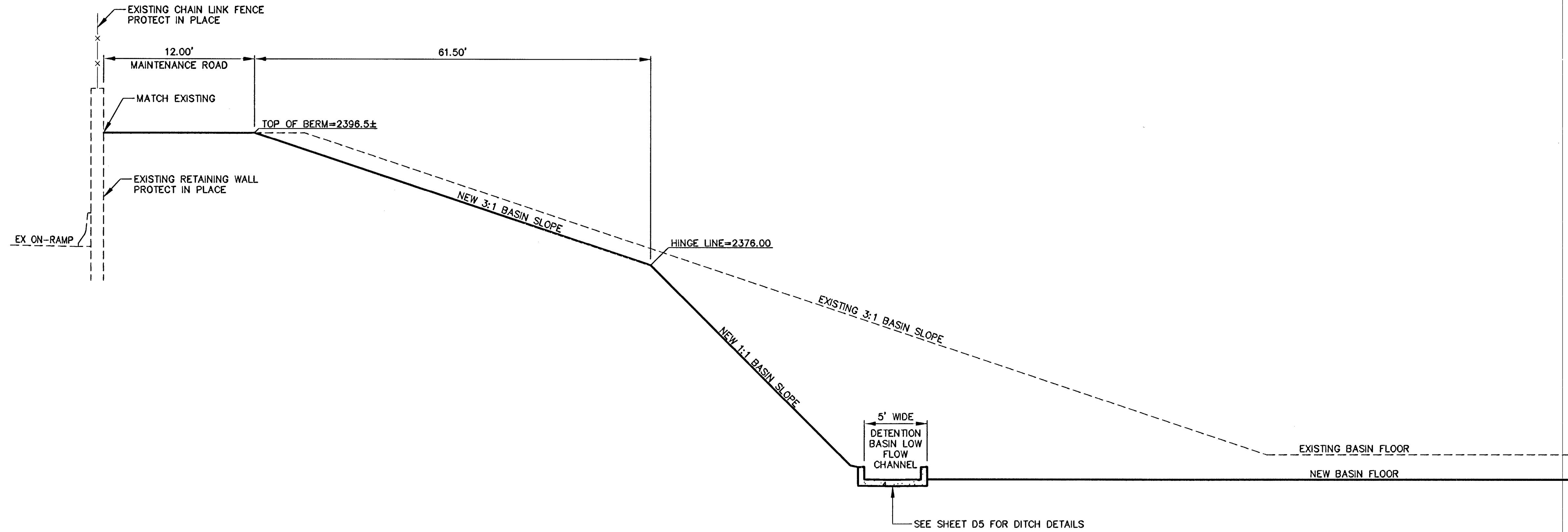
SECTION A-A EAST DETENTION BASIN SECTION ALONG EXISTING ON-RAMP
