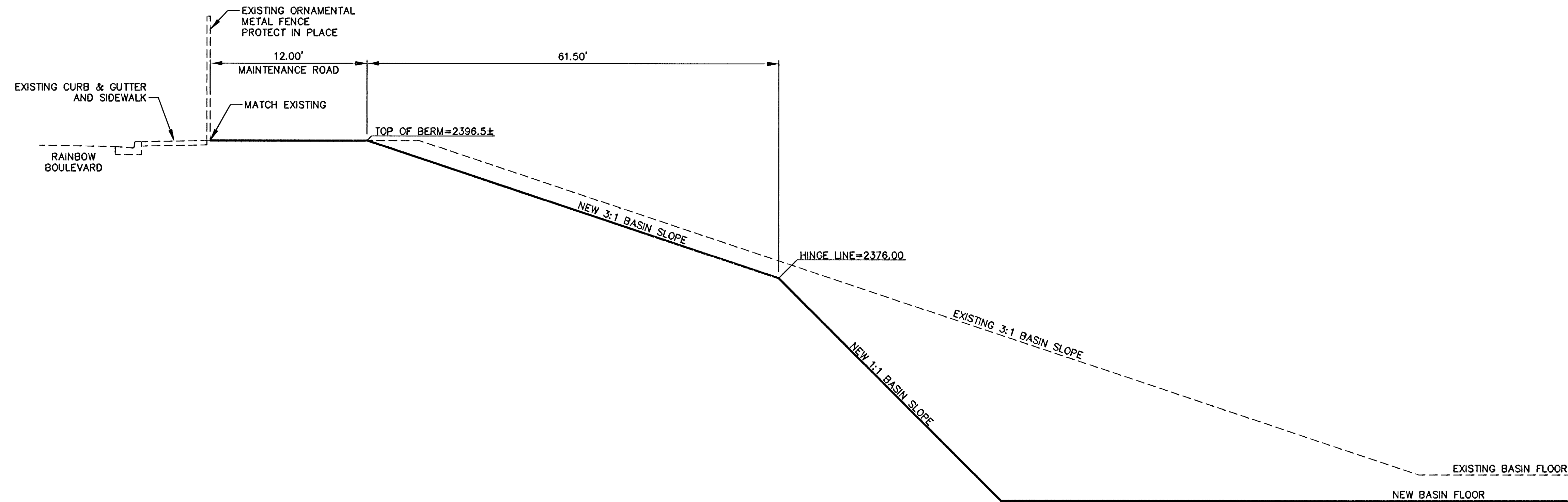
SECTION A-A EAST DETENTION BASIN SECTION ALONG EXISTING ON-RAMP
