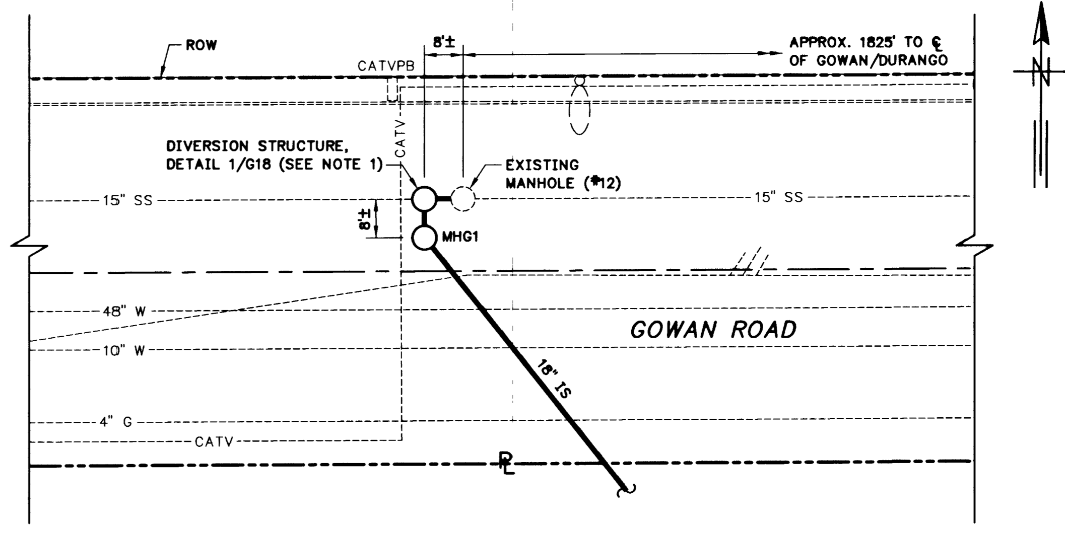
DETAIL 1/G10,G28 - DIVERSION STRUCTURE SCALE: 1" = 20'
