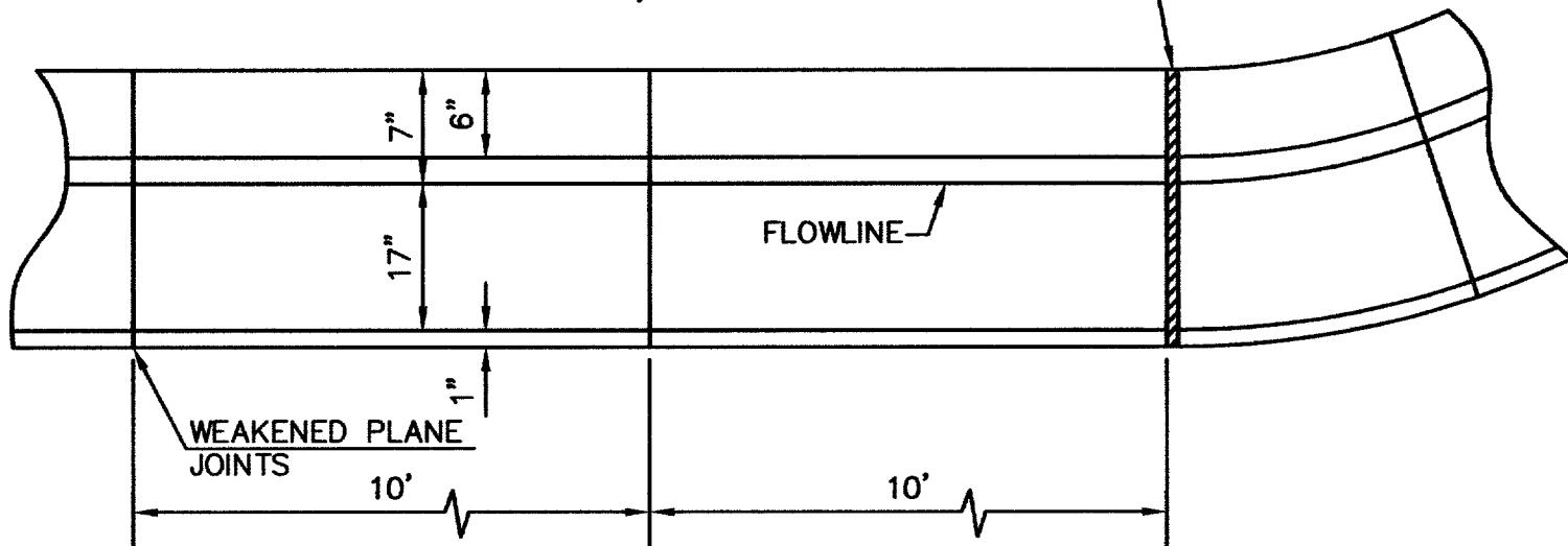
8' 'L' TYPE CURB & GUTTER
