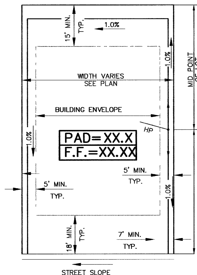
TYPICAL LOT GRADING FROM SIDE OF LOT
