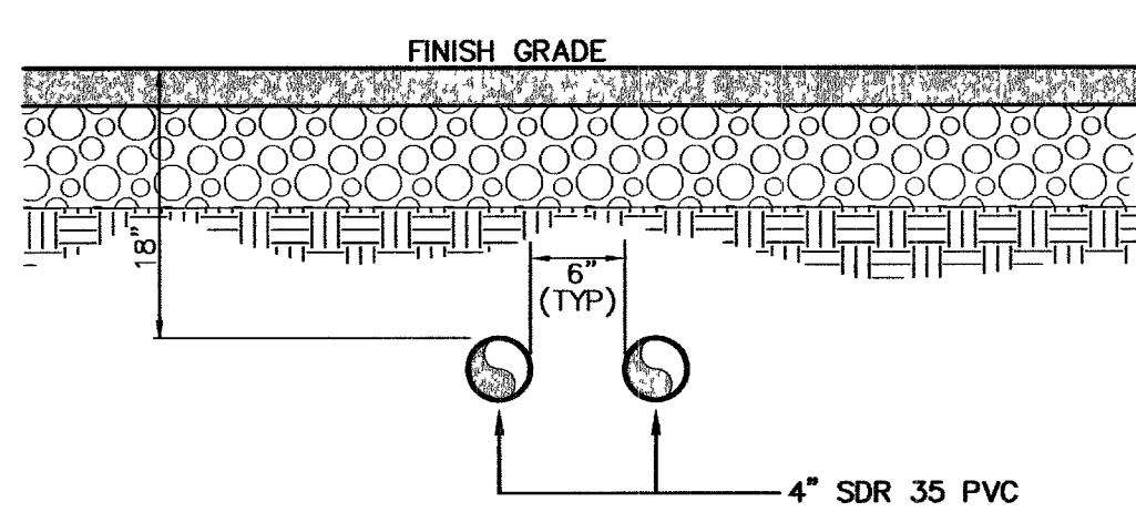
IRRIGATION SLEEVES - BANK "A"
