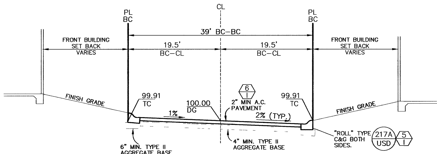
OFFSET CROWN SECTION
