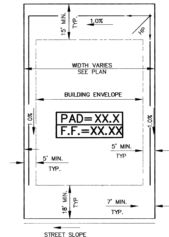
TYPICAL LOT GRADING
