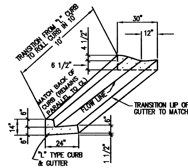
30' ROLL TYPE CURB & GUTTER TRANSITION TO 'L' TYPE CURB & GUTTER
