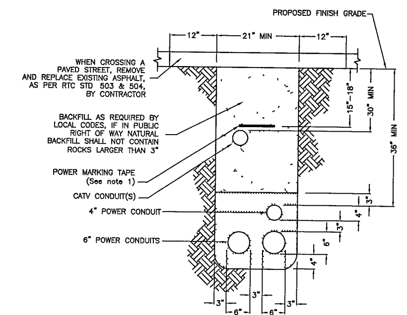
B TRENCH DETAIL STREET CROSSINGS (NOT TO SCALE)
