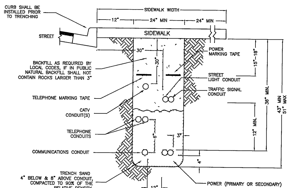
A SIDEWALK TRENCH DETAIL (NOT TO SCALE)
