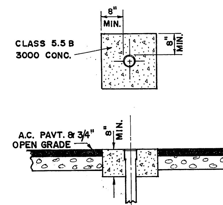
Valve Collar Detail
