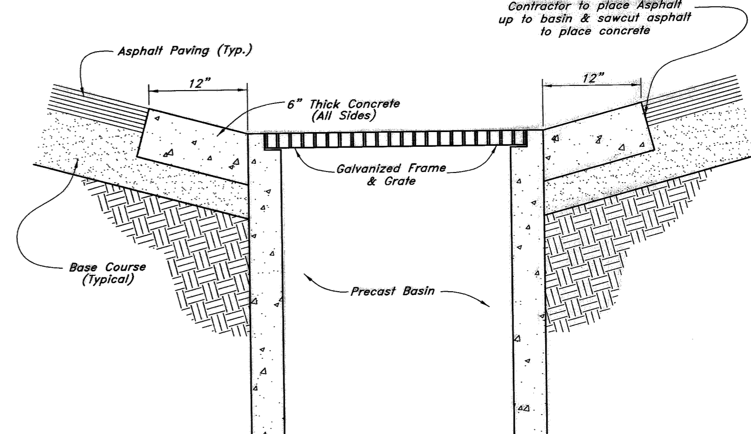
12 12" Concrete Collar Not to Scale
