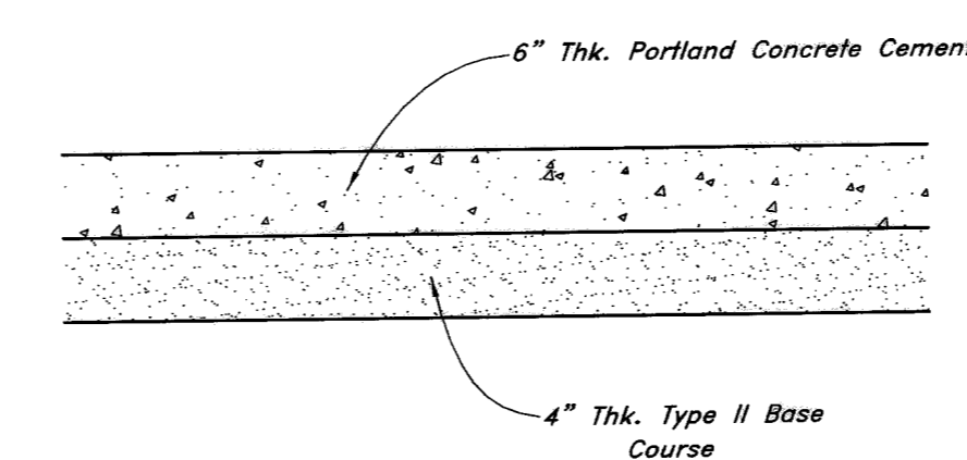
15 Concrete Pavement Detail Not to Scale
