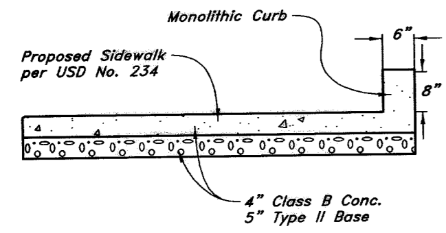
22 Flood Curb Detail Not to Scale
