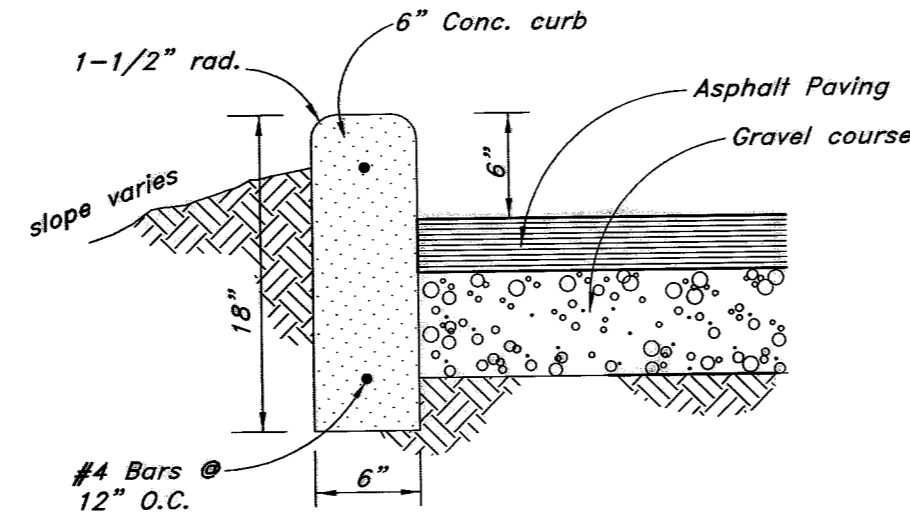
20 Typical Curb Wall Detail Not to Scale
