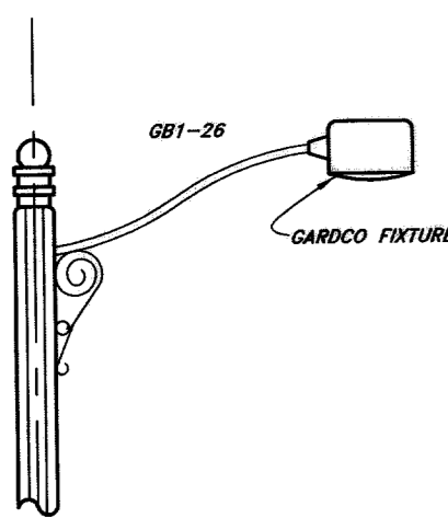
STREETLIGHT-SINGLE ARM
