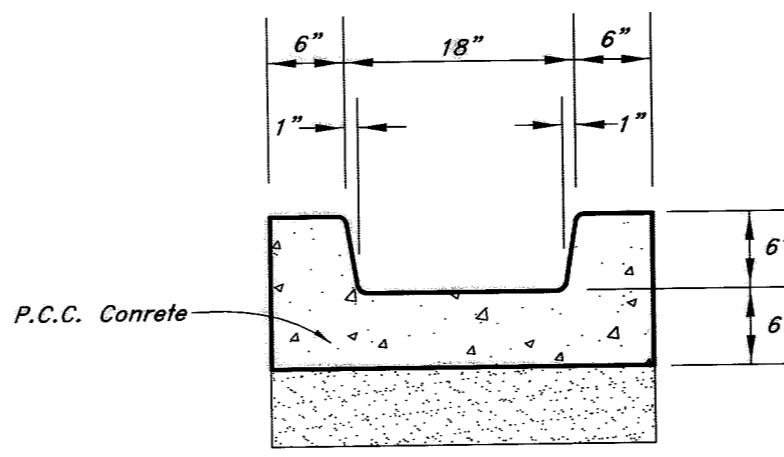
17 Drainage Channel Detail Not to Scale
