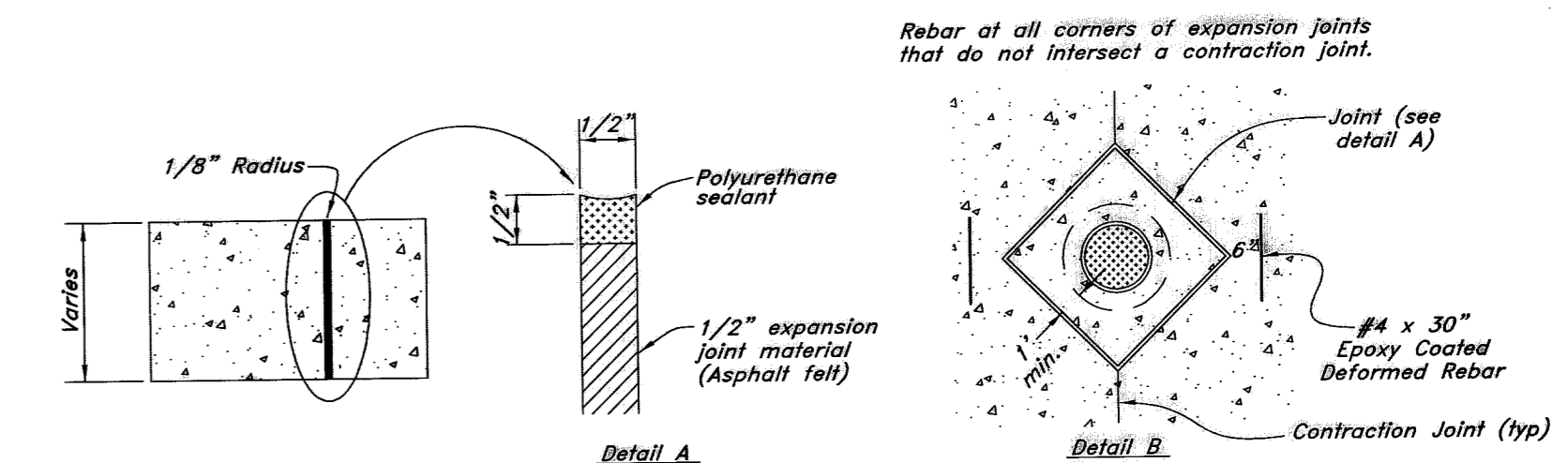
11 Expansion Joint Not to Scale
