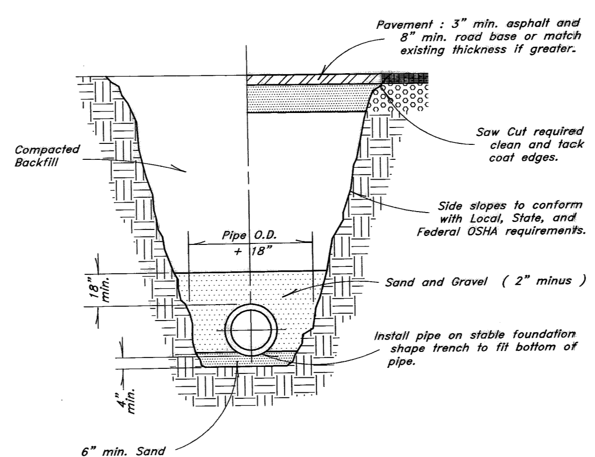
14 Typical Trench Detail Not to Scale
