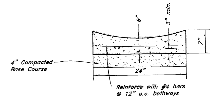
13 Typical Waterway Detail Not to Scale
