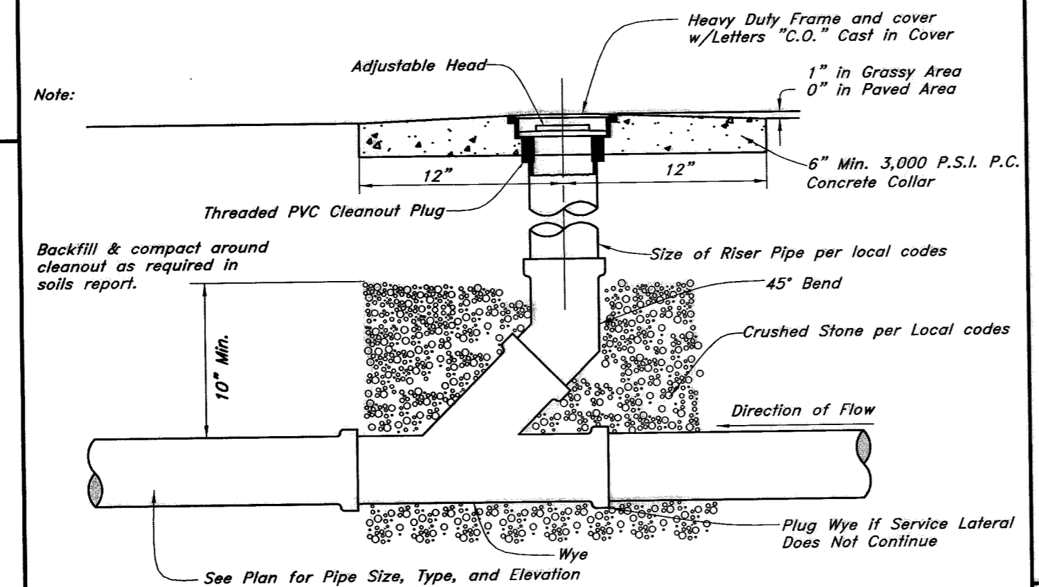
19 Cleanout Detail Not to Scale
