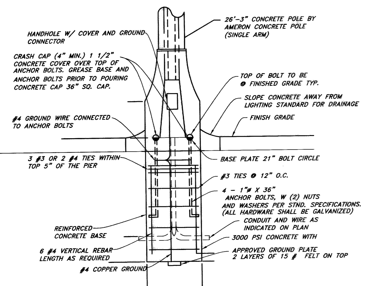
21 Street Light Pole Detail Not to Scale
