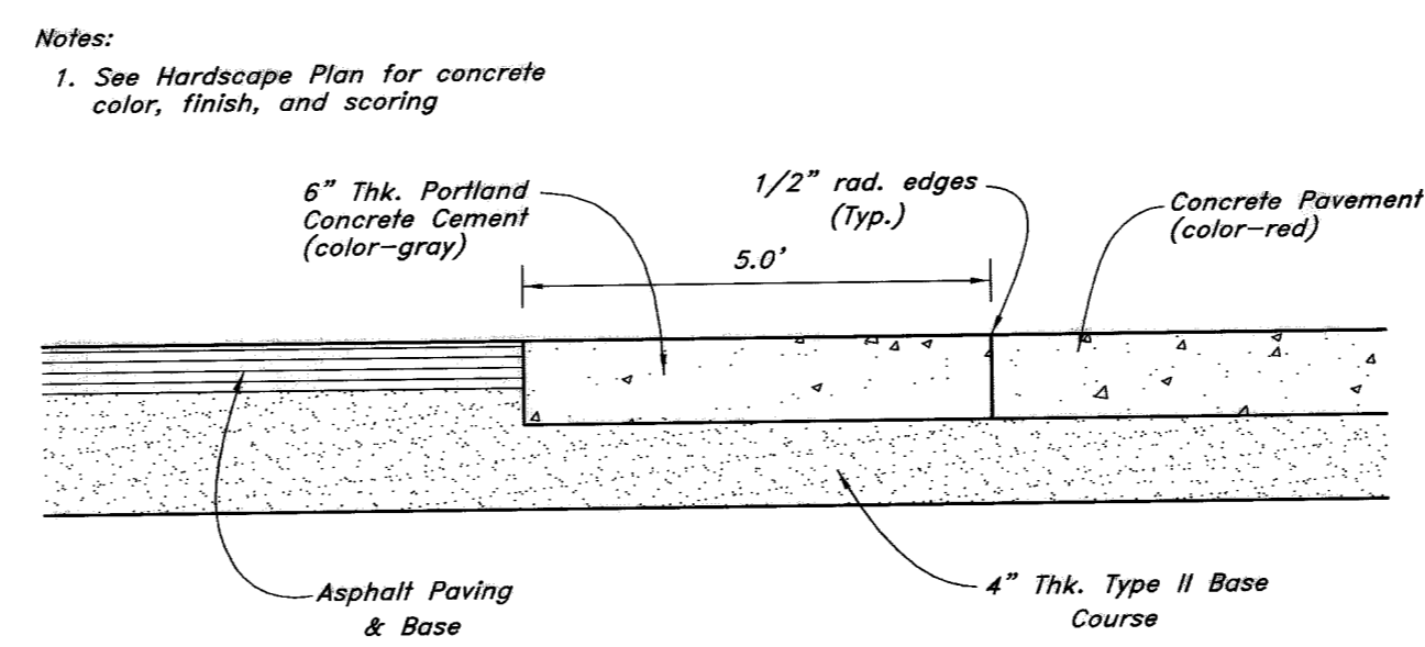
16 Concrete Pavement Band Not to Scale
