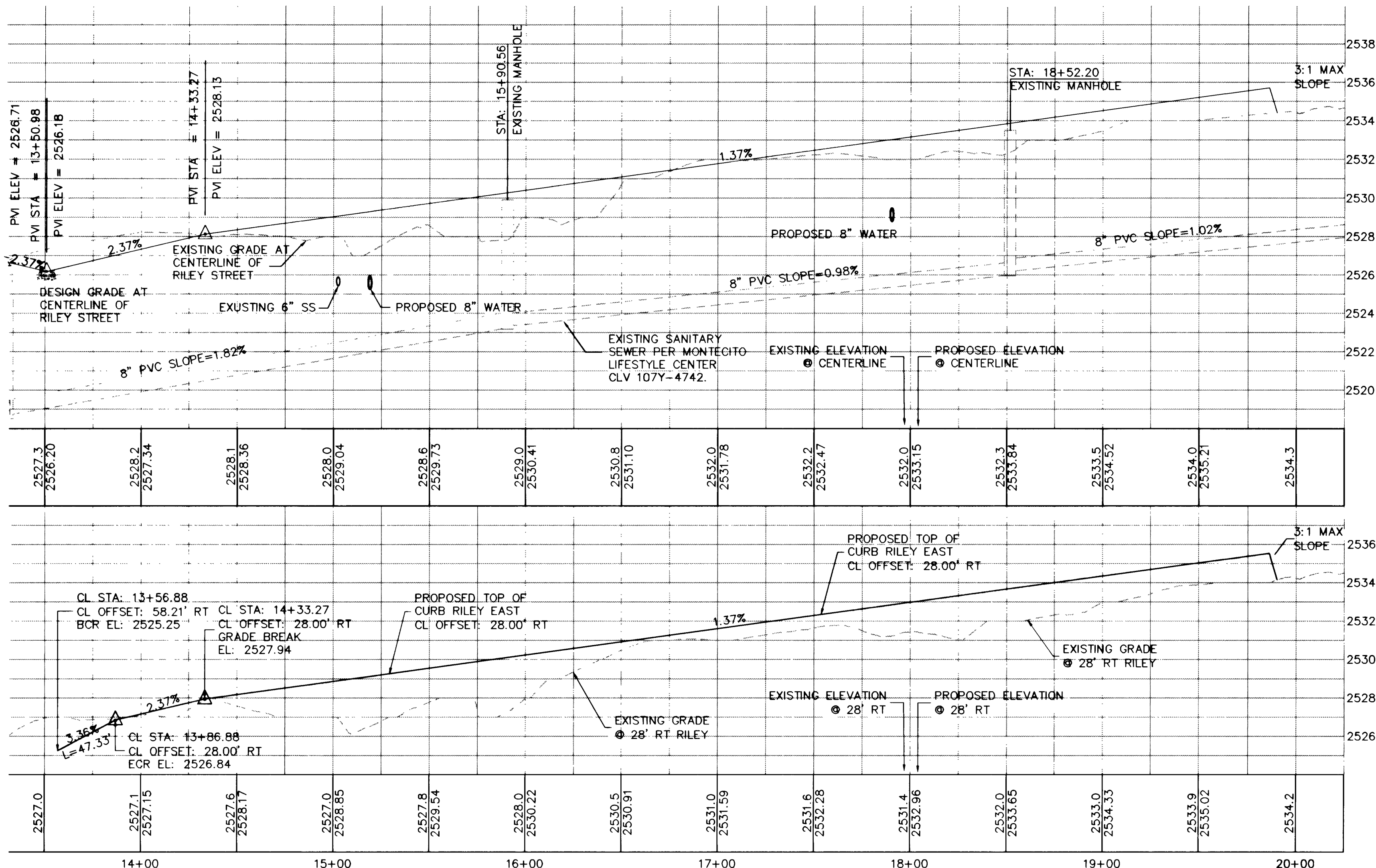
RILEY STREET PROFILE (PUBLIC) TOP-FINISHED GRADE CL RILEY, BOTTOM-TOP OF CURB RILEY EAST HORIZONTAL SCALE: 1"=40' VERTICAL SCALE: 1"=4'
