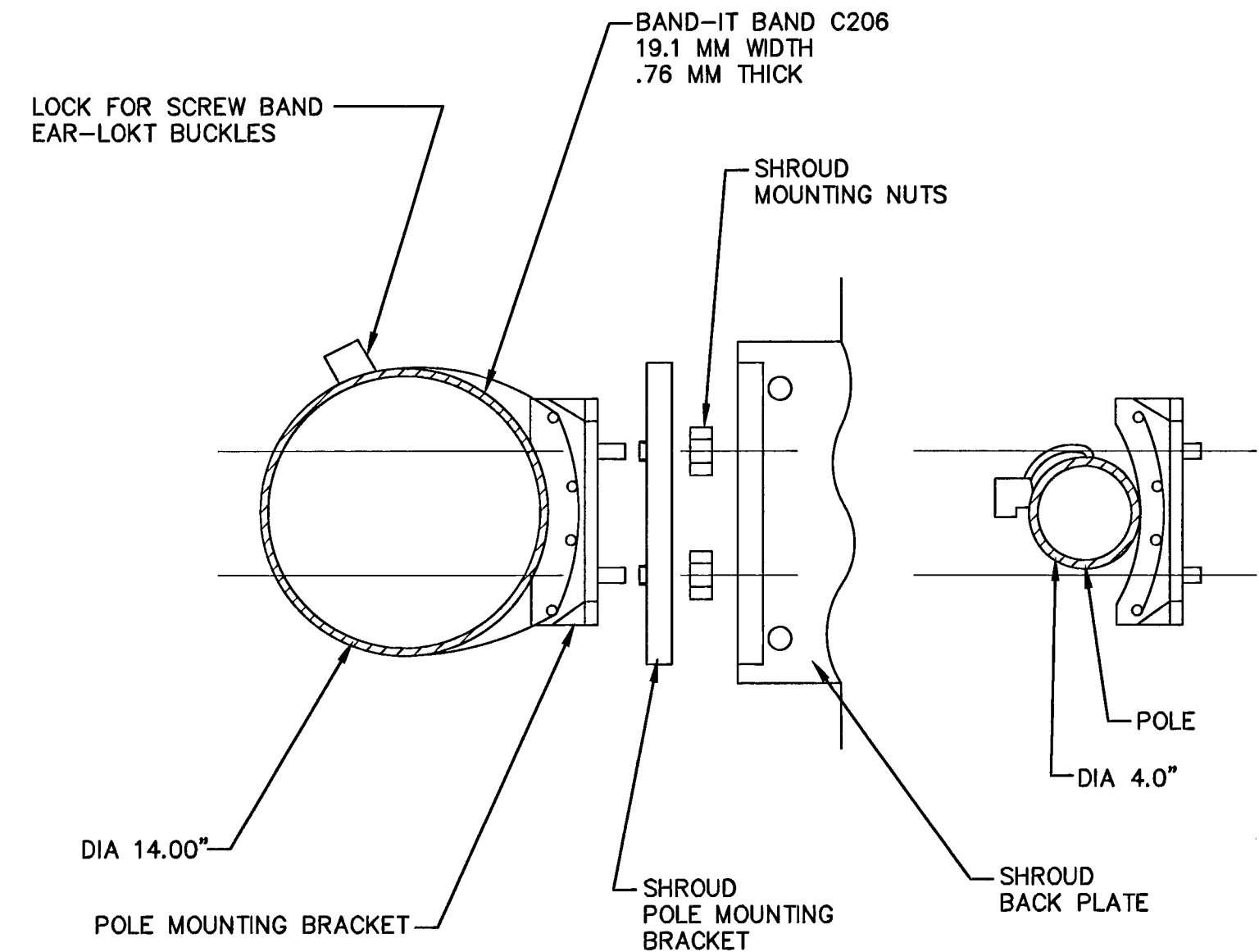
POLE MOUNTING
