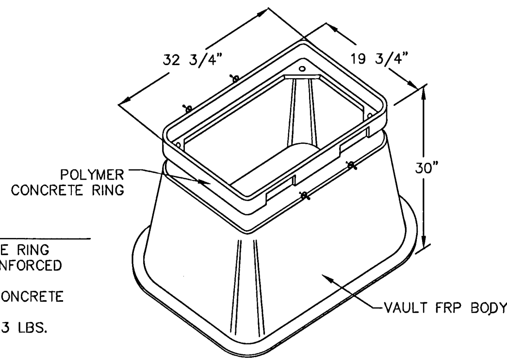
17' X 30' CONNECTOR MANHOLE
