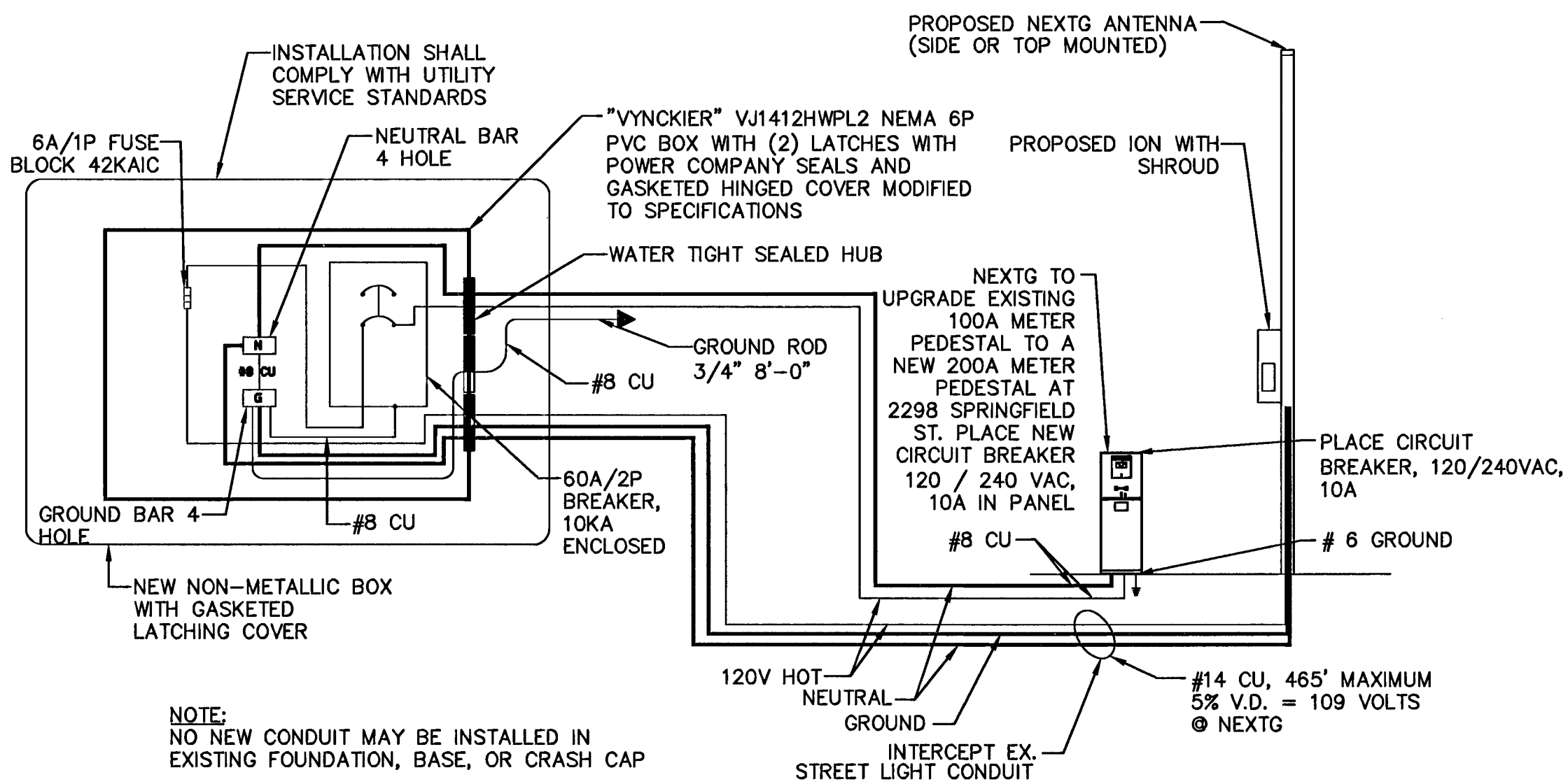
POWER SINGLE LINE DIAGRAM
