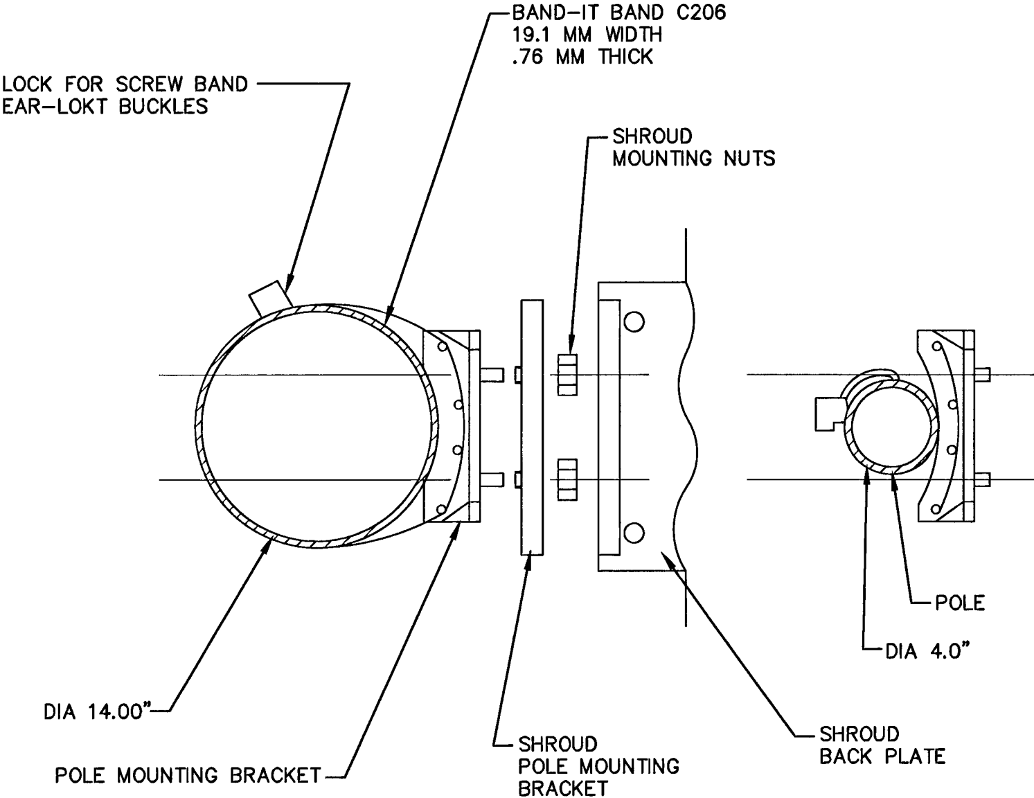
POLE MOUNTING NTS
