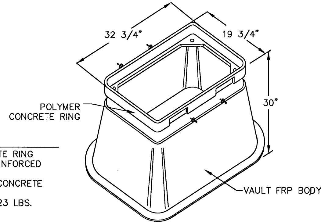
17' X 30' CONNECTOR MANHOLE NTS
