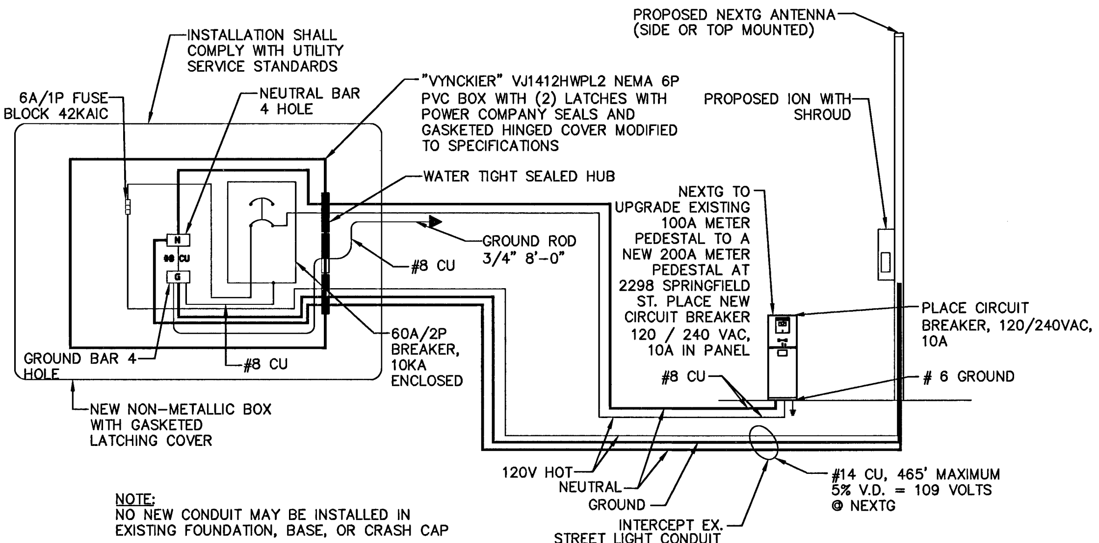
POWER SINGLE LINE DIAGRAM NTS
