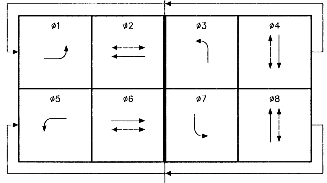
PHASE DIAGRAM CONFLICT FLASH SHALL BE ALL RED
