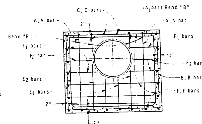
SECTION H-H
