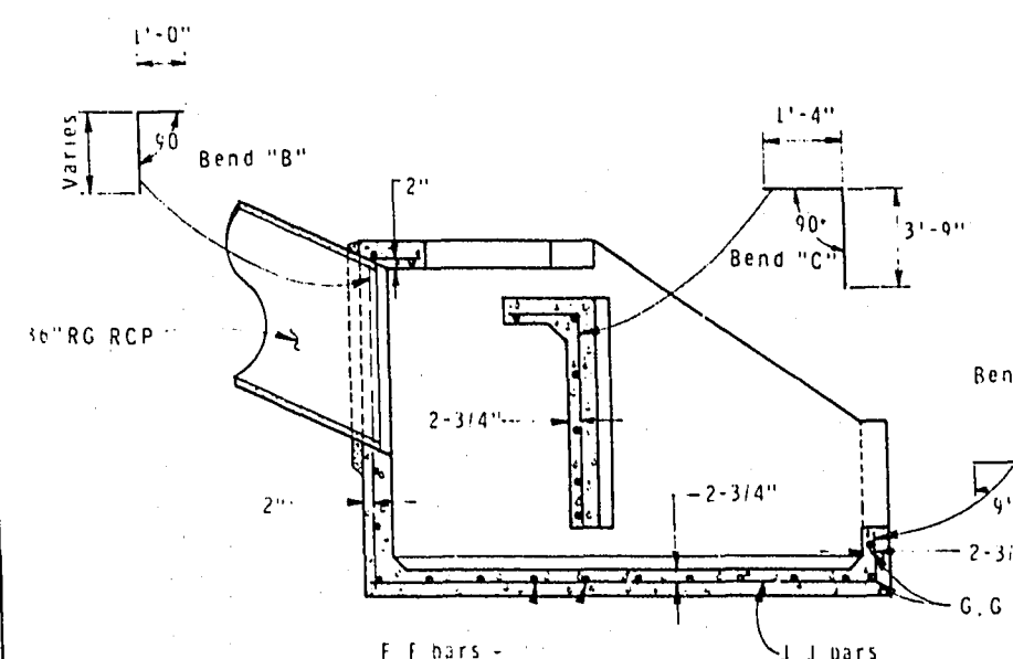
SECTION F-F
