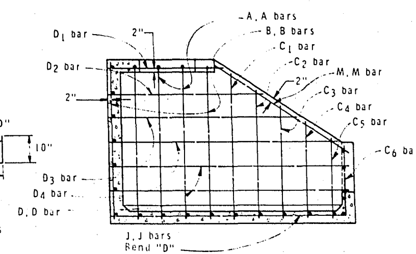
SECTION G-G
