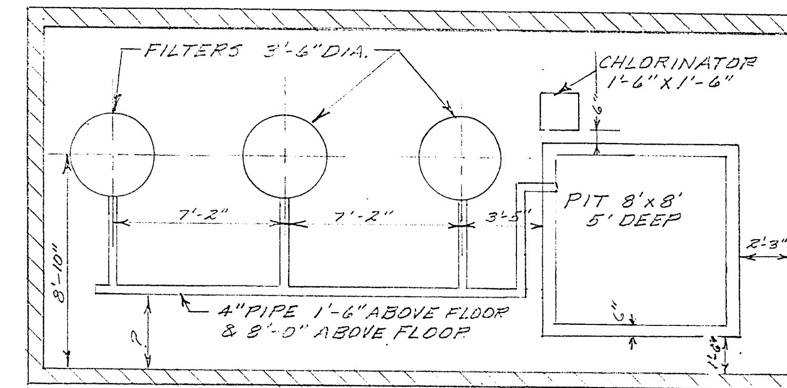
DETAIL OF FILTER ROOM SCALE: 1/4" = 1'-0"
