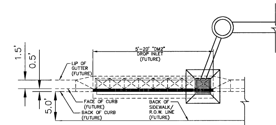
EXISTING UTILITY SUPPORT OVER RCB DETAIL
