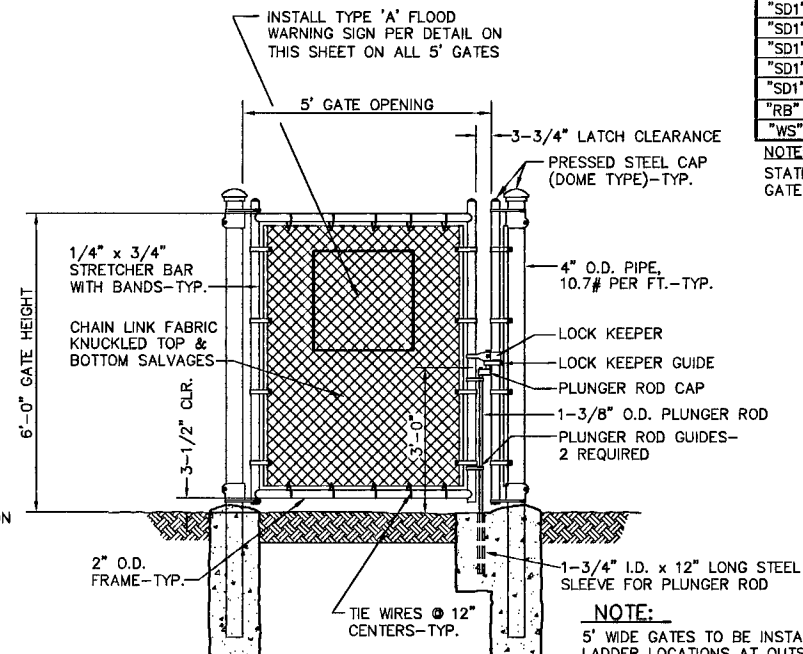
5' WIDE SINGLE-SWING GATE ELEVATION DETAIL
