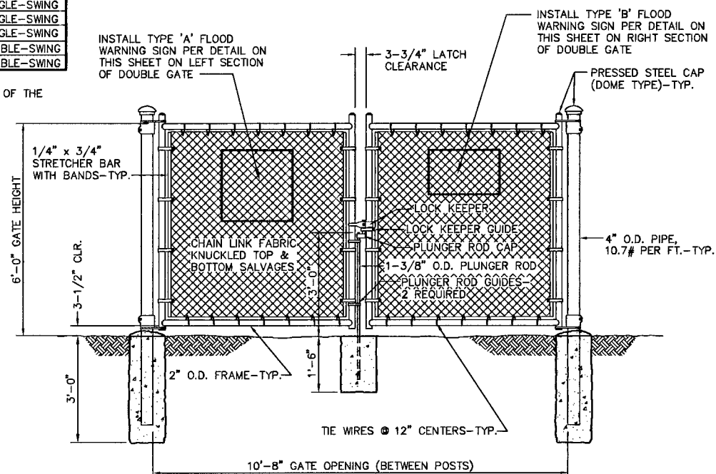
10'-8" DOUBLE SWING GATE DETAIL
