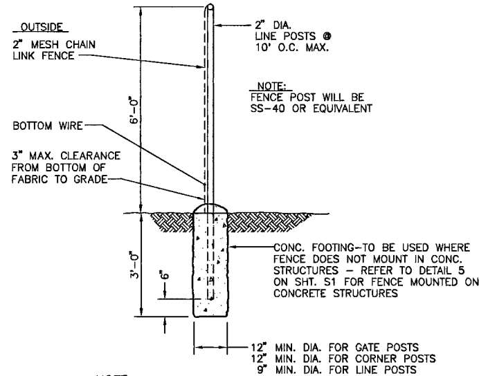
TYPICAL FENCE DETAIL N.T.S.
