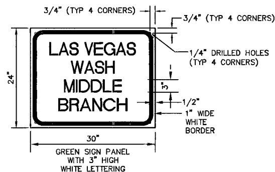
CHANNEL IDENTIFICATION SIGN DETAIL N.T.S.
