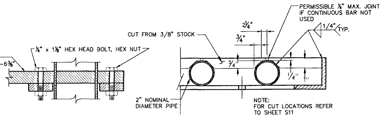
SECTION C-C
