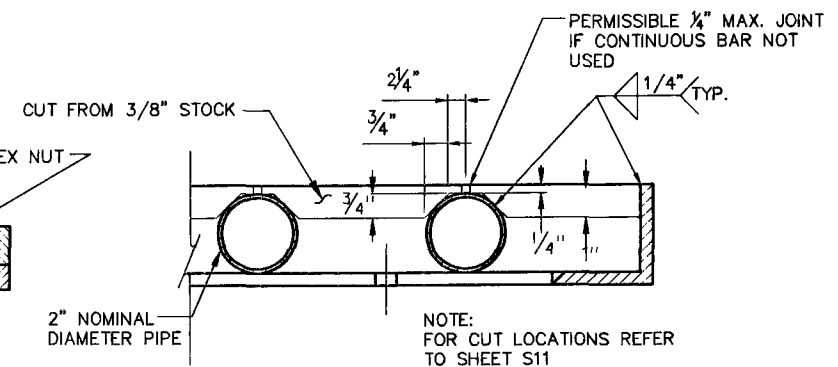
SECTION E-E
