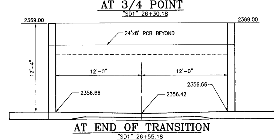
SECTIONS AT TRANSITION CHANNEL SCALE: 1/4"=1'-0"
