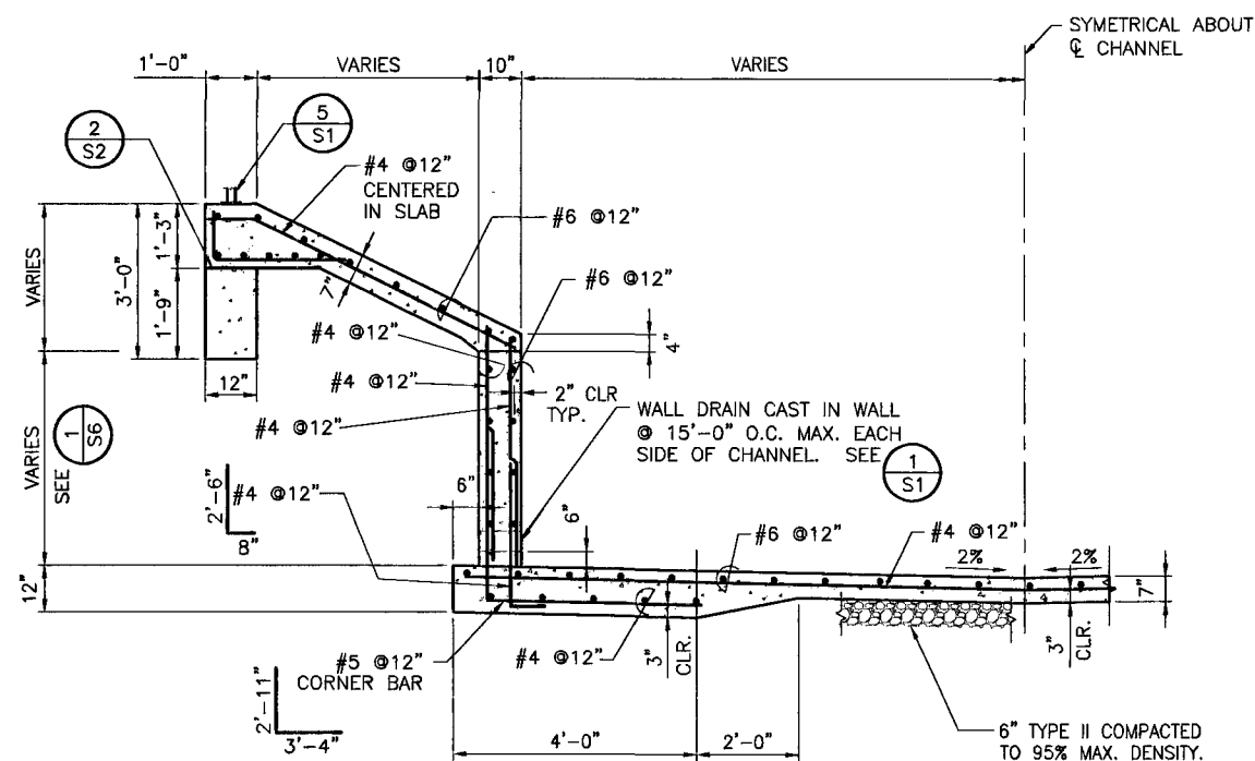
TRANSITION CHANNEL SECTION
