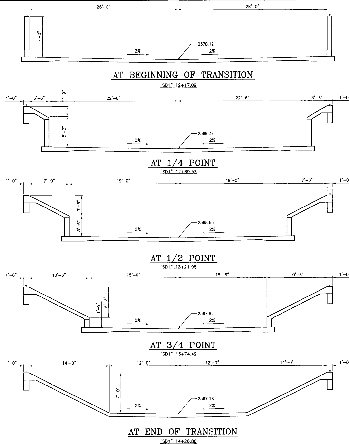
WALL SECTION AT TRANSITION CHANNEL
