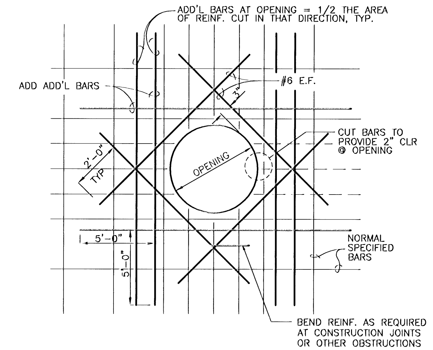
WALL OR SLAB OPENING DETAIL
