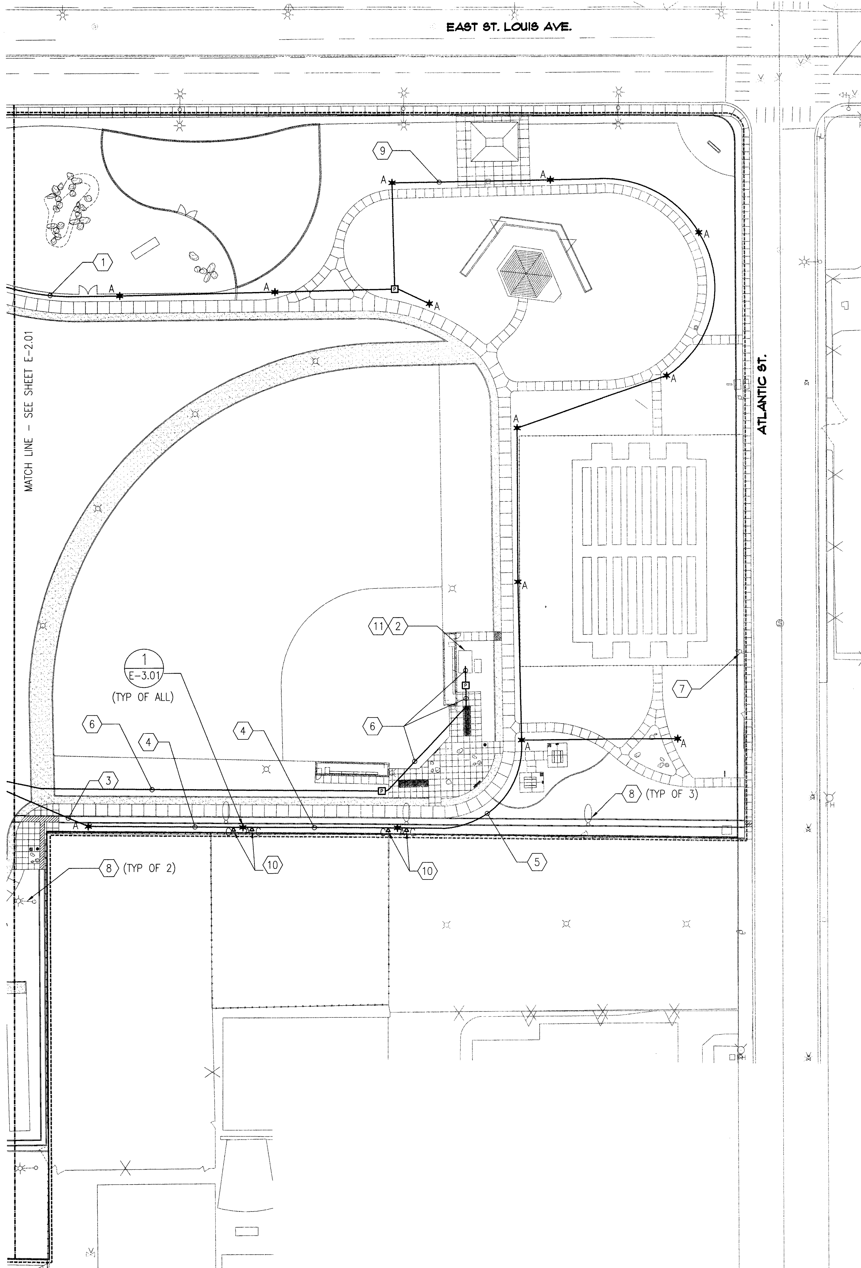
B PARTIAL ELECTRICAL SITE PLAN E-2.02 SCALE: 1"=40'-0" REFERENCE DRAWING E-2.02
