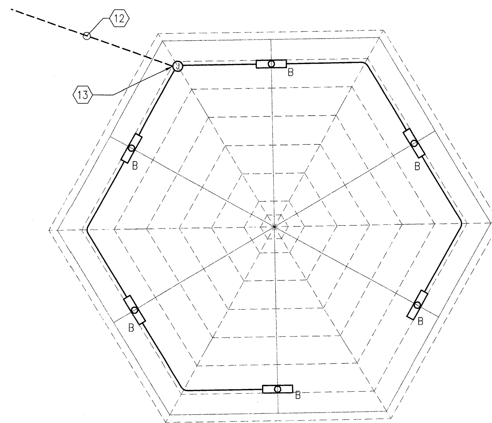
1 RAMADA ELECTRICAL PLAN E-2.02 SCALE: 1/8"=1'-0" REFERENCE DRAWING E-2.01
