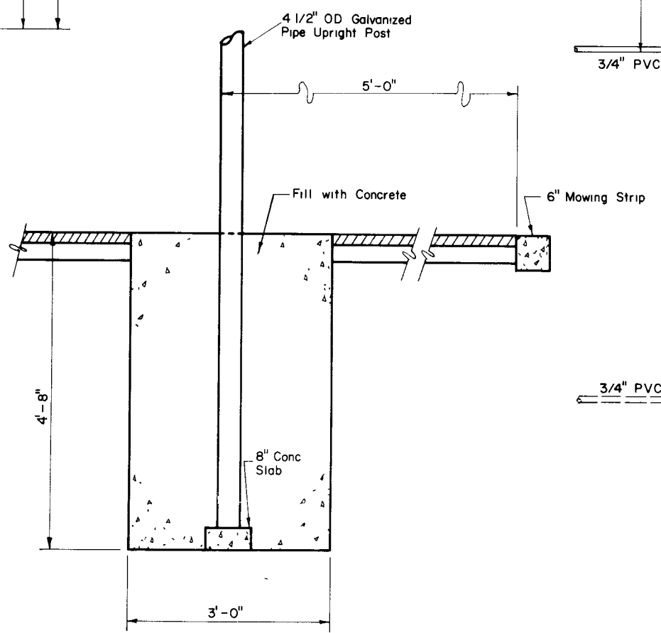
FOOTING FOR UPRIGHT POST
