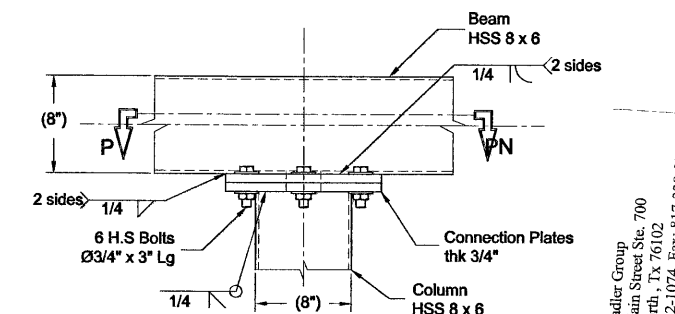
COLUMN - BEAM CONNECTION FRONT VIEW
