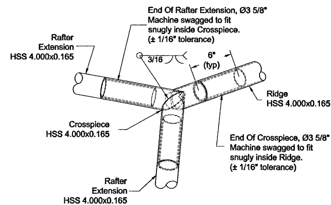
DETAIL L
