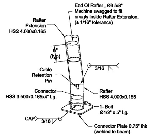
DETAIL M
