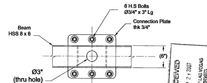
SECTION P-P
